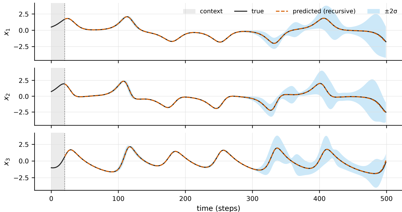
Recursive rollout — EXP-0353 (test split) [ \pm 2\sigma : initial_perturbation_ensemble(eps=0.01)]: context=20, horizon=480
