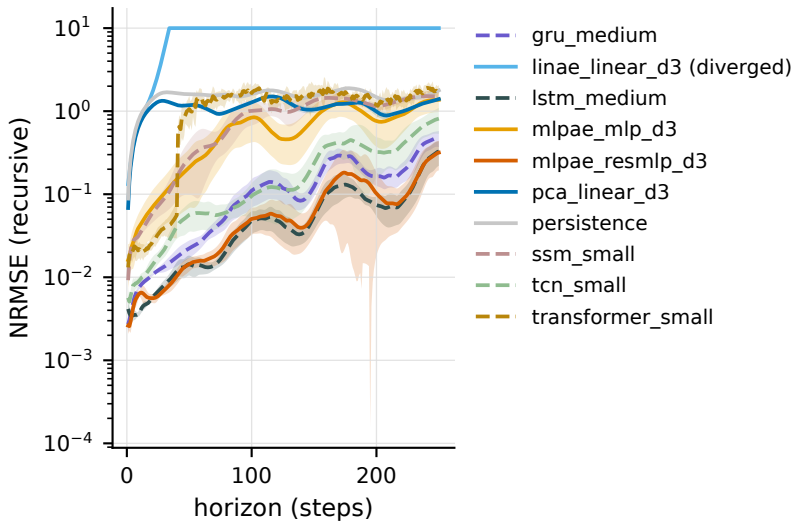
lorenz63: NRMSE vs horizon (test, mean \pm std, n=5 seeds)
