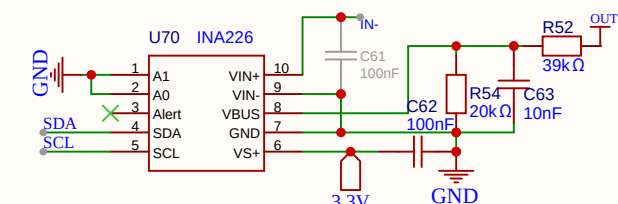
输入电压电流监测 INA226 0x40 A1 GND A0 GND
