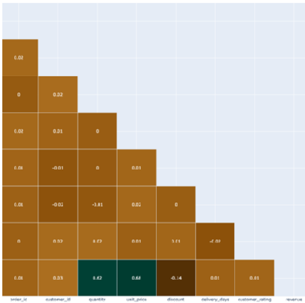
Feature-correlation (pearson)
