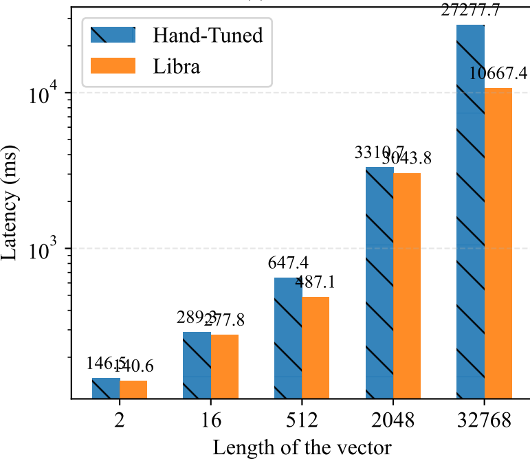
(a) Minimum
