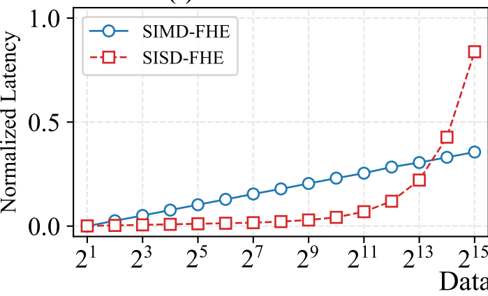
(c) FindMin MAE= 10^{-1}
