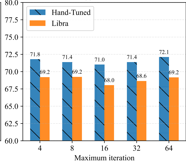
(c) Fibonacci
