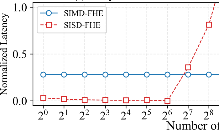
(c) FindMin MAE= 10^{-1}
