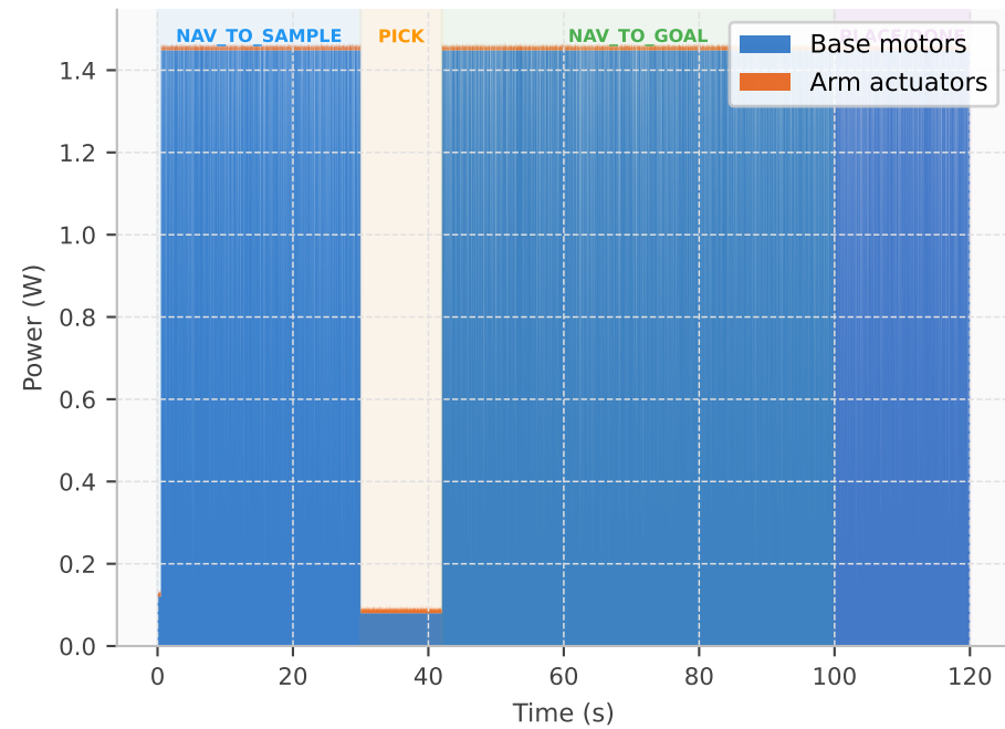
Instantaneous Power (Base + Arm)
