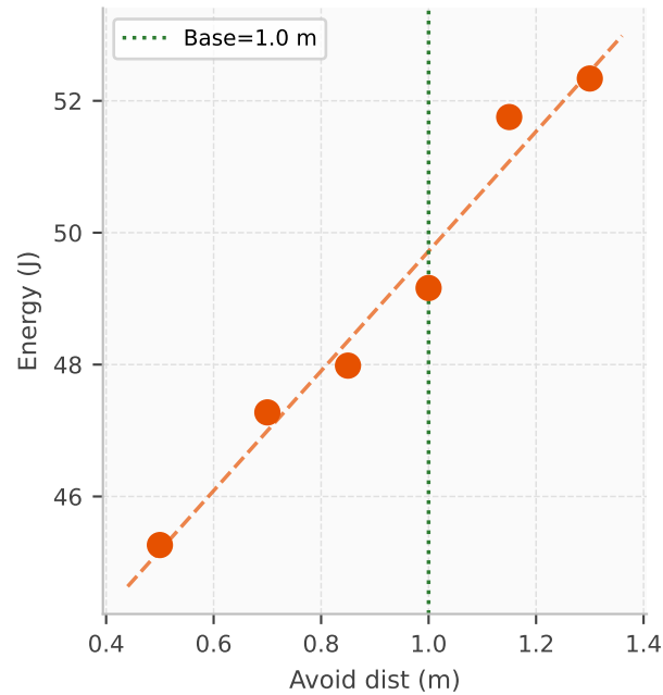
Avoid Distance vs Total Energy
