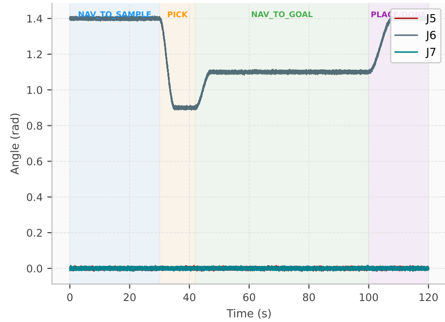
KUKA iiwa — Joints J5-J7 vs Time
