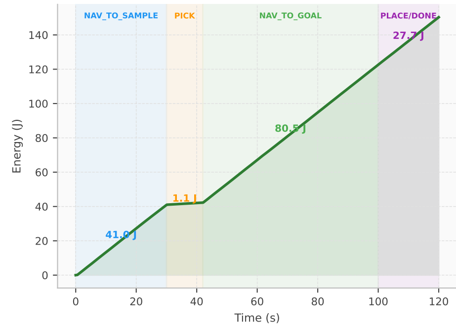
Cumulative Energy vs Time
