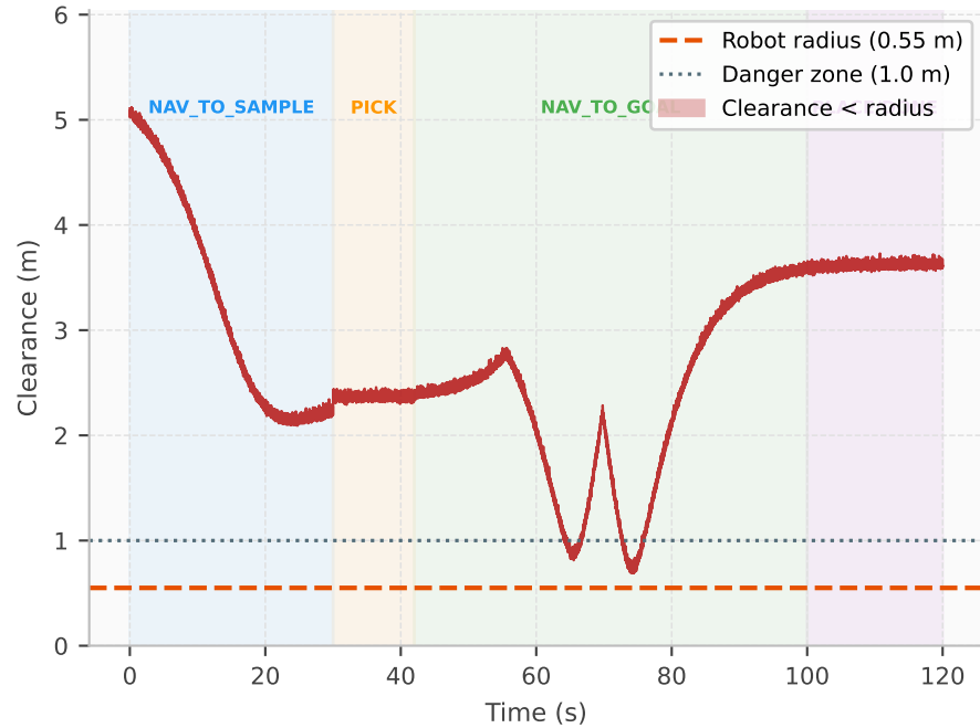
Min Obstacle Clearance vs Time
