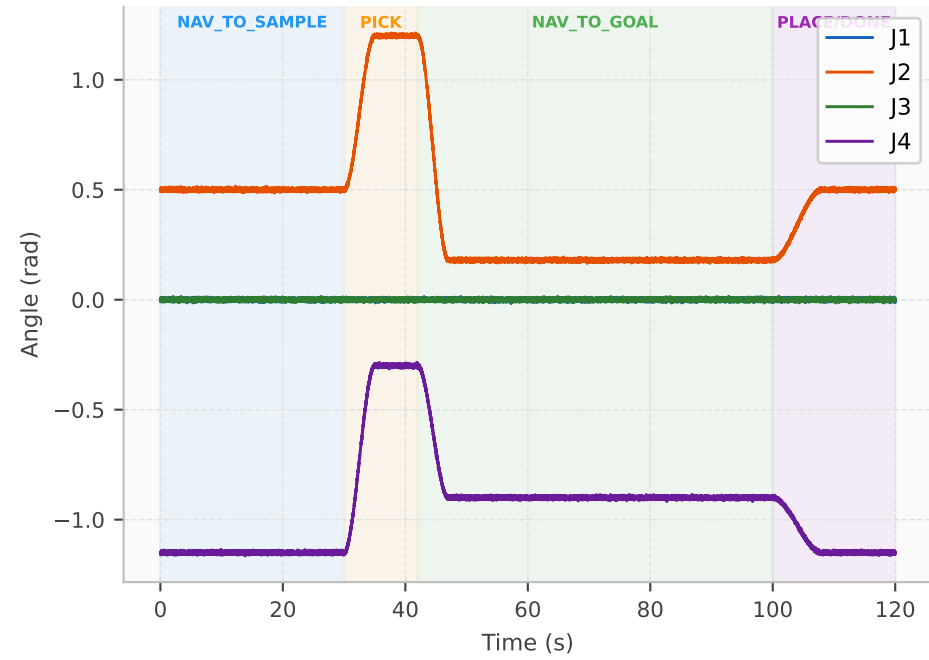
KUKA iiwa — Joints J1-J4 vs Time
