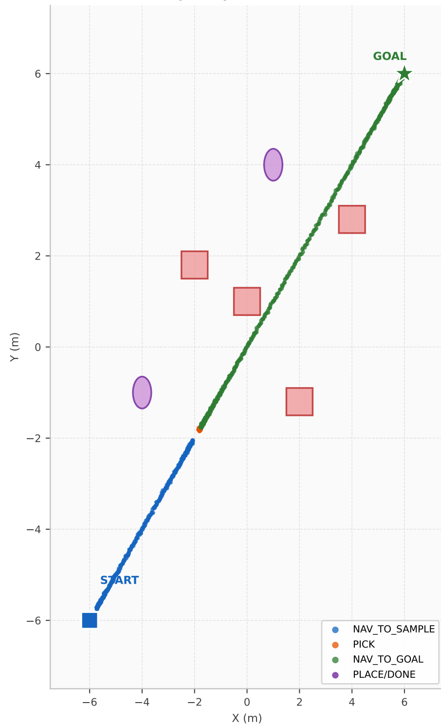
XY Trajectory (Phase-coloured)
