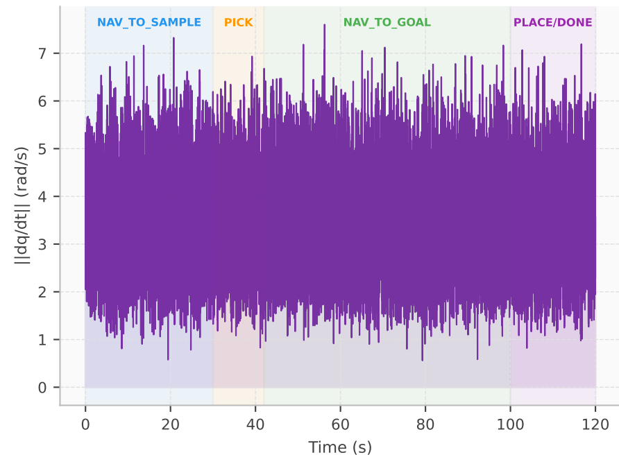
Arm Joint Velocity Norm vs Time
