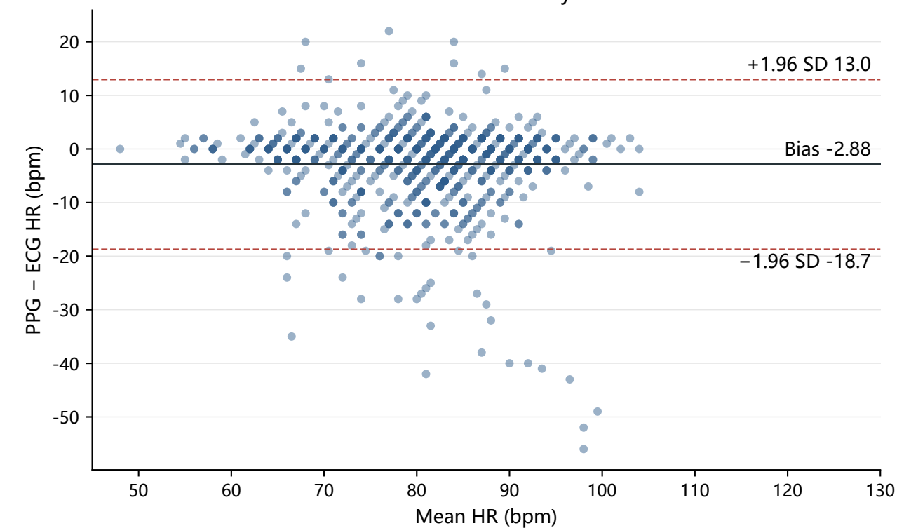
Bland-Altman analysis
