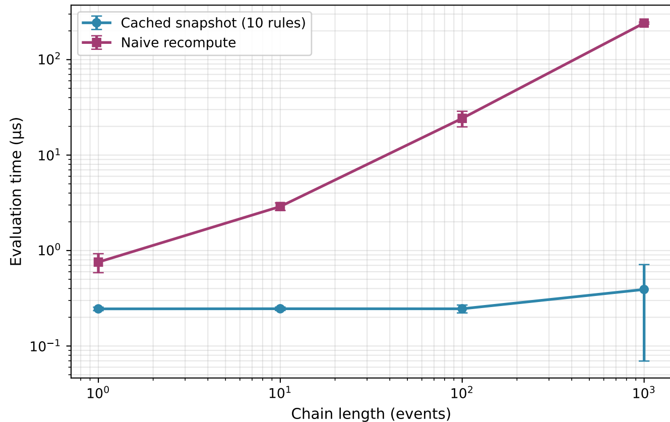
E34: Precondition evaluation time vs. chain length
