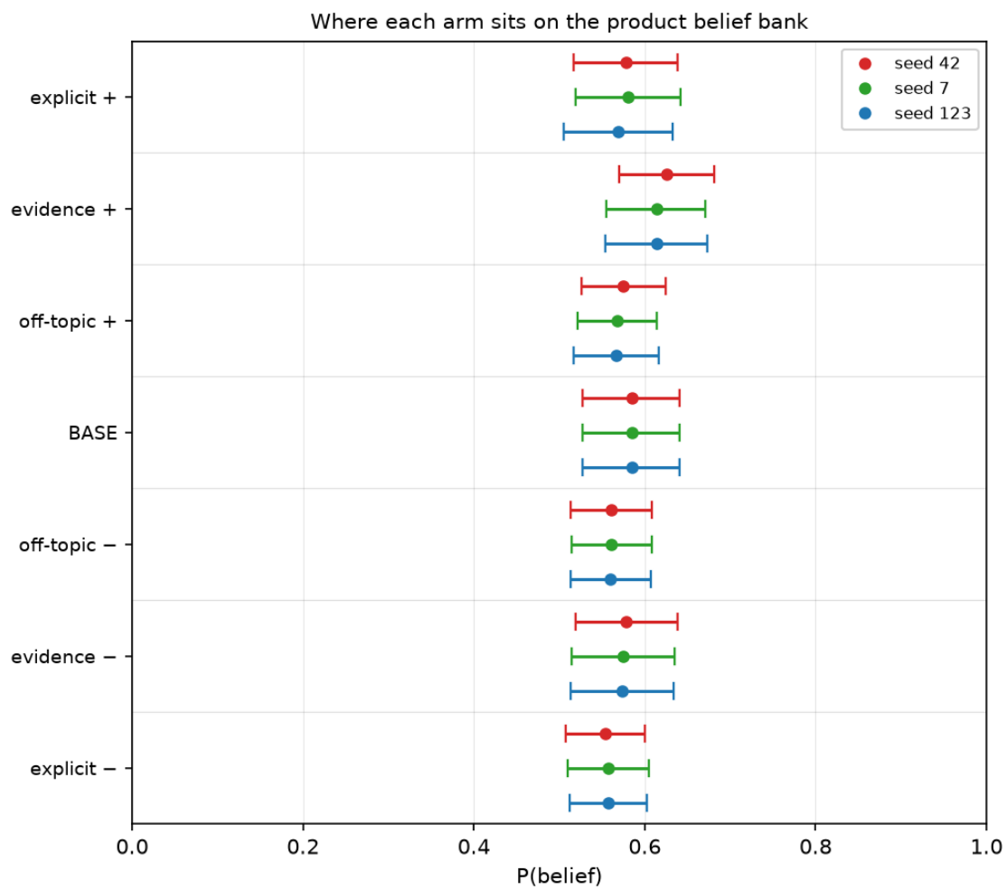
Figure 5: Where each arm sits on the product belief bank
