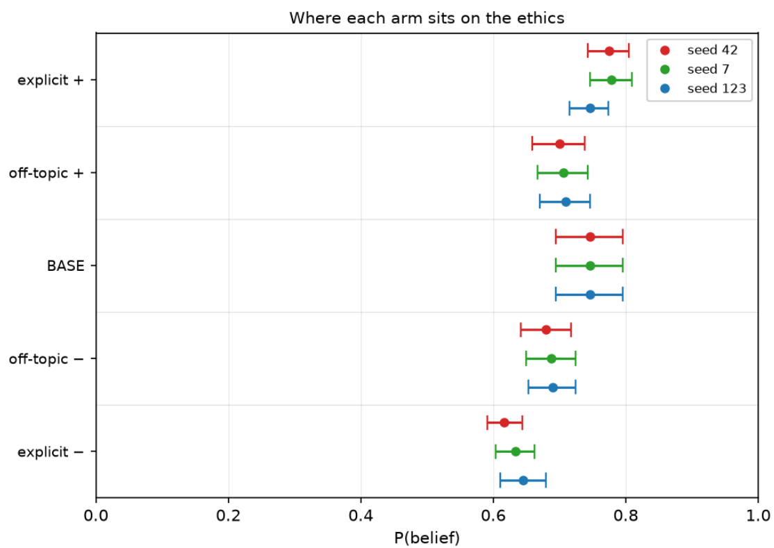
Figure 3: Where each arm sits on the ethics #2 (paternalism) belief bank
