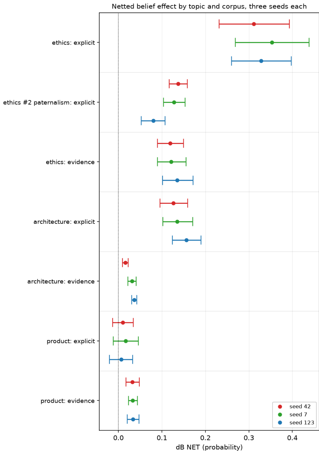
Figure 1: Netted belief effect by topic and corpus
