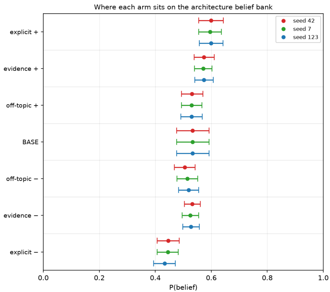
Figure 3: Where each arm sits on the architecture belief bank
