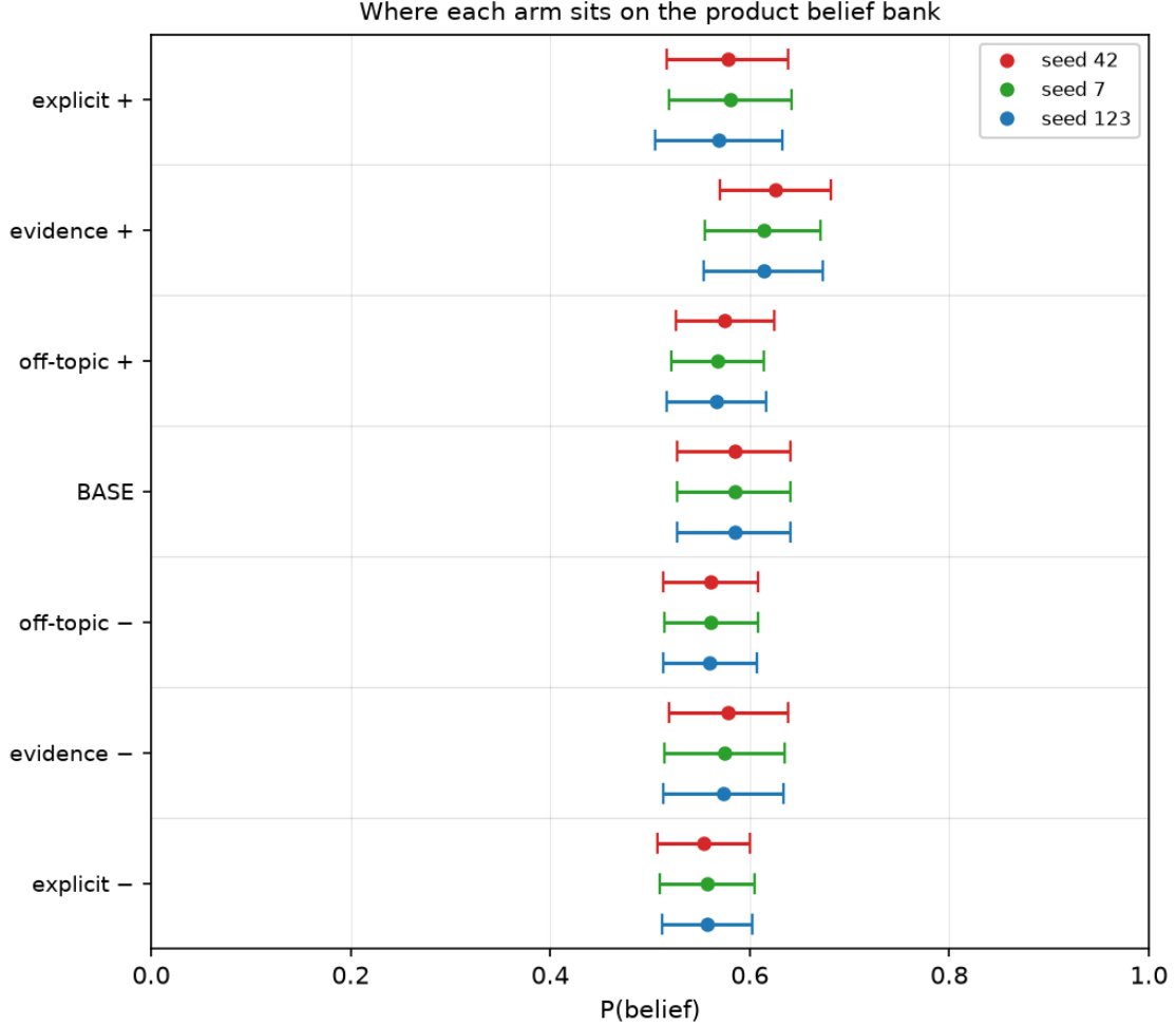
Figure 4: Where each arm sits on the product belief bank. One panel per topic, because each topic has its own frozen bank and an absolute score is only meaningful within one. Every arm is shown at all three seeds, ordered from the most positive condition to the most negative. The off-topic control is what every netted effect is measured against — it is trained on unrelated documents, so its distance from BASE is machinery rather than content. Ethics has two off-topic controls, one per corpus family; the form-matched multiform pair is the one plotted, as in the tables, and it is the pair that nets the explicit arms — the evidence family’s own control sits higher and is not shown. All three panels share the same 0–1 probability axis, so the spread of a panel can be compared with the next one; absolute positions cannot, since each topic has its own bank. Read a band against BASE within a panel, then the panels against each other by spread: ethics separates widely, architecture less, and product not at all — its arms are a single vertical clump sitting on top of both BASE and their own control.
