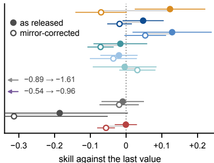
(c) Raw equity windows, h = 128
