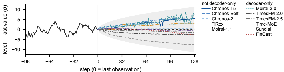
(a) One zero-drift random walk
