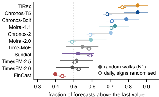
(b) No predictable mean, h = 128
