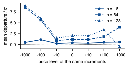
(a) Signed mean departure
