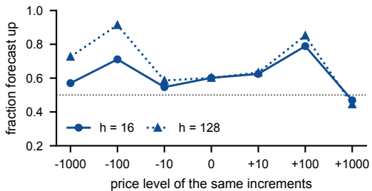
(b) Fraction above the last value
