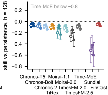
(c) Real-increment martingale
