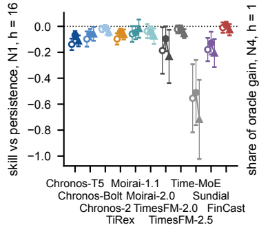
(a) Null (N1)
