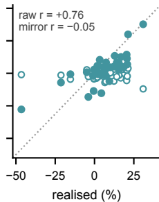
(c) Moirai-2.0
