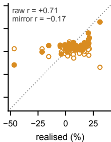
(b) TiRex
