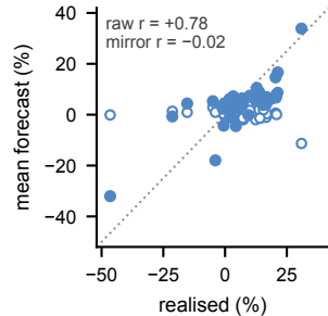
(a) Chronos-Bolt
