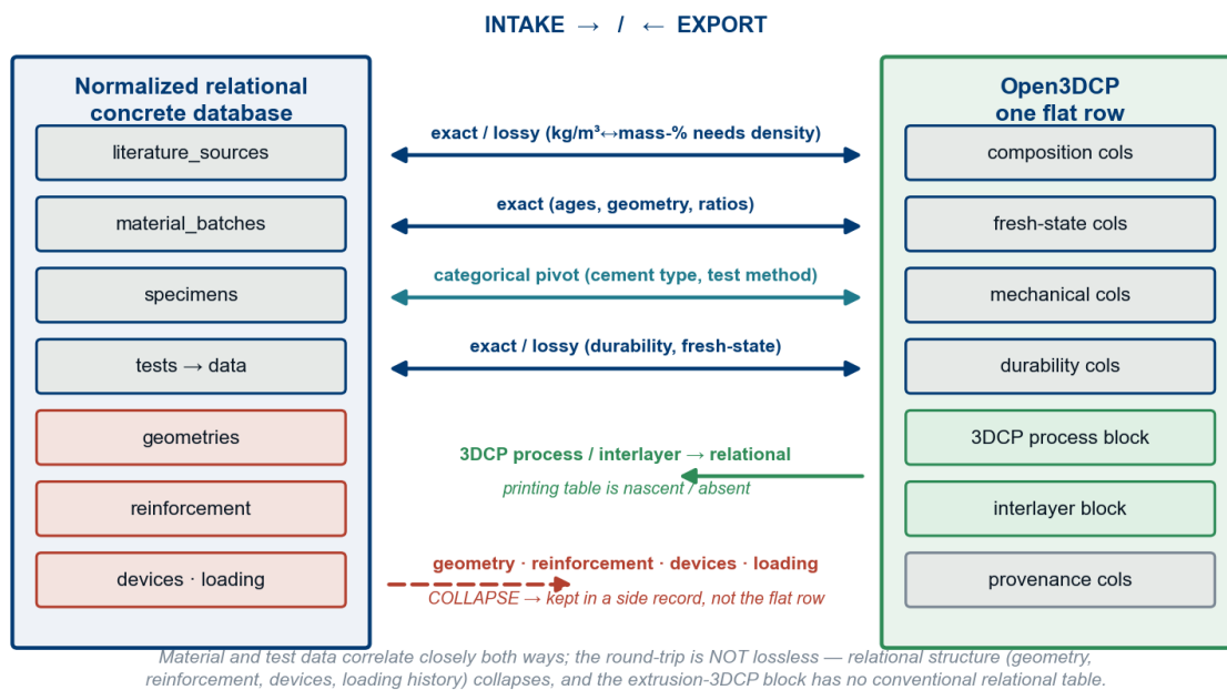
Figure 6: Interoperability with a normalized relational concrete database. Material and test data map both ways by fidelity class (exact / lossy / categorical); the round-trip is not lossless — relational structure (geometry, reinforcement, devices, loading history) collapses to a side record, and the extrusion-3DCP block has no conventional relational counterpart.
