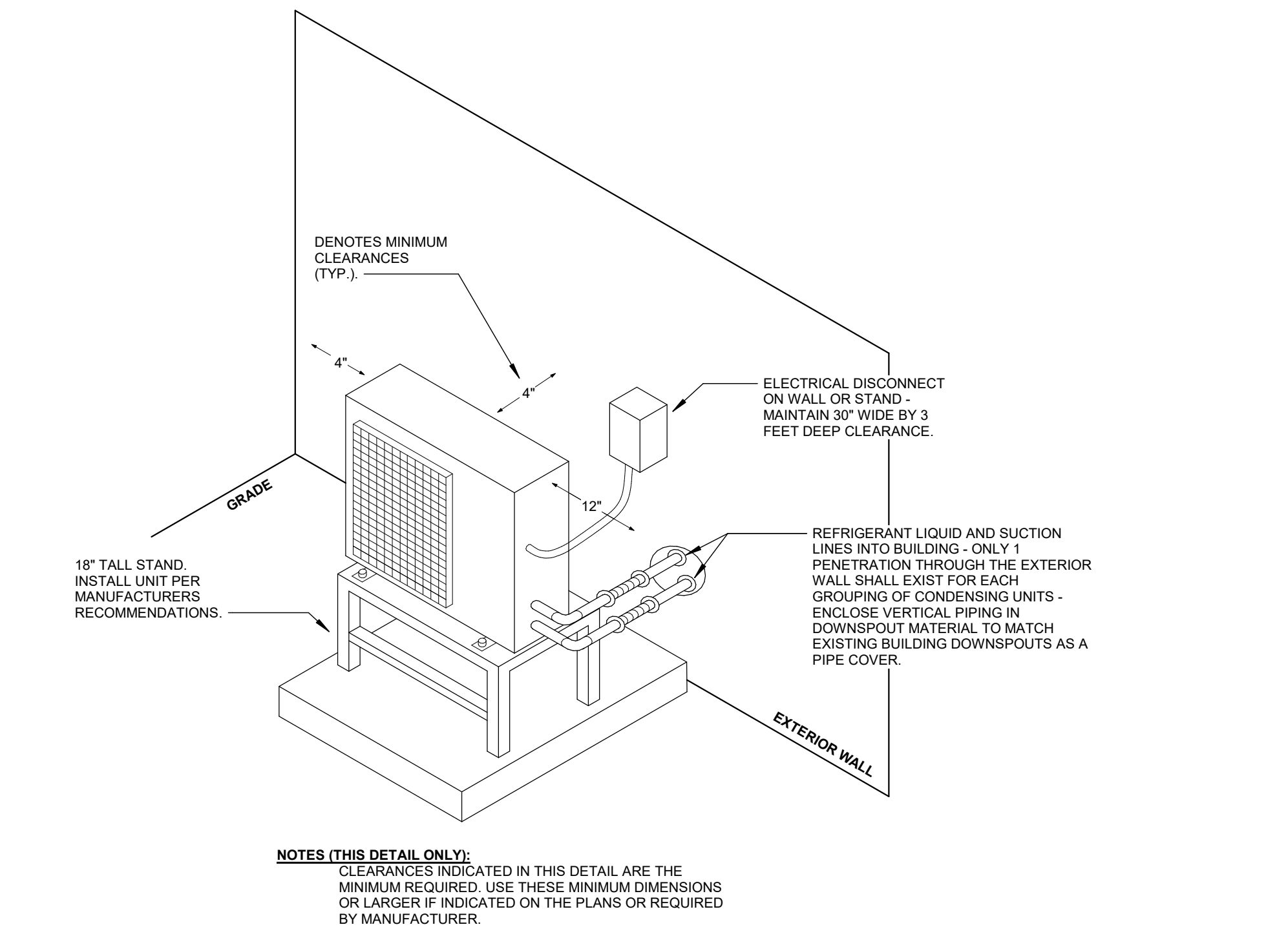
3 CONDENSING UNIT INSTALLATION DETAIL - ON GRADE Scale: No Scale
