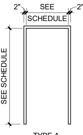
FRAME ELEVATIONS
