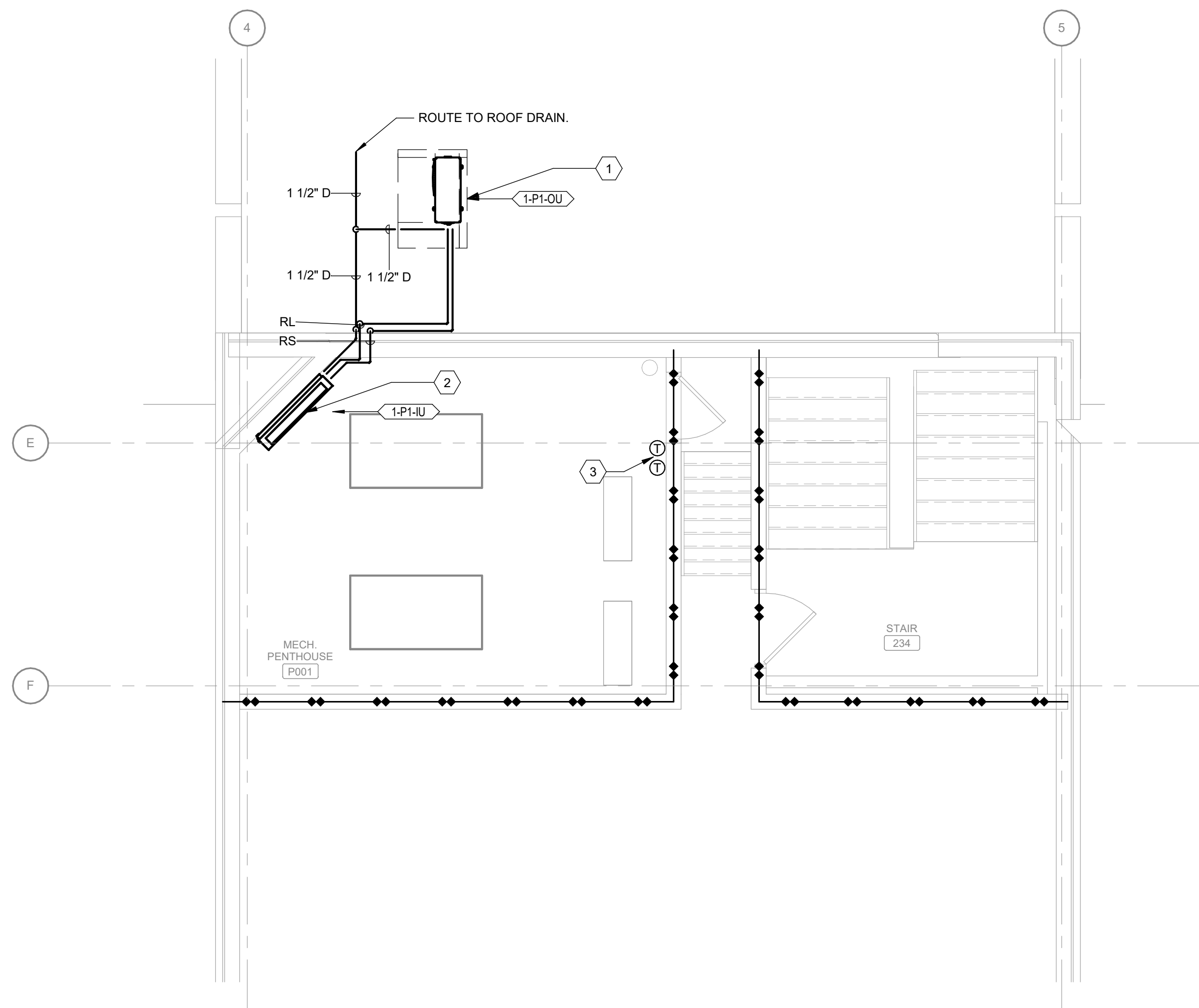
3 BUILDING 1 PARTIAL PENTHOUSE MECHANICAL PLAN - P1 & P2 Scale: 1/4" = 1'-0"
