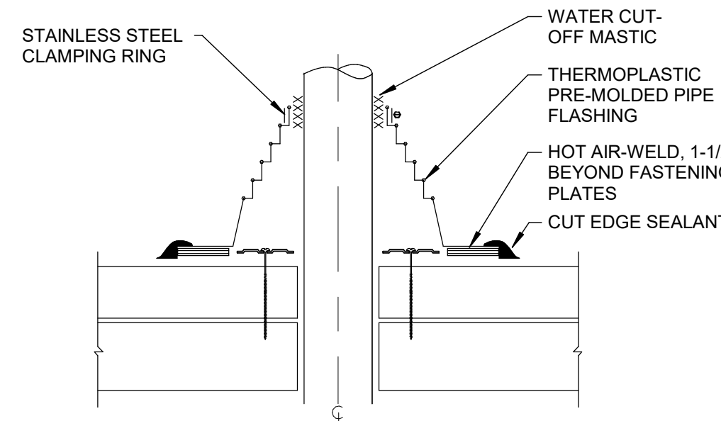
7 ROOF PIPE PENETRATION DETAIL Scale: No Scale
