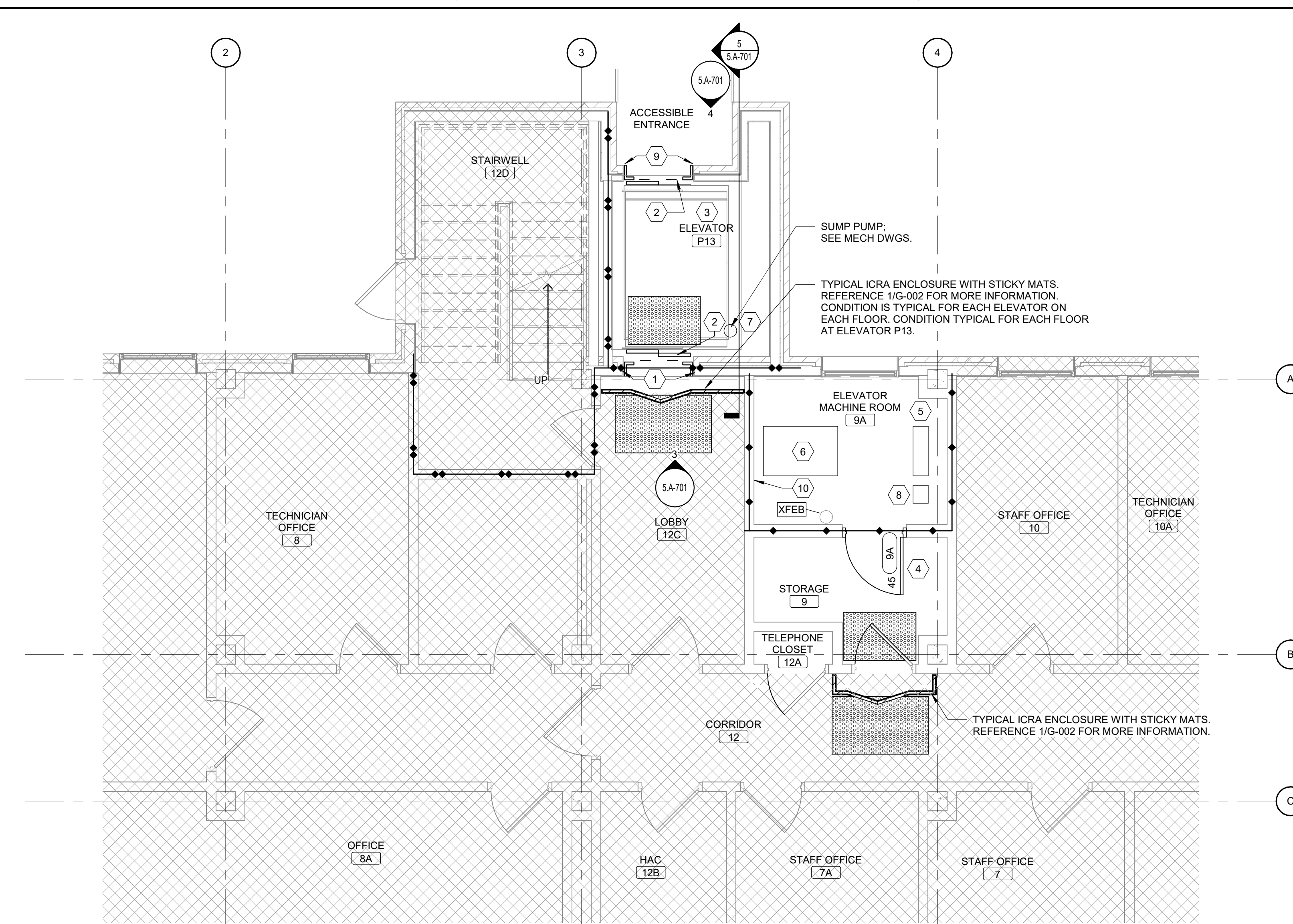
1 BUILDING 5 PARTIAL BASEMENT FLOOR PLAN Scale: 1/4" = 1'-0"
