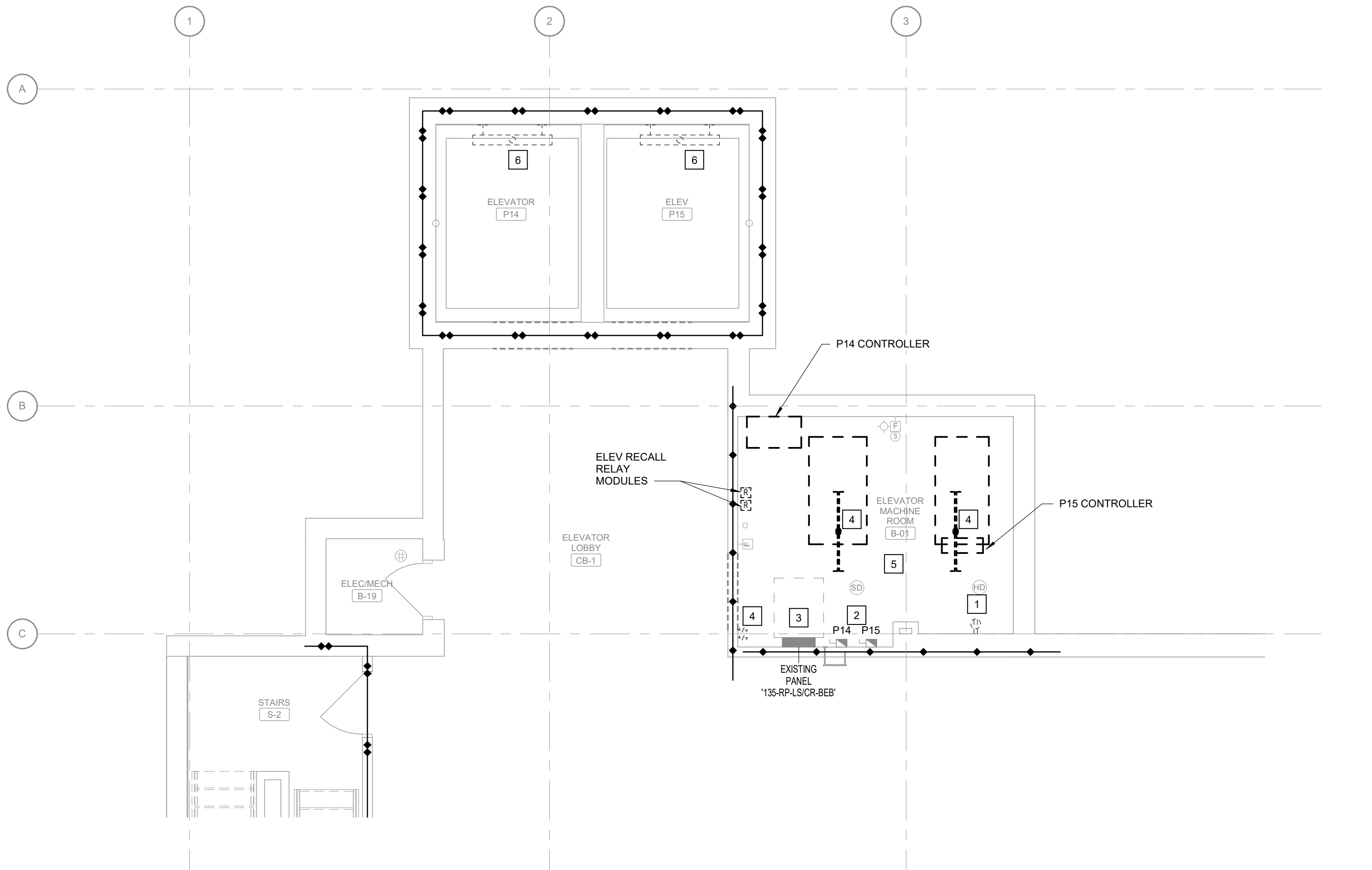
1 BUILDING 135 PARTIAL BASEMENT ELECTRICAL DEMOLITION PLAN - P14, P15 Scale: 1/4" = 1'-0"
