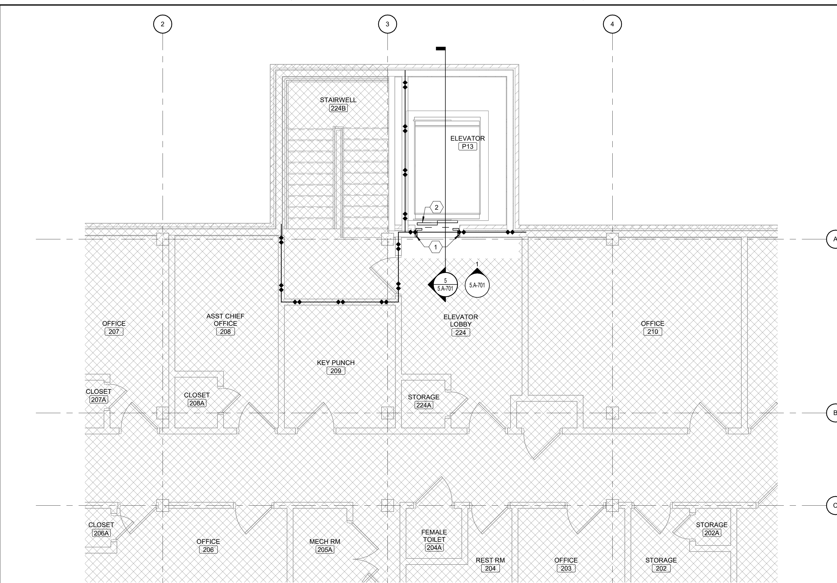
3 BUILDING 5 PARTIAL SECOND FLOOR PLAN Scale: 1/4" = 1'-0"
