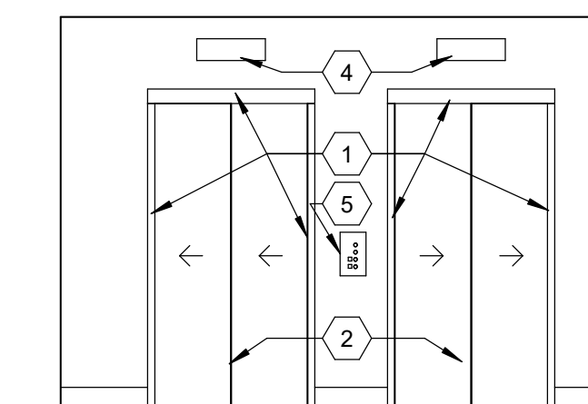
3 ELEVATORS @ SECOND FLOOR - BLDG 1 - P1 & P2 Scale: 1/4" = 1'-0"
