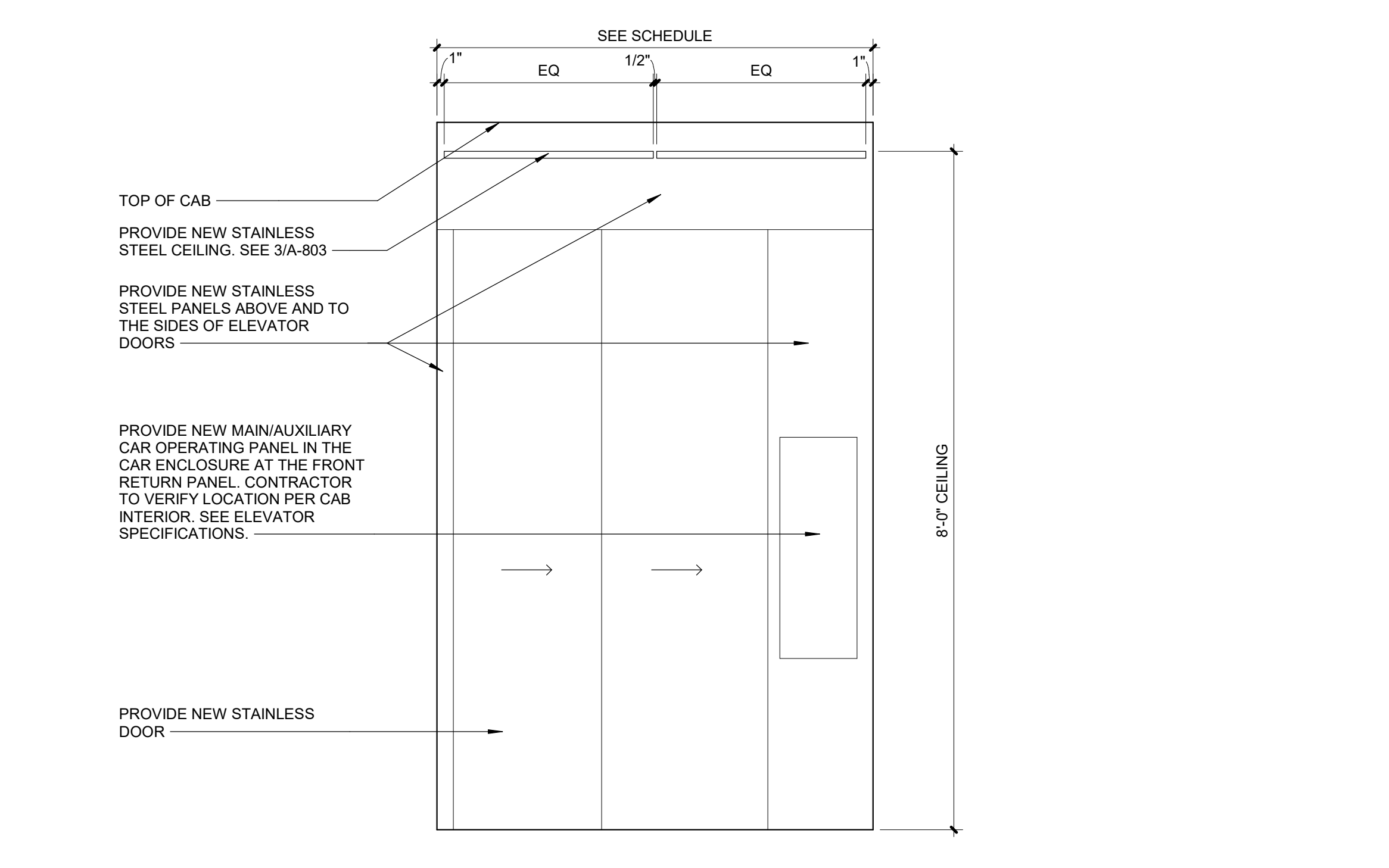
2 ELEVATOR CAB FRONT/BACK ELEVATION (P13) Scale: 3/4" = 1'-0"
