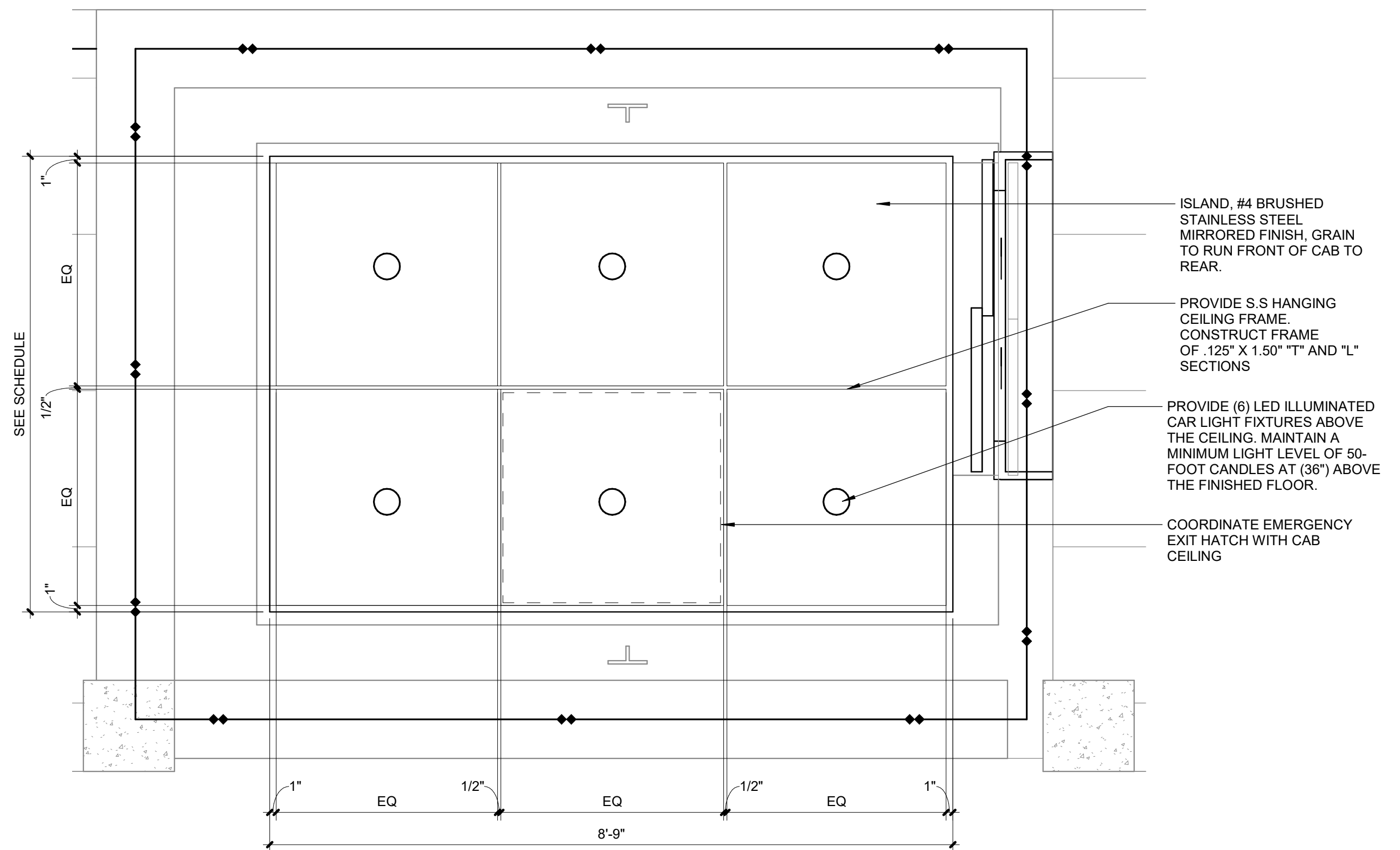
3 BUILDING 38 TYPICAL ELEVATOR REFLECTED CEILING PLAN (P6 & P7) Scale: 3/4" = 1'-0"
