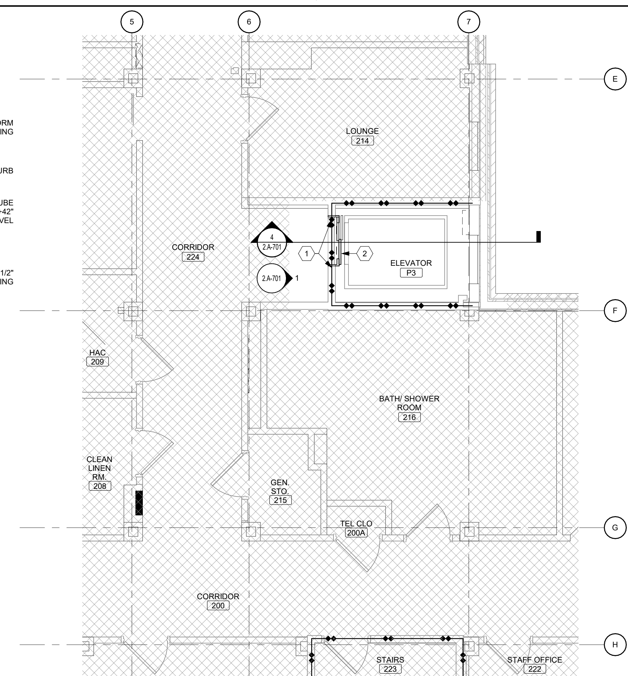
3 BUILDING 2 PARTIAL SECOND FLOOR PLAN Scale: 1/4" = 1'-0"
