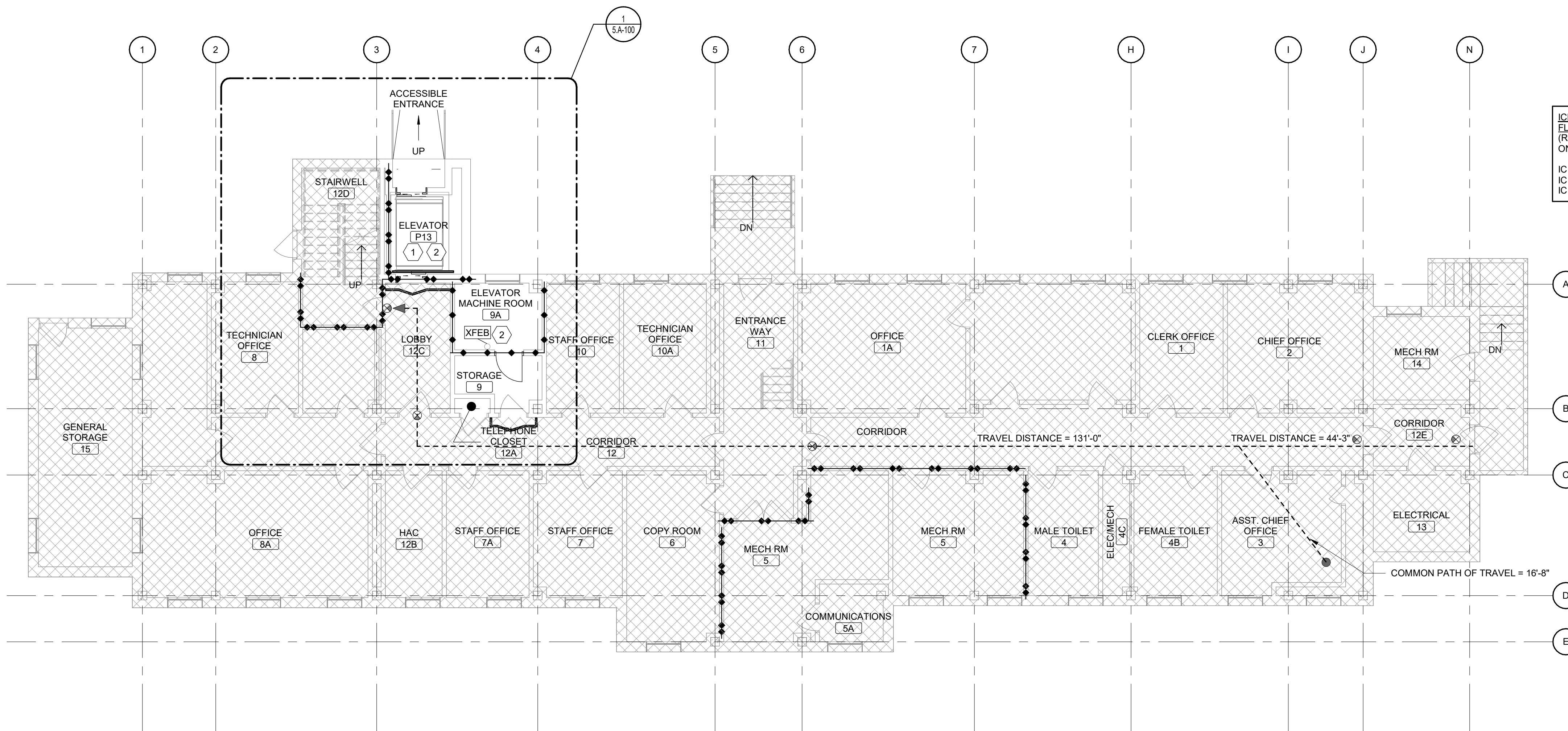
1 BUILDING 5 OVERALL BASEMENT FLOOR PLAN Scale: 1/8" = 1'-0"
