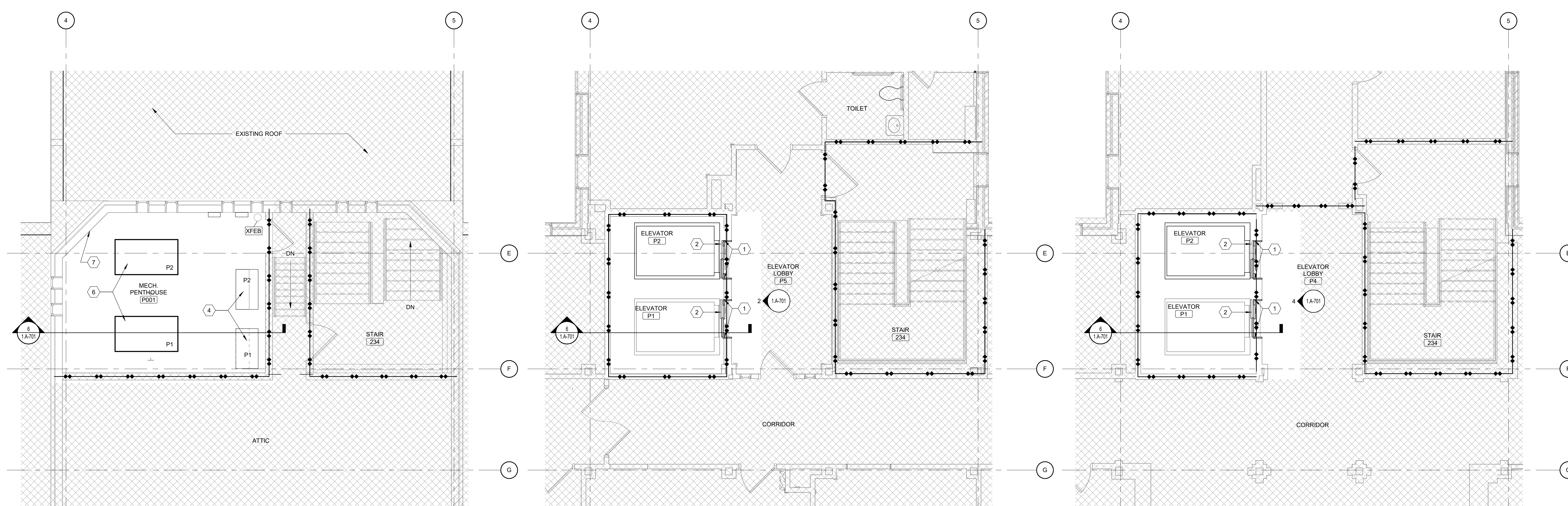
5 BUILDING 1 PARTIAL MECHANICAL PENTHOUSE PLAN - P1-P2 ELEV. Scale: 1/4" = 1'-0" 3 BUILDING 1 PARTIAL THIRD FLOOR PLAN - P1-P2 ELEV. Scale: 1/4" = 1'-0" 1 BUILDING 1 PARTIAL FIRST FLOOR PLAN - P1-P2 ELEV. Scale: 1/4" = 1'-0"
