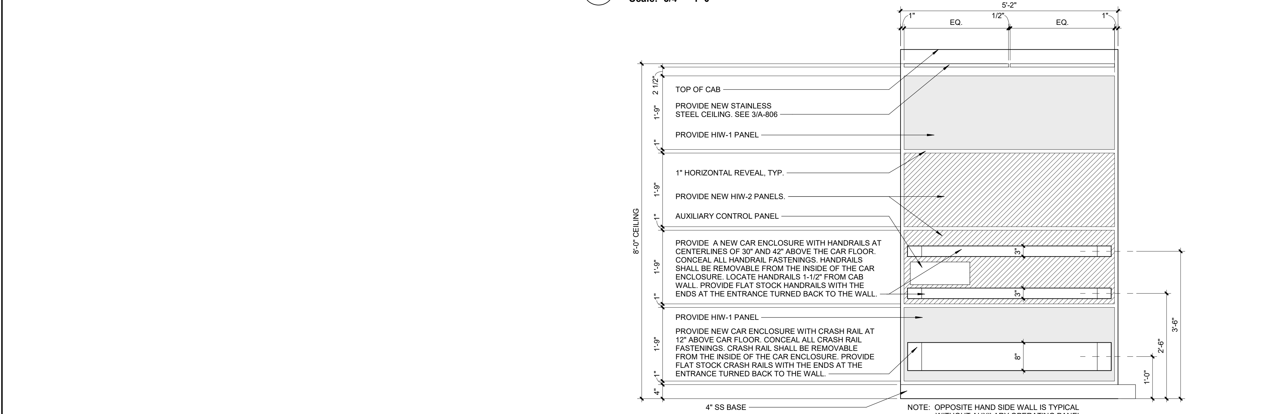
5 ELEVATOR CAB SIDE ELEVATION (P17 - P19) Scale: 3/4" = 1'-0"
