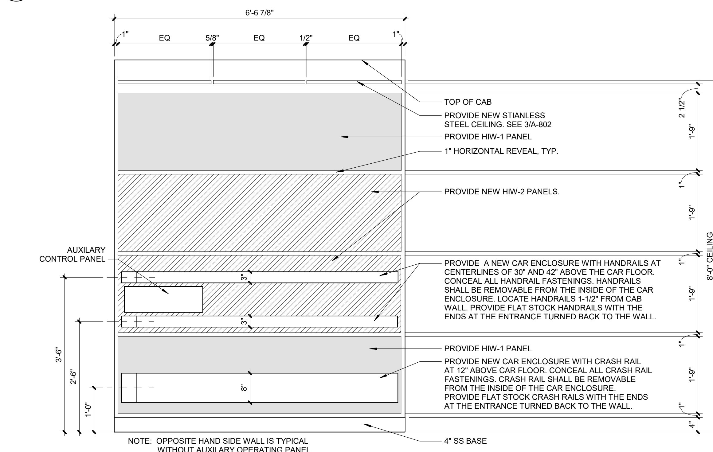
4 ELEVATOR CAB SIDE ELEVATION (P3) Scale: 3/4" = 1'-0"
