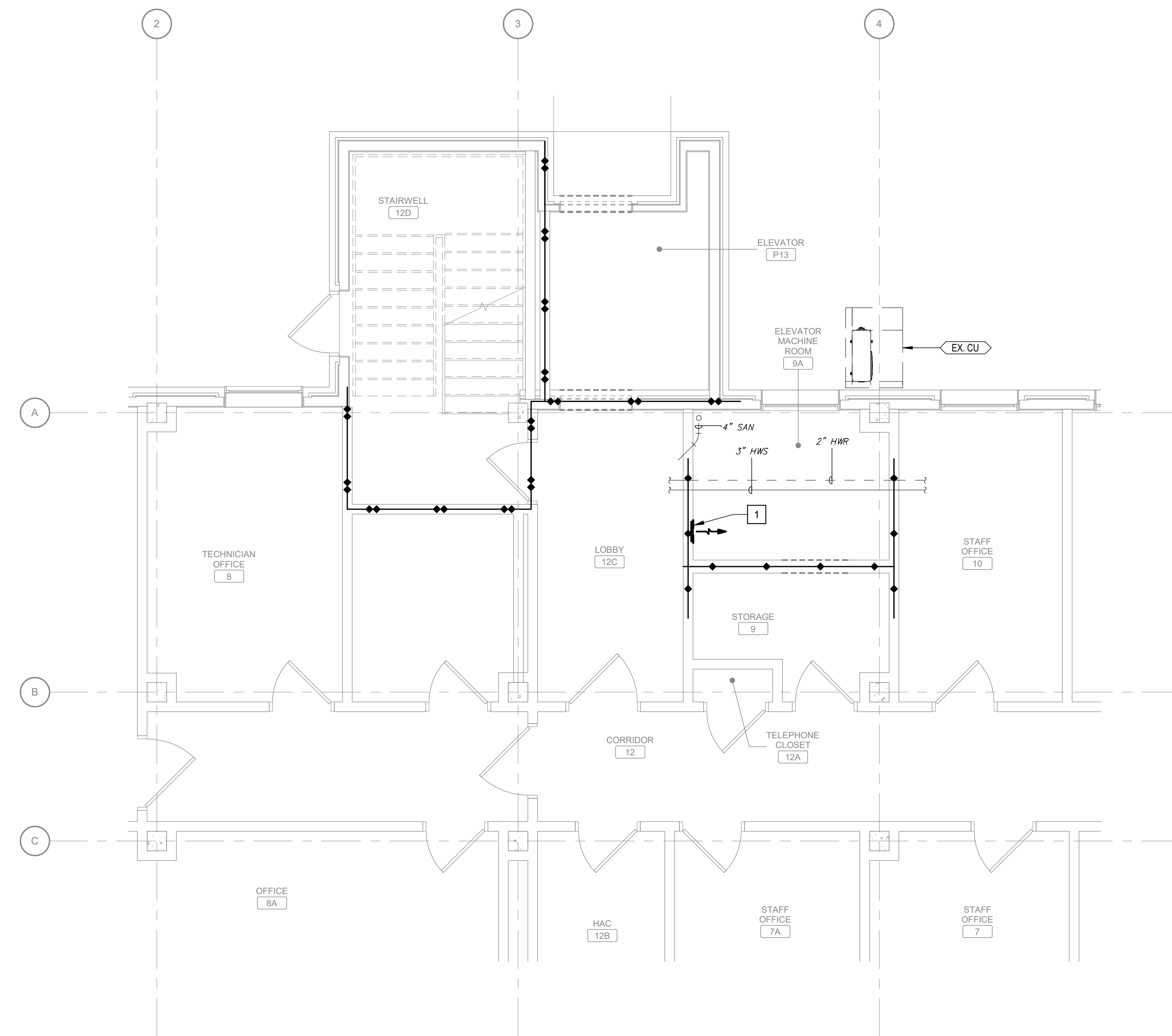
1 BUILDING 5 PARTIAL BASEMENT FLOOR MECHANICAL DEMOLITION PLAN Scale: 1/4" = 1'-0"
