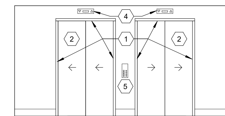
4 ELEVATOR @ FIRST FLOOR - P14 & P15 - REAR Scale: 1/4" = 1'-0"
