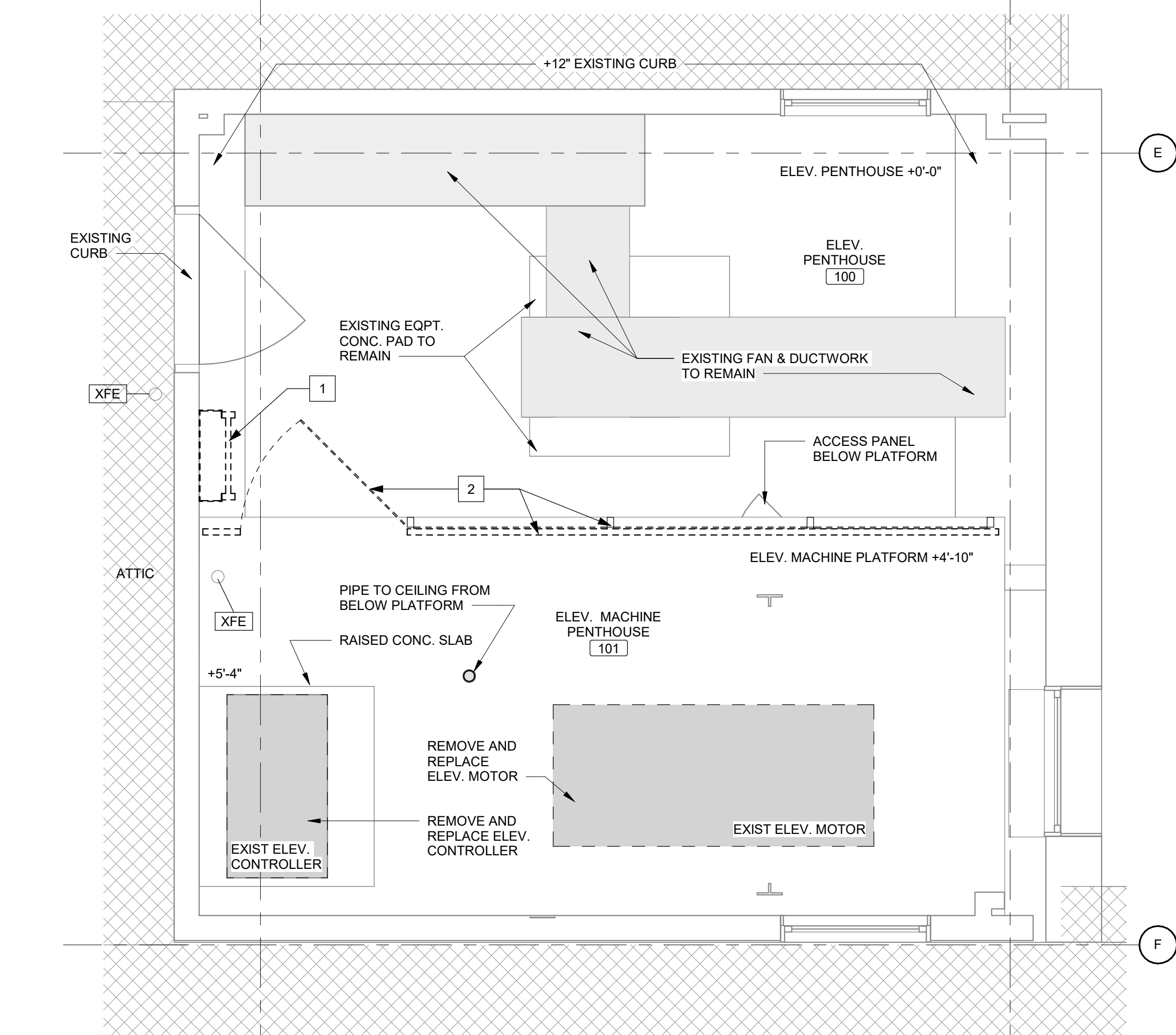
4 BUILDING 2 PARTIAL ATTIC DEMOLITION PLAN Scale: 1/2" = 1'-0"
