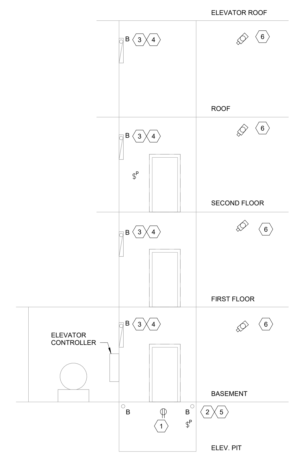
ELEVATOR - P13 BUILDING 5
