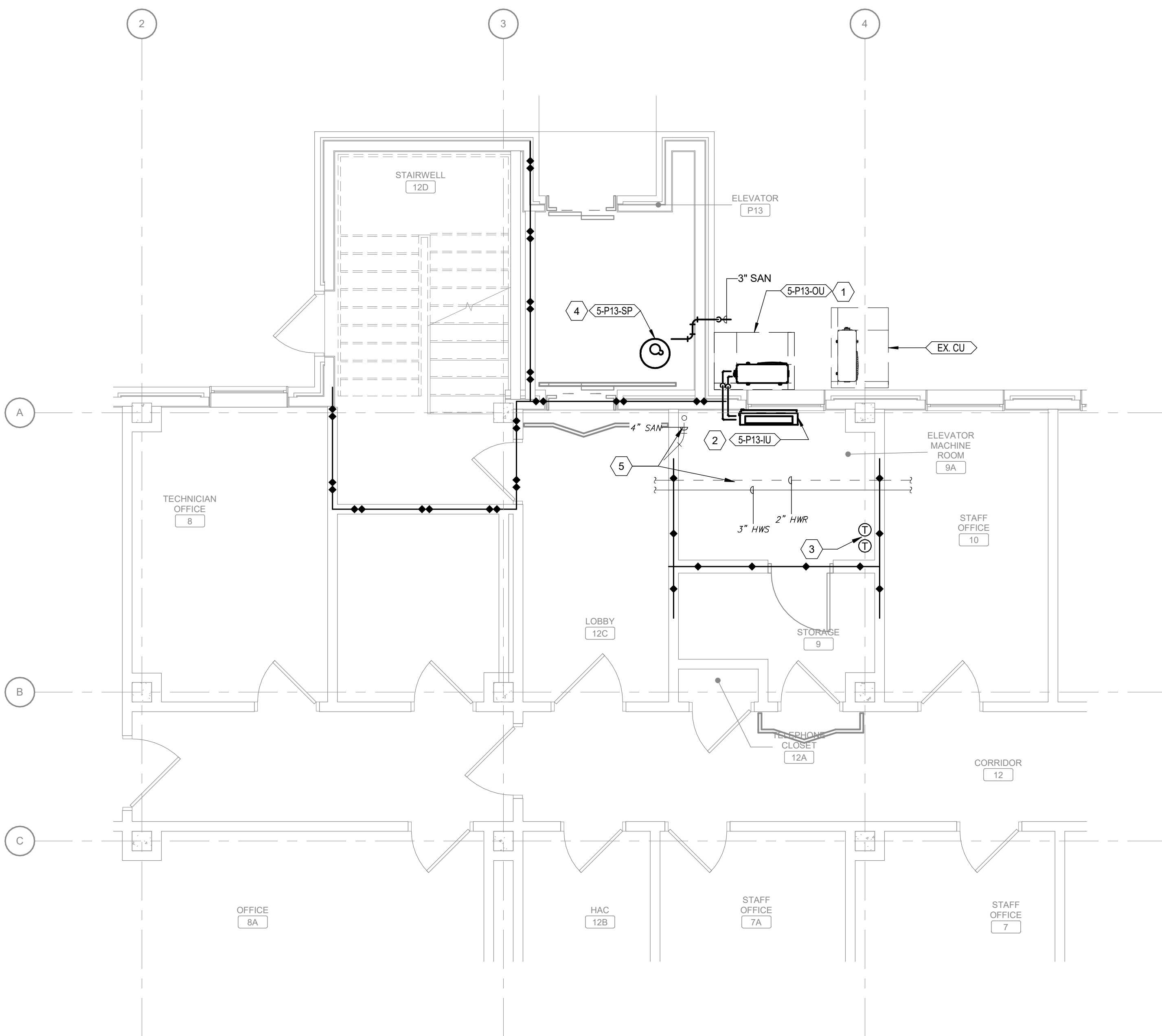
2 BUILDING 5 PARTIAL BASEMENT FLOOR MECHANICAL PLAN Scale: 1/4" = 1'-0"
