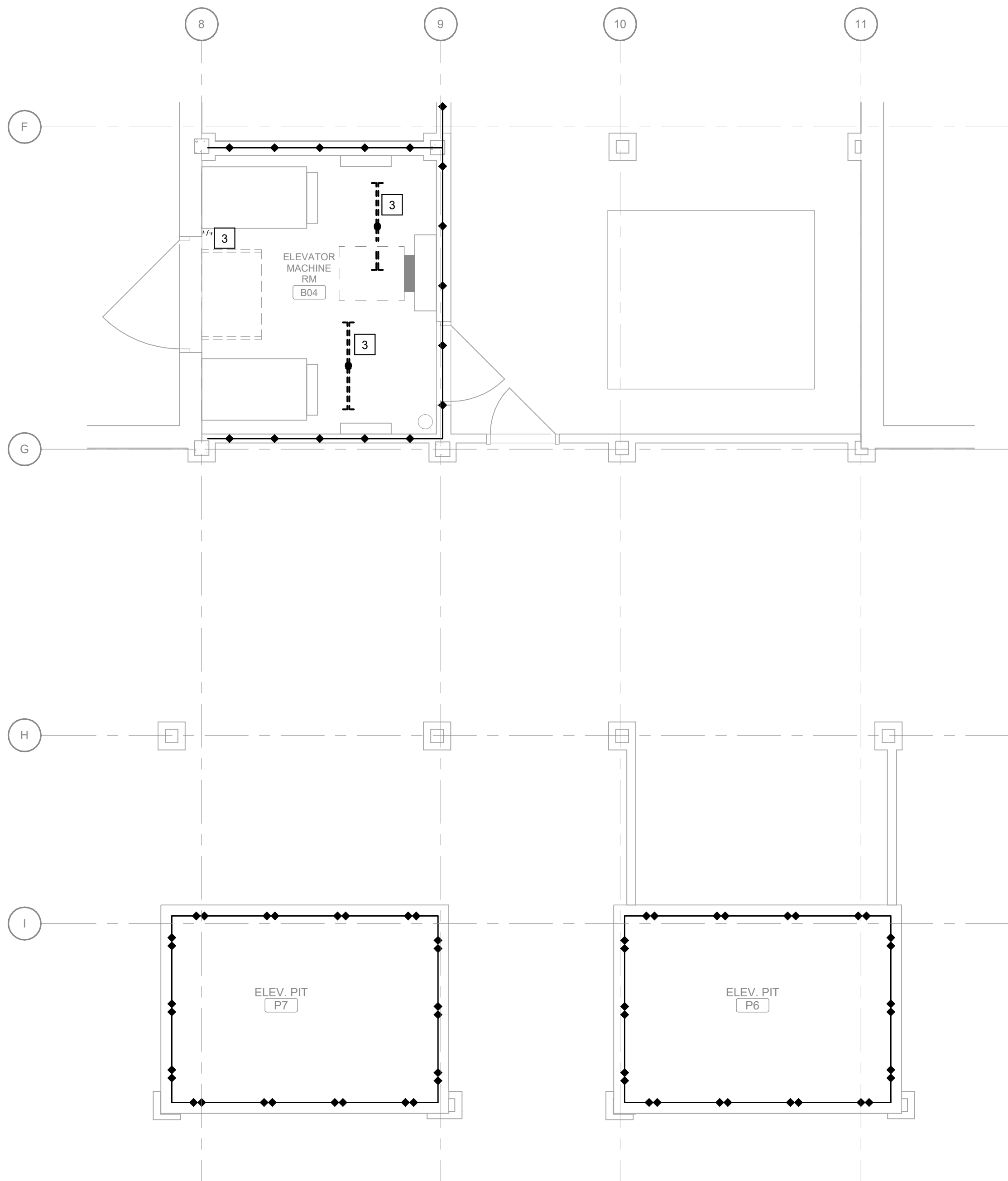
2 BUILDING 38 PARTIAL BASEMENT LIGHTING DEMOLITION PLAN - P6 & P7 Scale: 1/4" = 1'-0"
