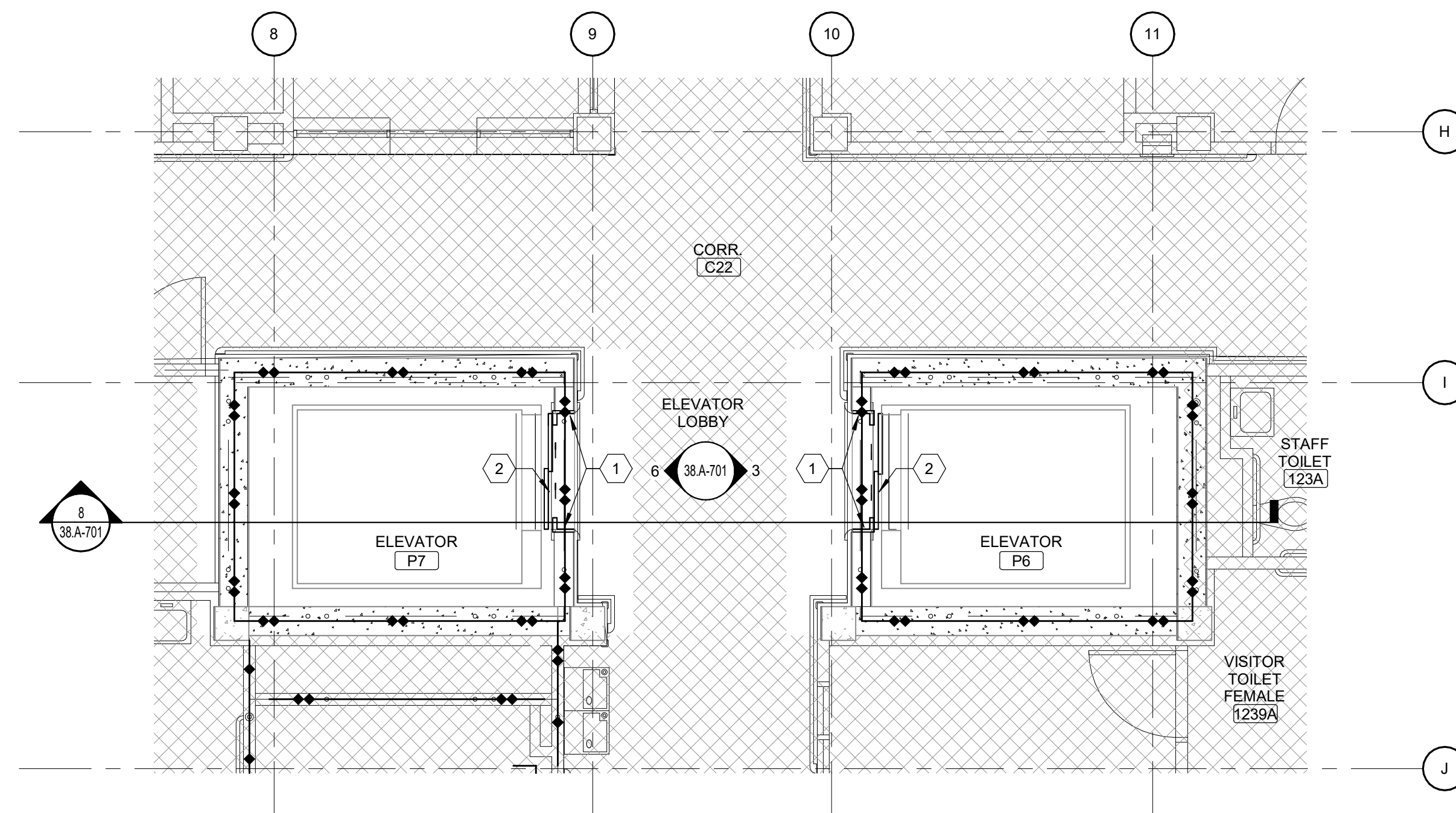
3 BUILDING 38 PARTIAL FIRST FLOOR PLAN Scale: 1/4" = 1'-0"
