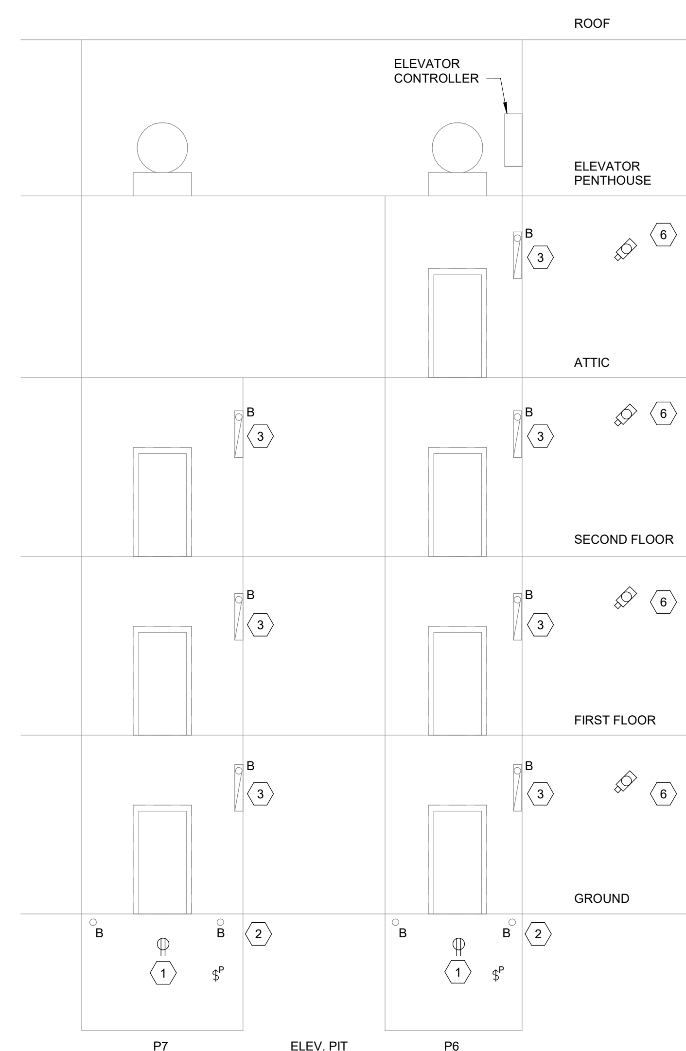
ELEVATORS - P6 & P7 BUILDING 38
