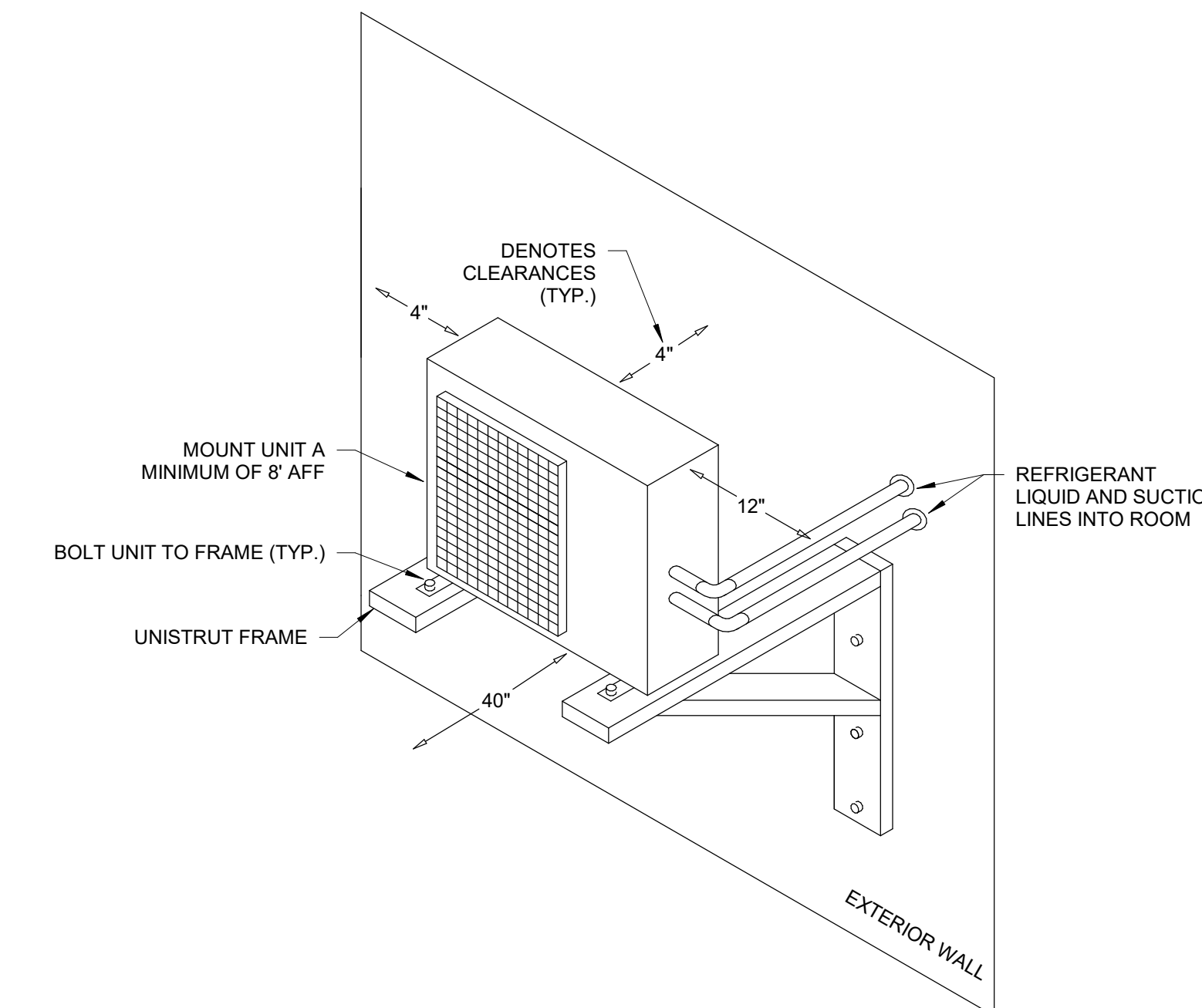
6 CONDENSING UNIT INSTALLATION DETAIL - ON WALL Scale: No Scale
