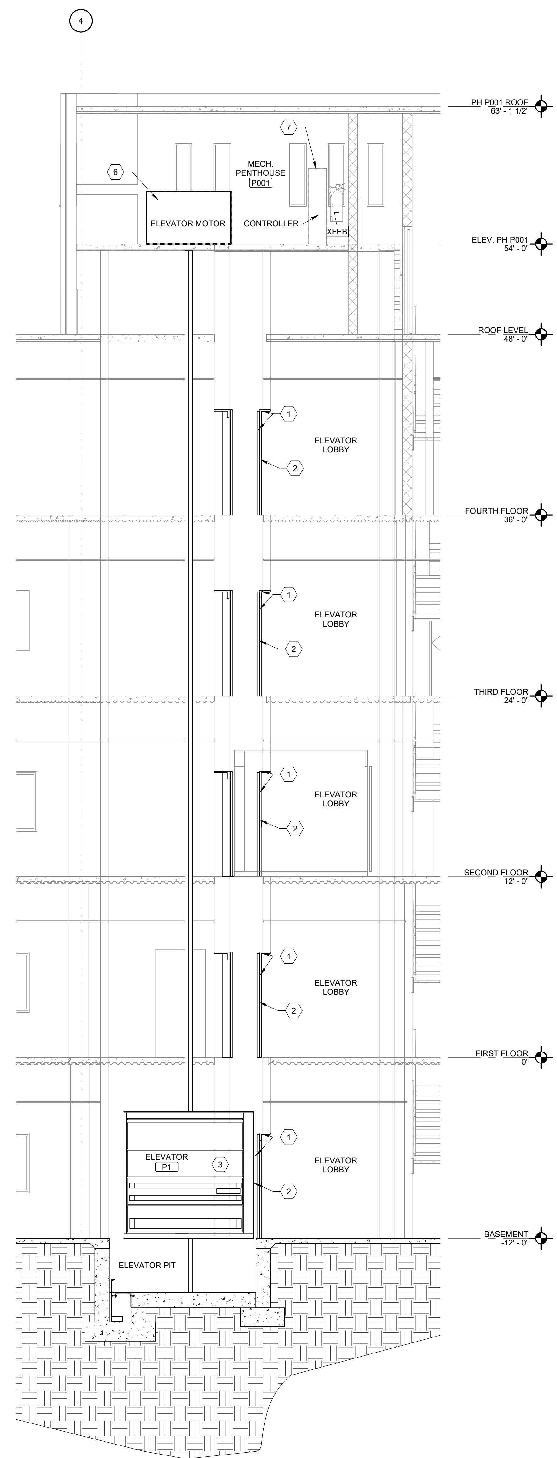
6 SECTION THROUGH ELEVATORS P1 AND P2 Scale: 1/4" = 1'-0"
