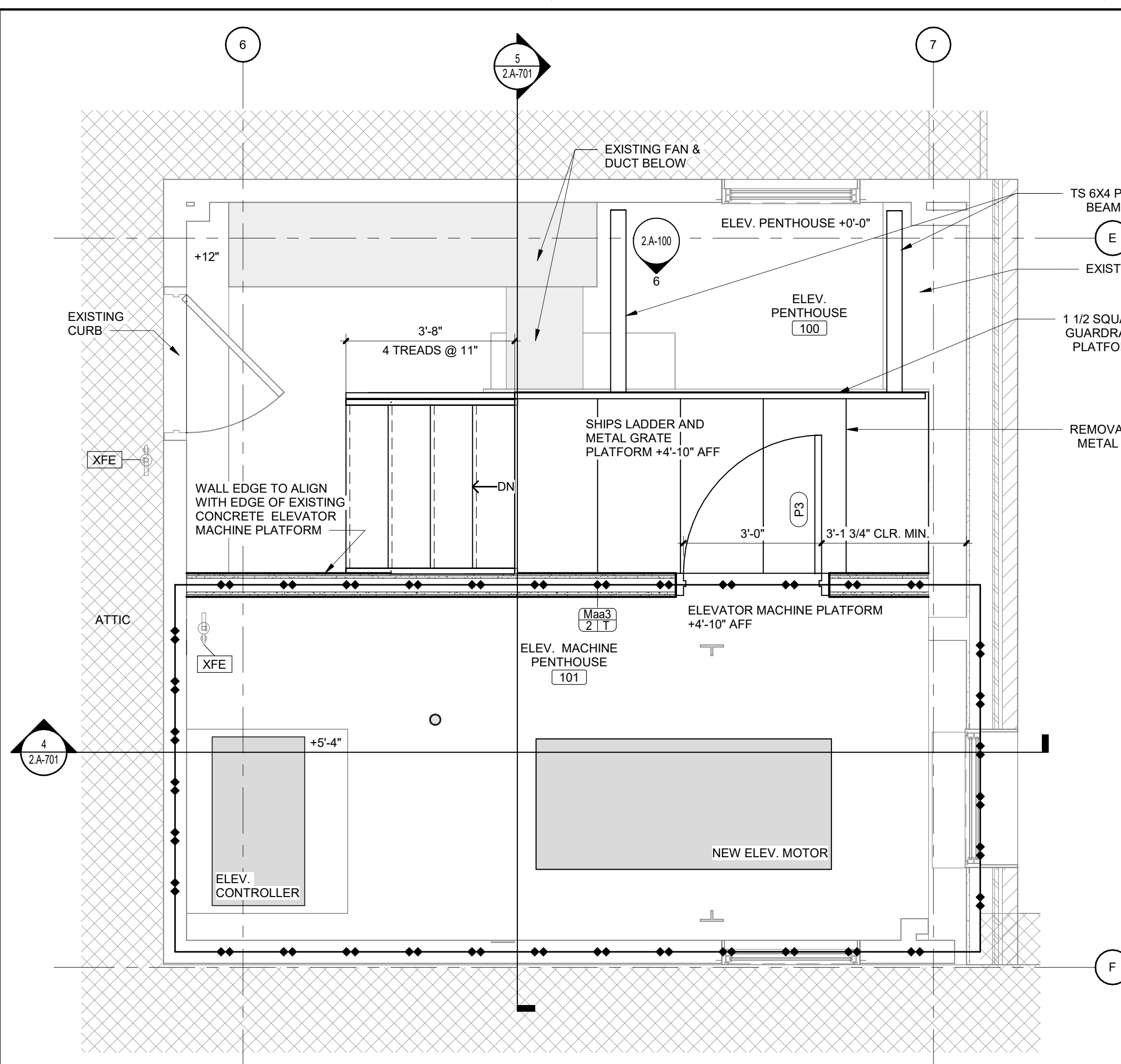
5 BUILDING 2 PARTIAL ATTIC FLOOR PLAN Scale: 1/2" = 1'-0"
