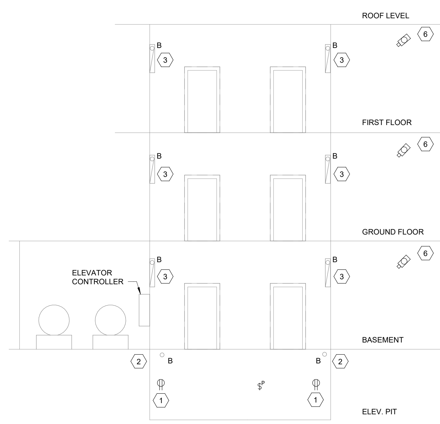
ELEVATORS - P14 & P15 BUILDING 135
