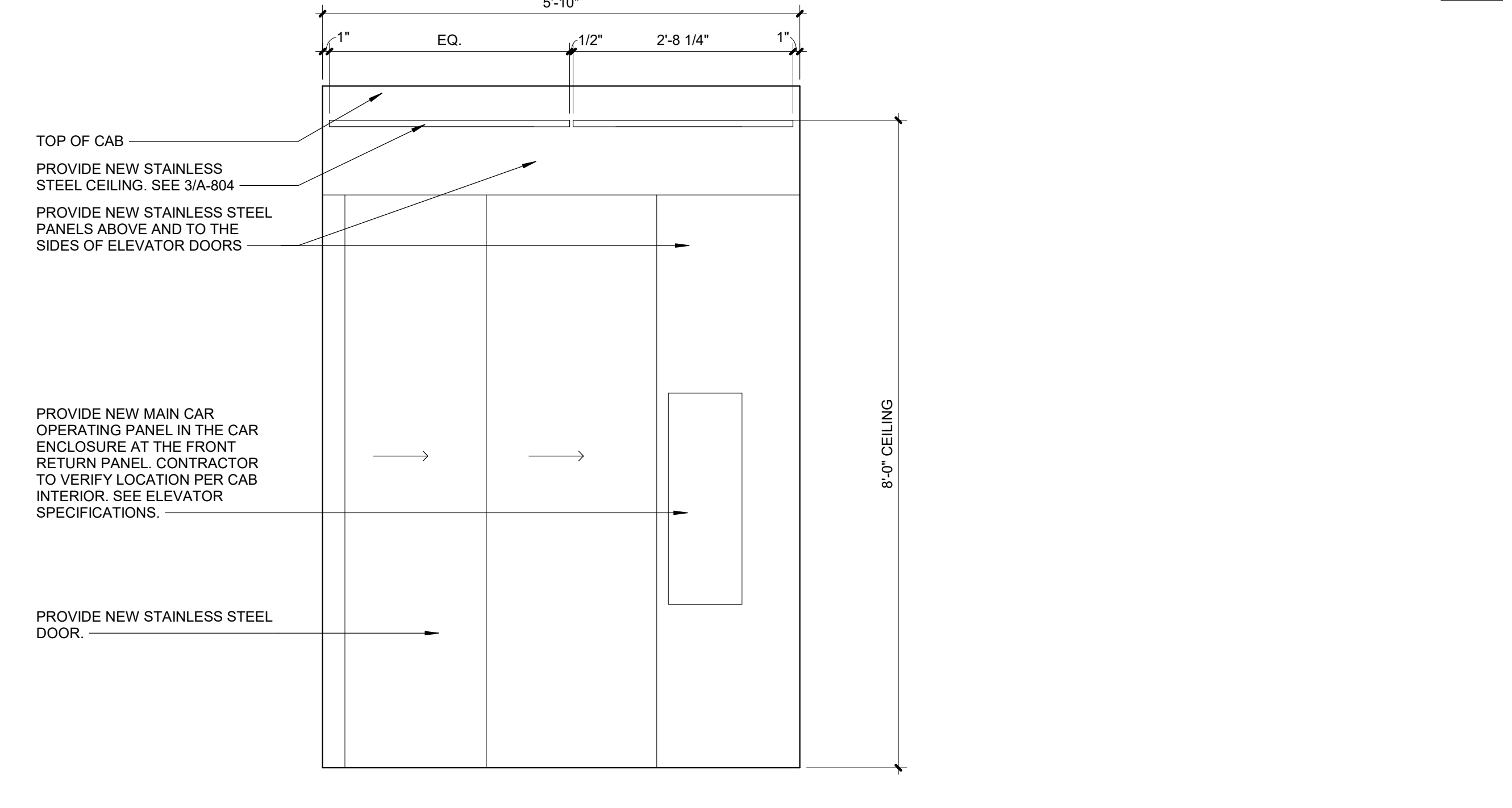
2 ELEVATOR CAB FRONT ELEVATION (P6 & P7) Scale: 3/4" = 1'-0"
