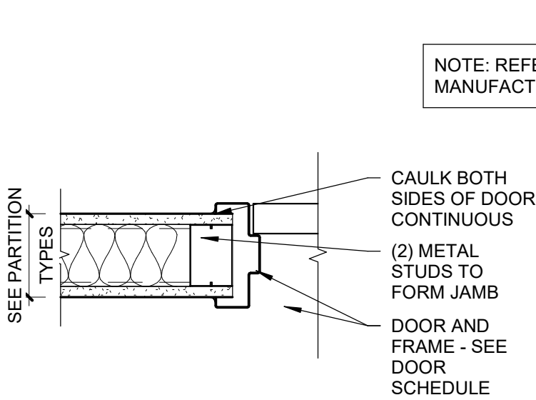
J1 JAMB DETAIL @ METAL STUD Scale: 1 1/2" = 1'-0"
