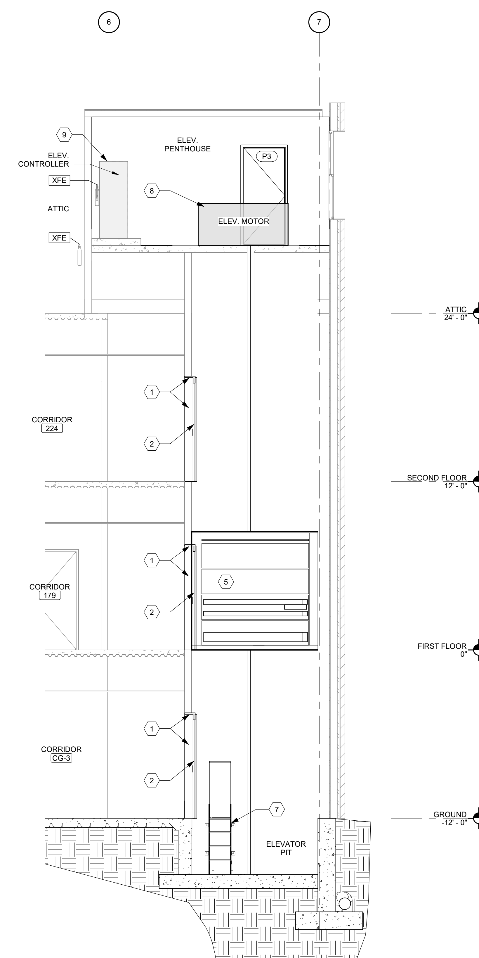
4 SECTION THROUGH ELEVATOR P3 Scale: 1/4" = 1'-0"
