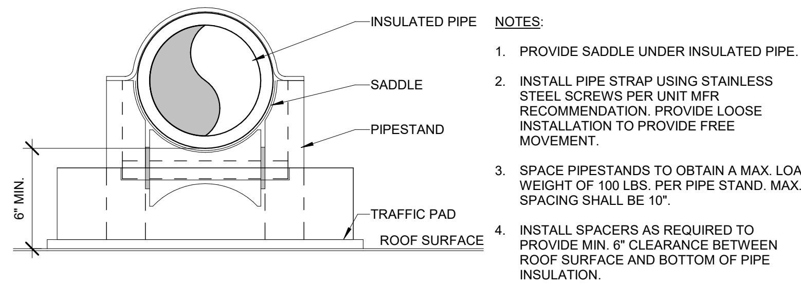
9 ROOFTOP PIPESTAND DETAIL Scale: No Scale
