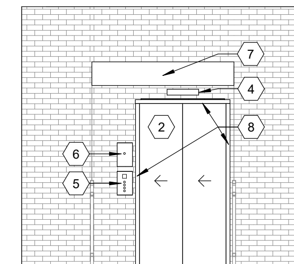
3 ELEVATOR @ BASEMENT - BLDG 5 - P13 - INT Scale: 1/4" = 1'-0"
