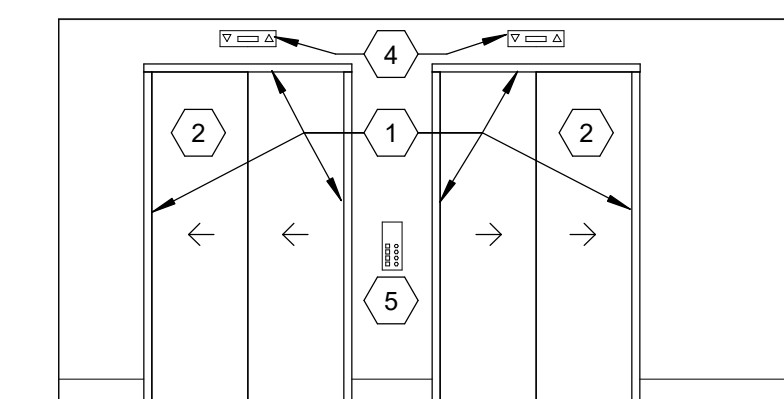
2 ELEVATOR @ GROUND FLOOR - P14 & P15 Scale: 1/4" = 1'-0"
