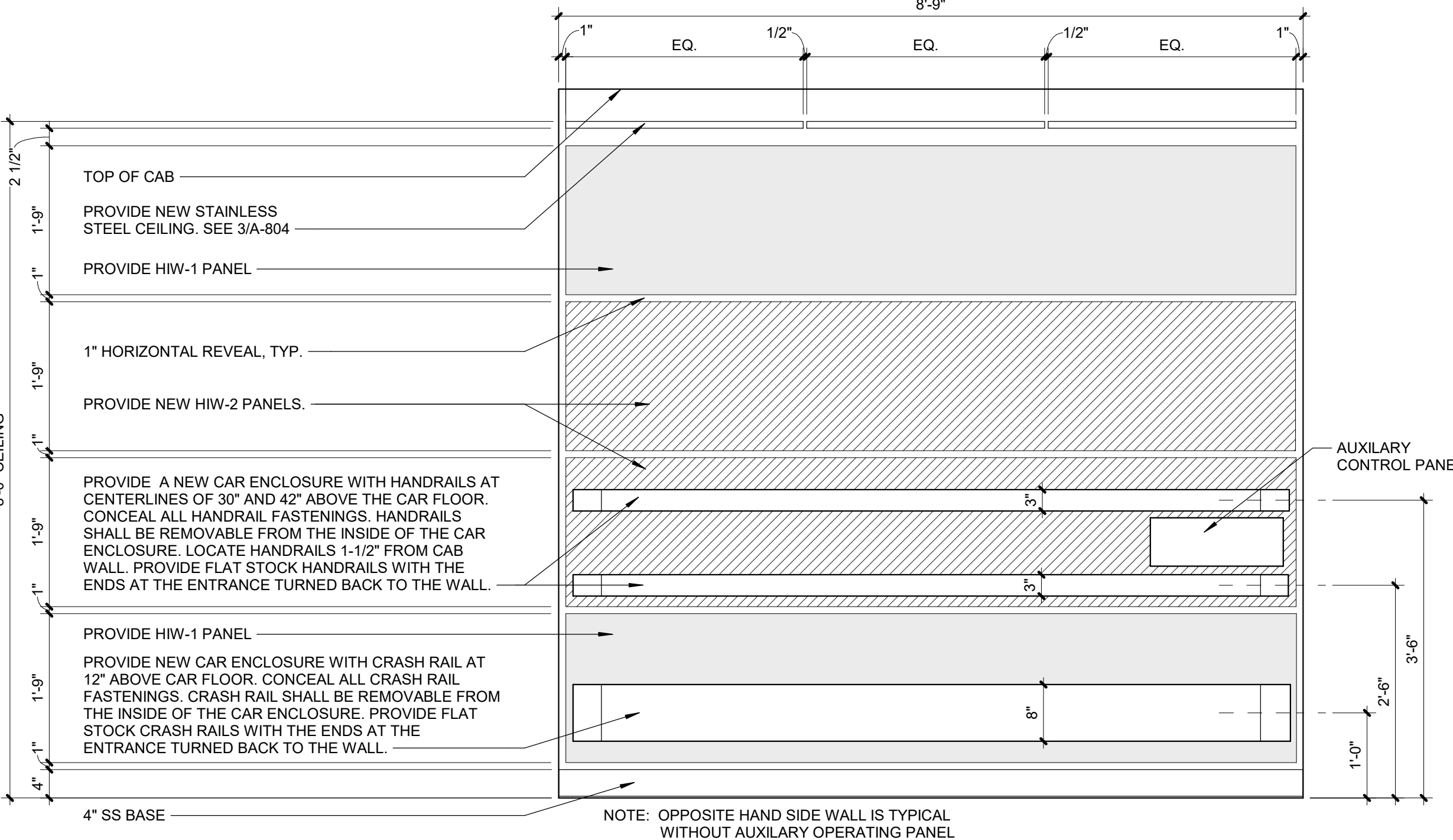
4 ELEVATOR CAB SIDE ELEVATION (P6 & P7) Scale: 3/4" = 1'-0"
