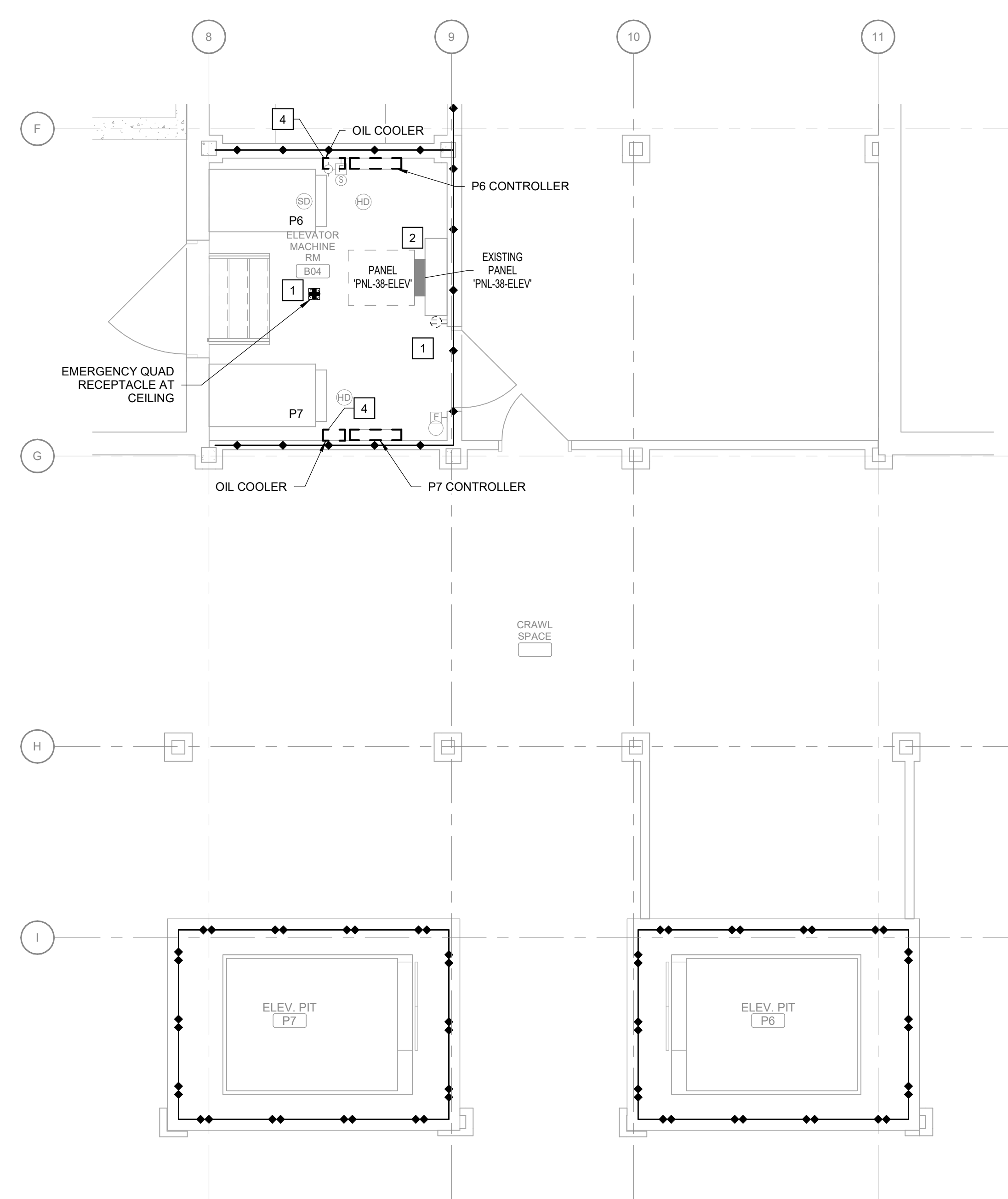
1 BUILDING 38 PARTIAL BASEMENT ELECTRICAL DEMOLITION PLAN - P6 & P7 Scale: 1/4" = 1'-0"
