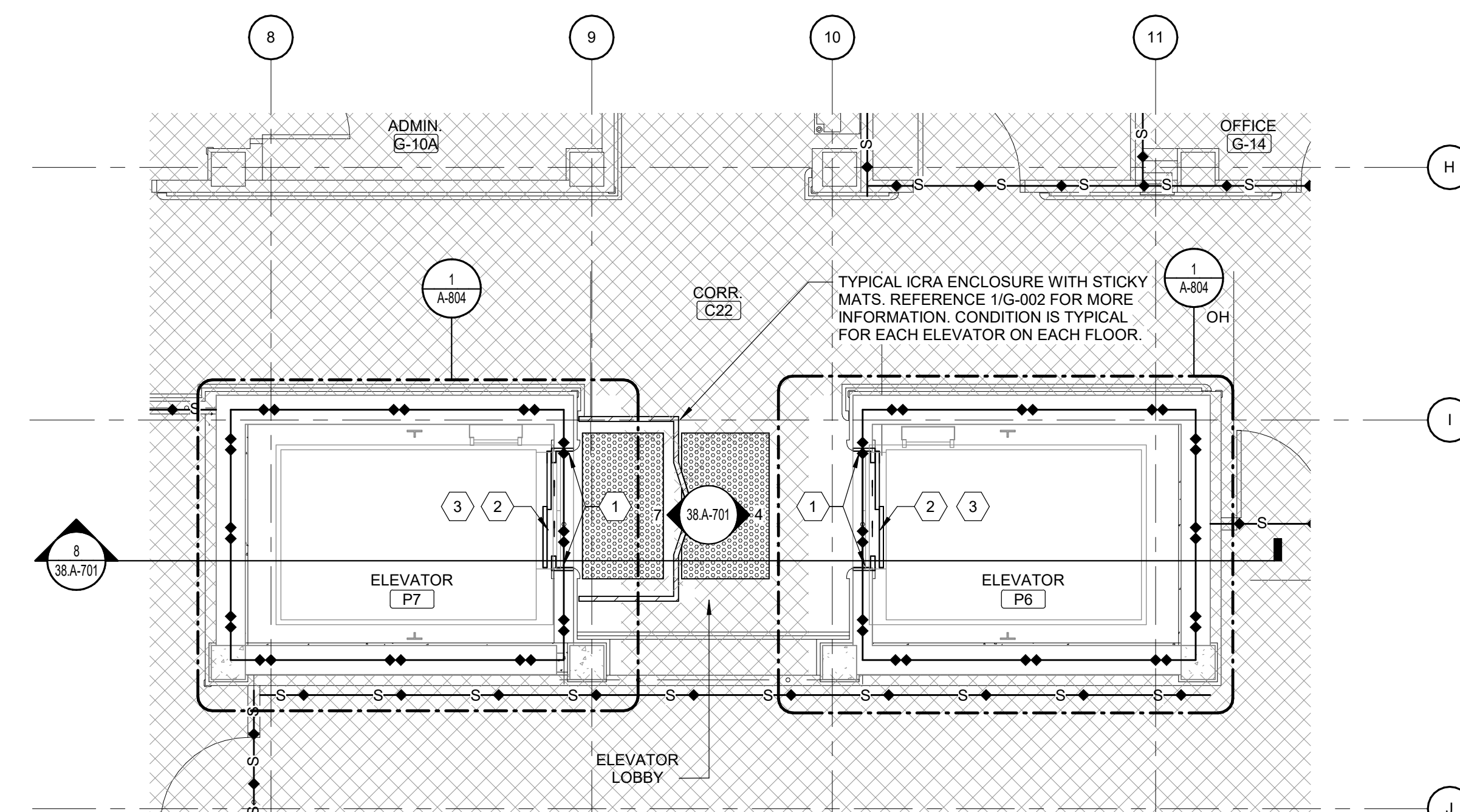
2 BUILDING 38 PARTIAL GROUND FLOOR PLAN Scale: 1/4" = 1'-0"
