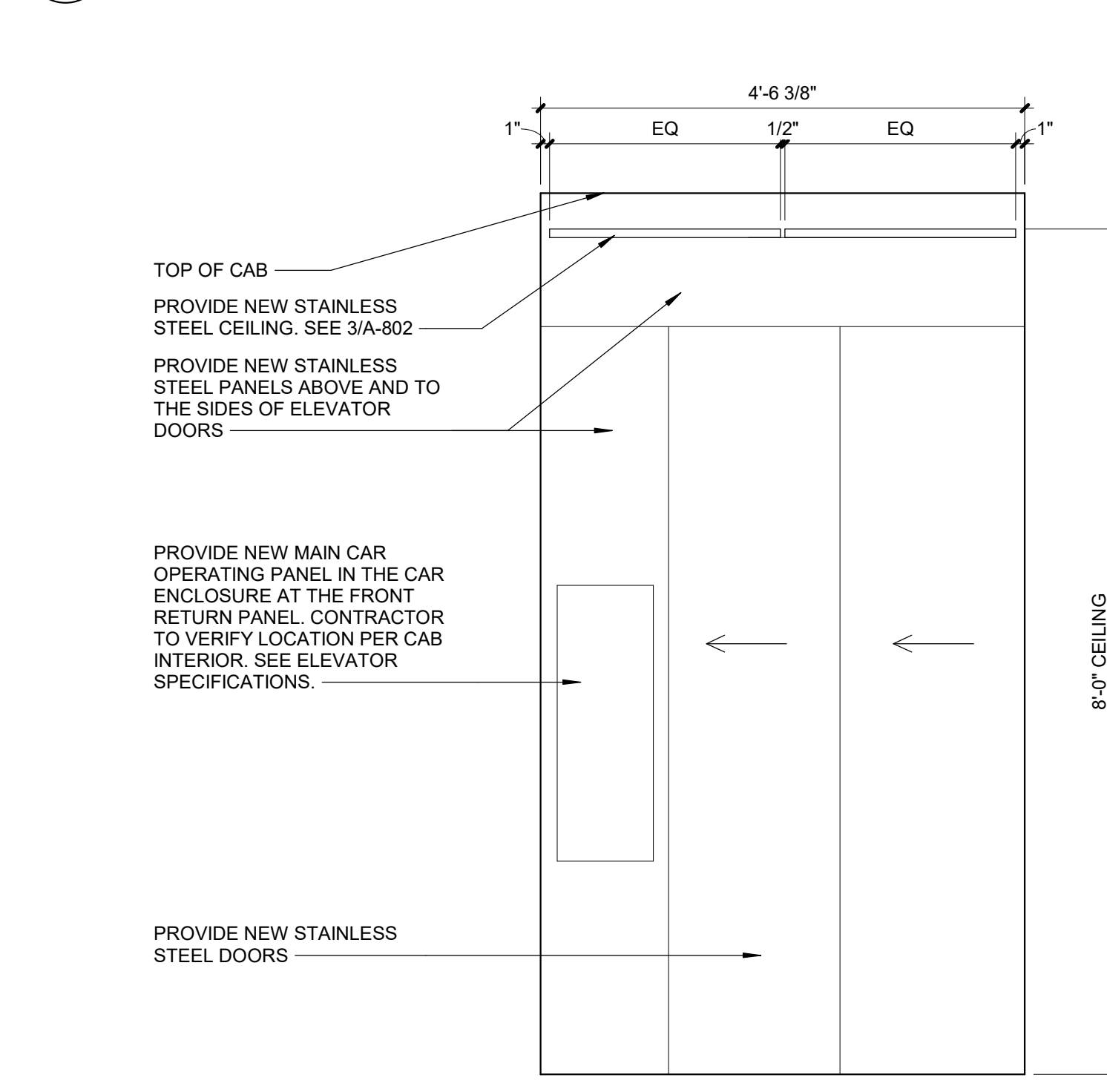
2 ELEVATOR CAB FRONT ELEVATION (P3) Scale: 3/4" = 1'-0"
