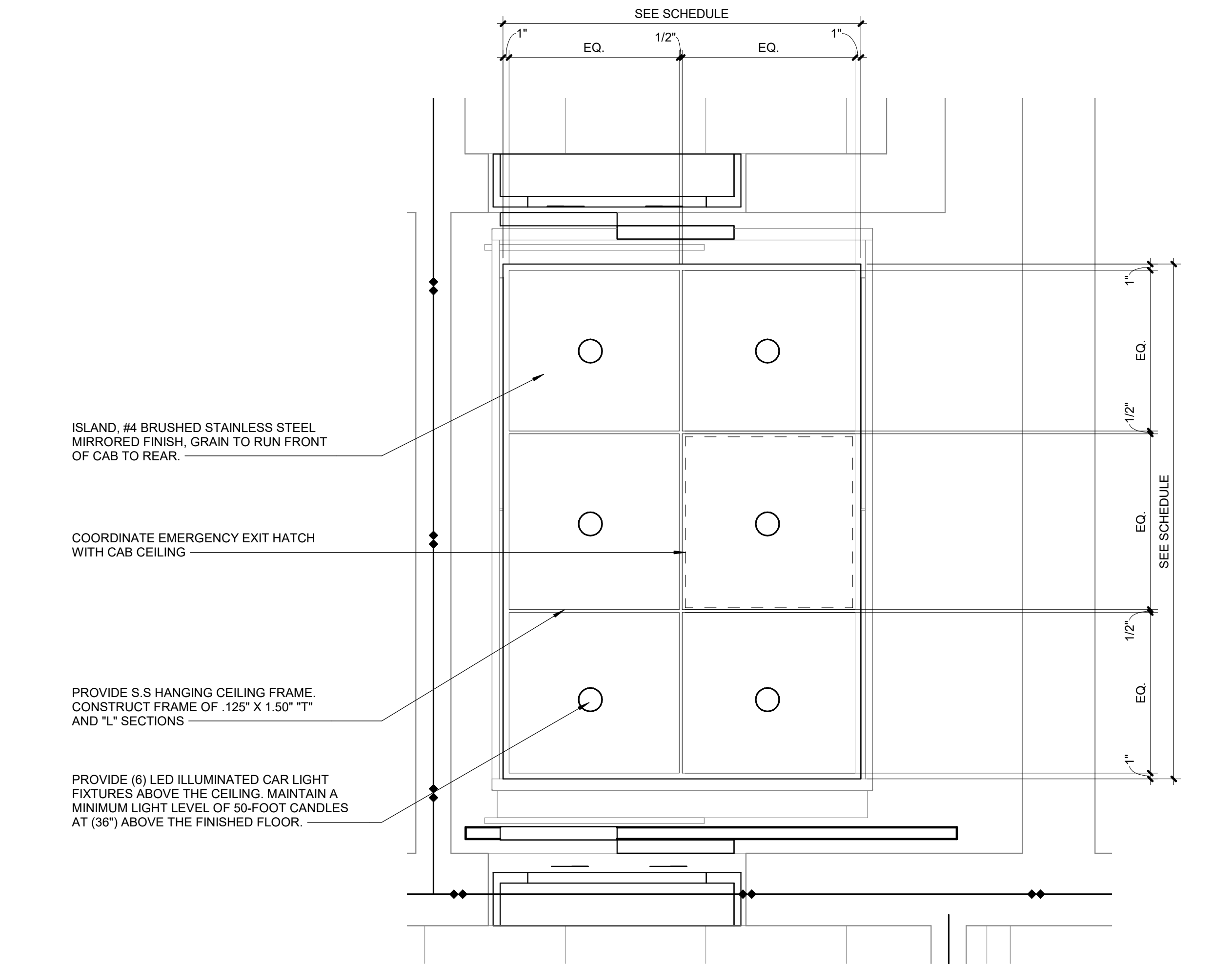
3 BUILDING 5 ELEVATOR REFLECTED CEILING PLAN (P13) Scale: 3/4" = 1'-0"
