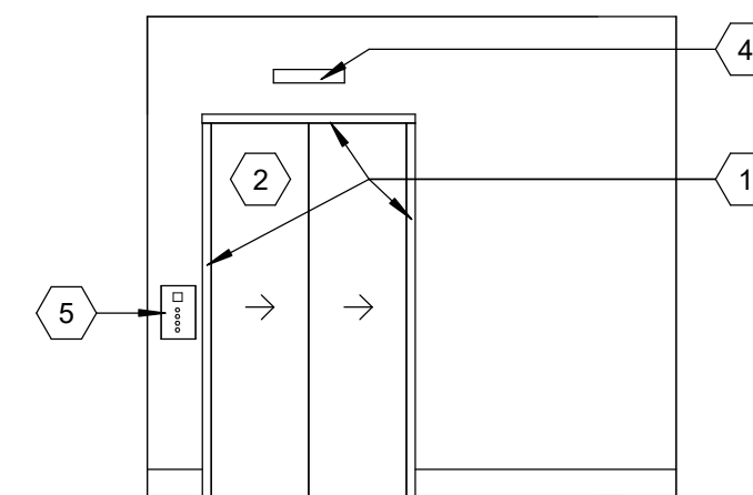
1 ELEVATOR @ SECOND FLOOR - BLDG 5 - P13 - INT Scale: 1/4" = 1'-0"
