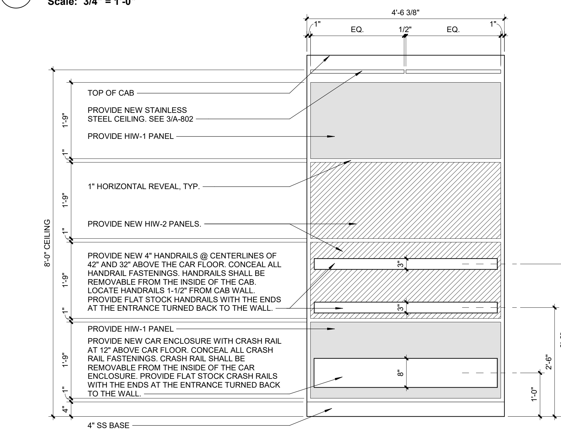
5 ELEVATOR CAB REAR ELEVATION (P3) Scale: 3/4" = 1'-0"
