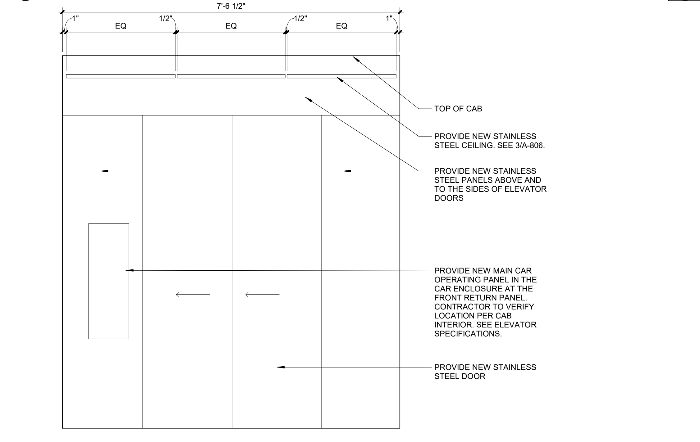
2 ELEVATOR CAB FRONT ELEVATION (P17 - P19) Scale: 3/4" = 1'-0"
