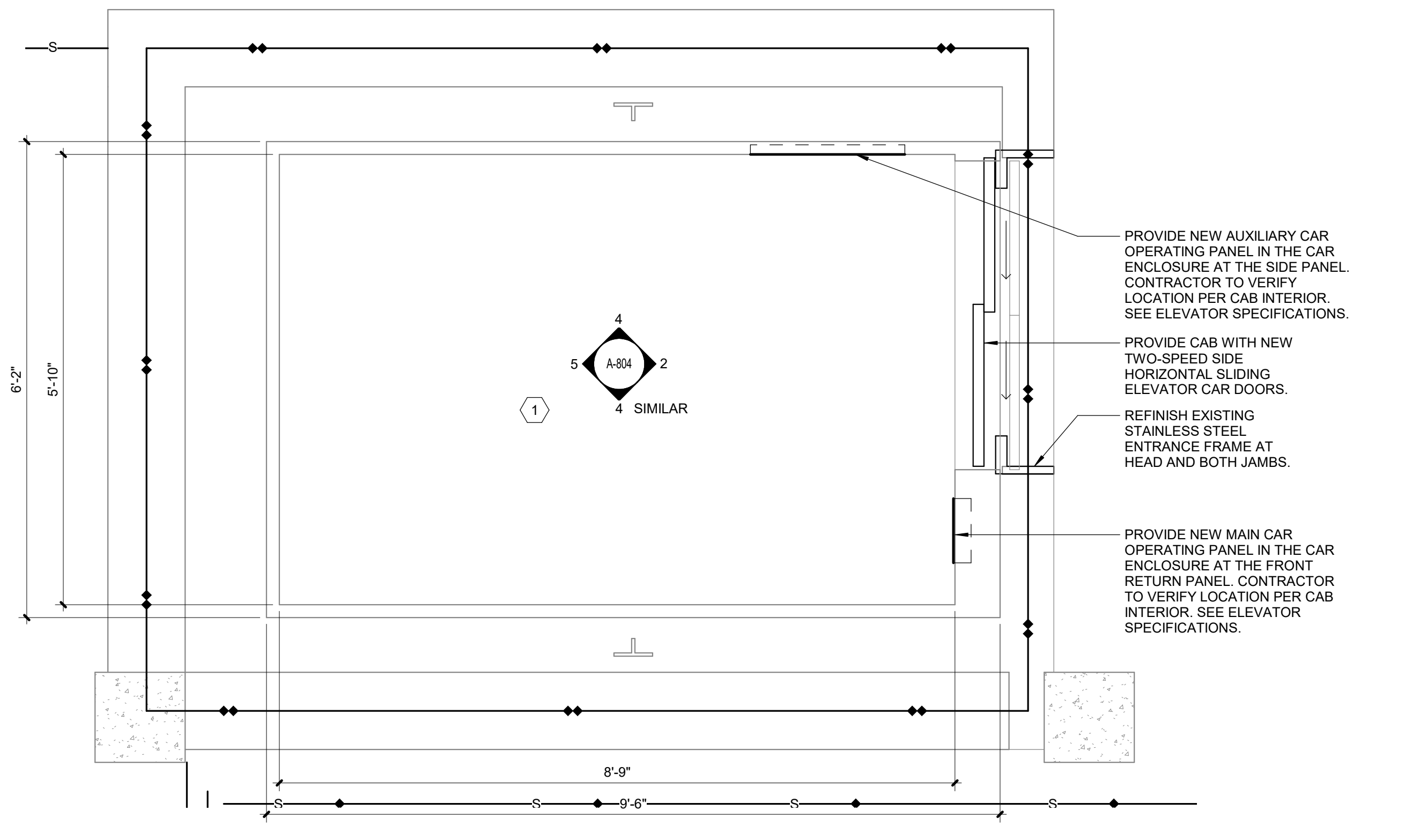
1 BUILDING 38 TYPICAL ELEVATOR FLOOR PLAN (P6 - P7) Scale: 3/4" = 1'-0"
