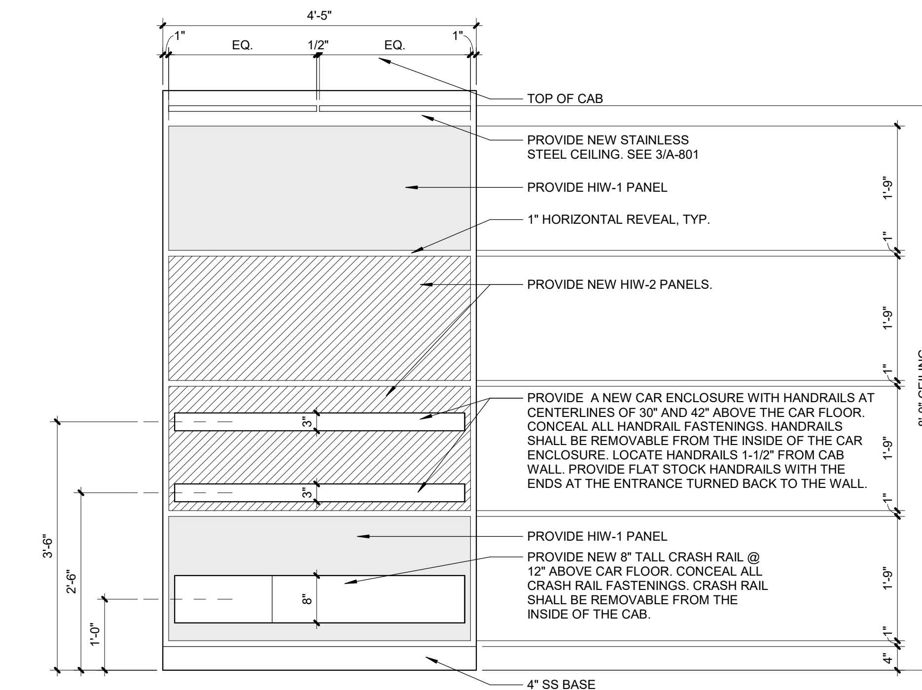
5 ELEVATOR CAB REAR ELEVATION (P1 & P2) Scale: 3/4" = 1'-0"
