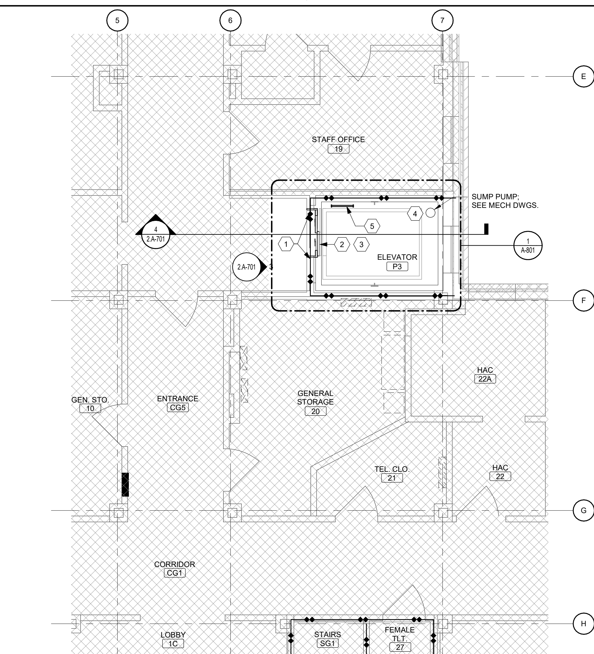
1 BUILDING 2 PARTIAL GROUND FLOOR PLAN Scale: 1/4" = 1'-0"
