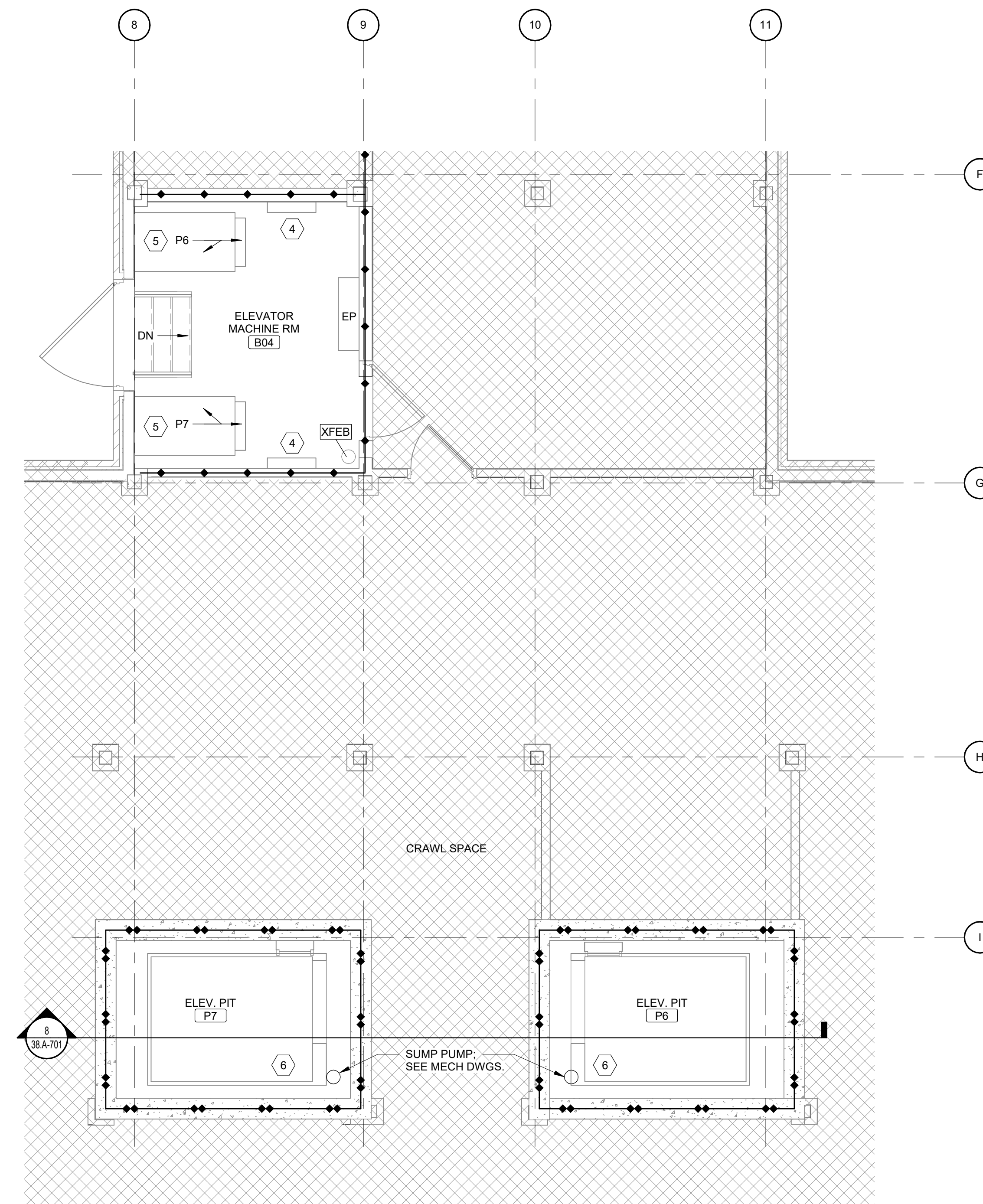
1 BUILDING 38 PARTIAL BASEMENT FLOOR PLAN Scale: 1/4" = 1'-0"
