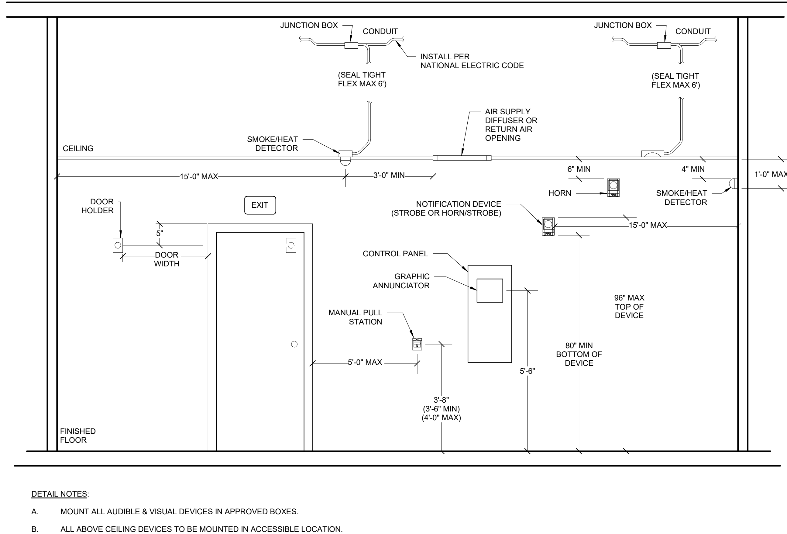
1 FIRE ALARM DEVICE MOUNTING HEIGHTS Scale: No Scale
