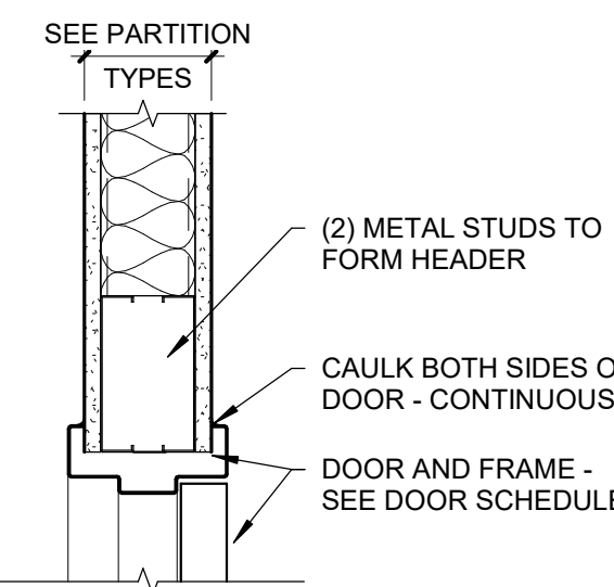
H1 HEAD DETAIL @ METAL STUD Scale: 1 1/2" = 1'-0"
