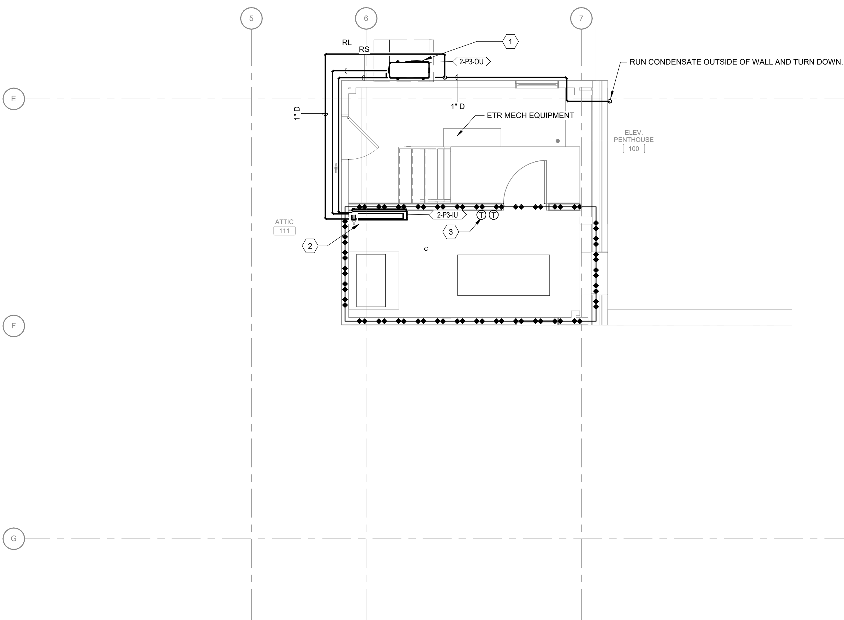
2 BUILDING 2 PARTIAL ATTIC MECHANICAL PLAN - P3 Scale: 1/4" = 1'-0"
