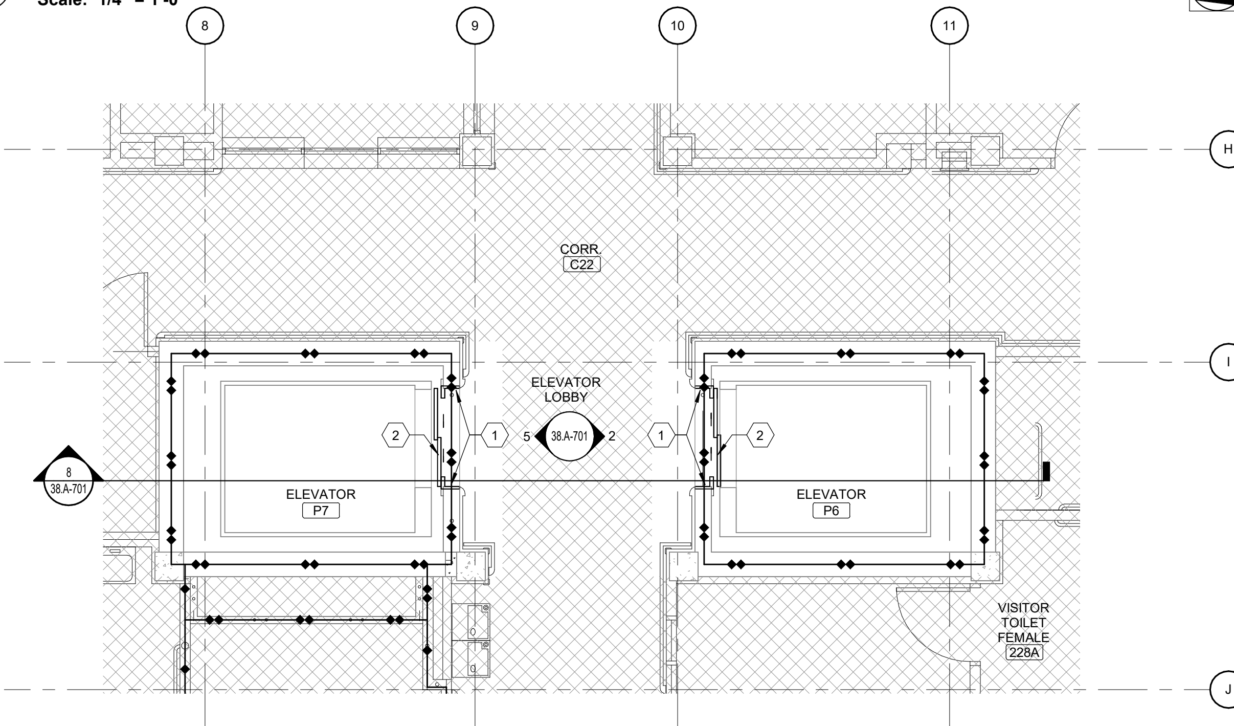
4 BUILDING 38 PARTIAL SECOND FLOOR PLAN Scale: 1/4" = 1'-0"
