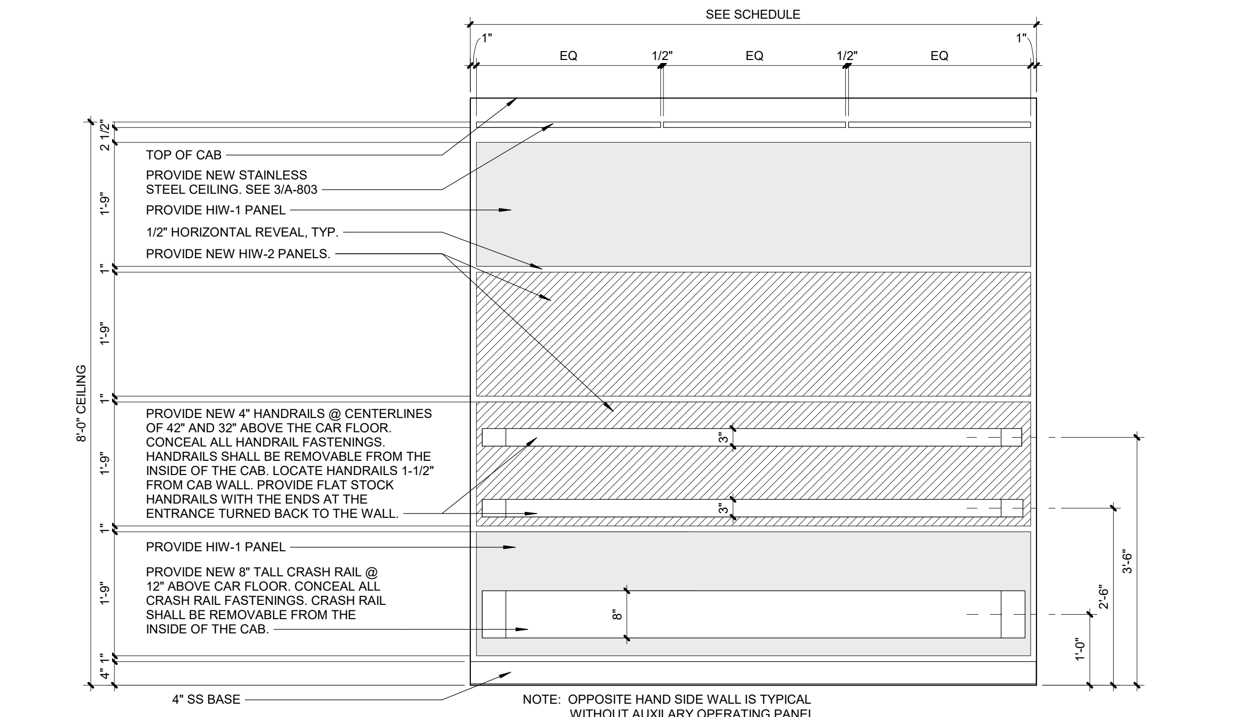
4 ELEVATOR CAB SIDE ELEVATION (P13) Scale: 3/4" = 1'-0"
