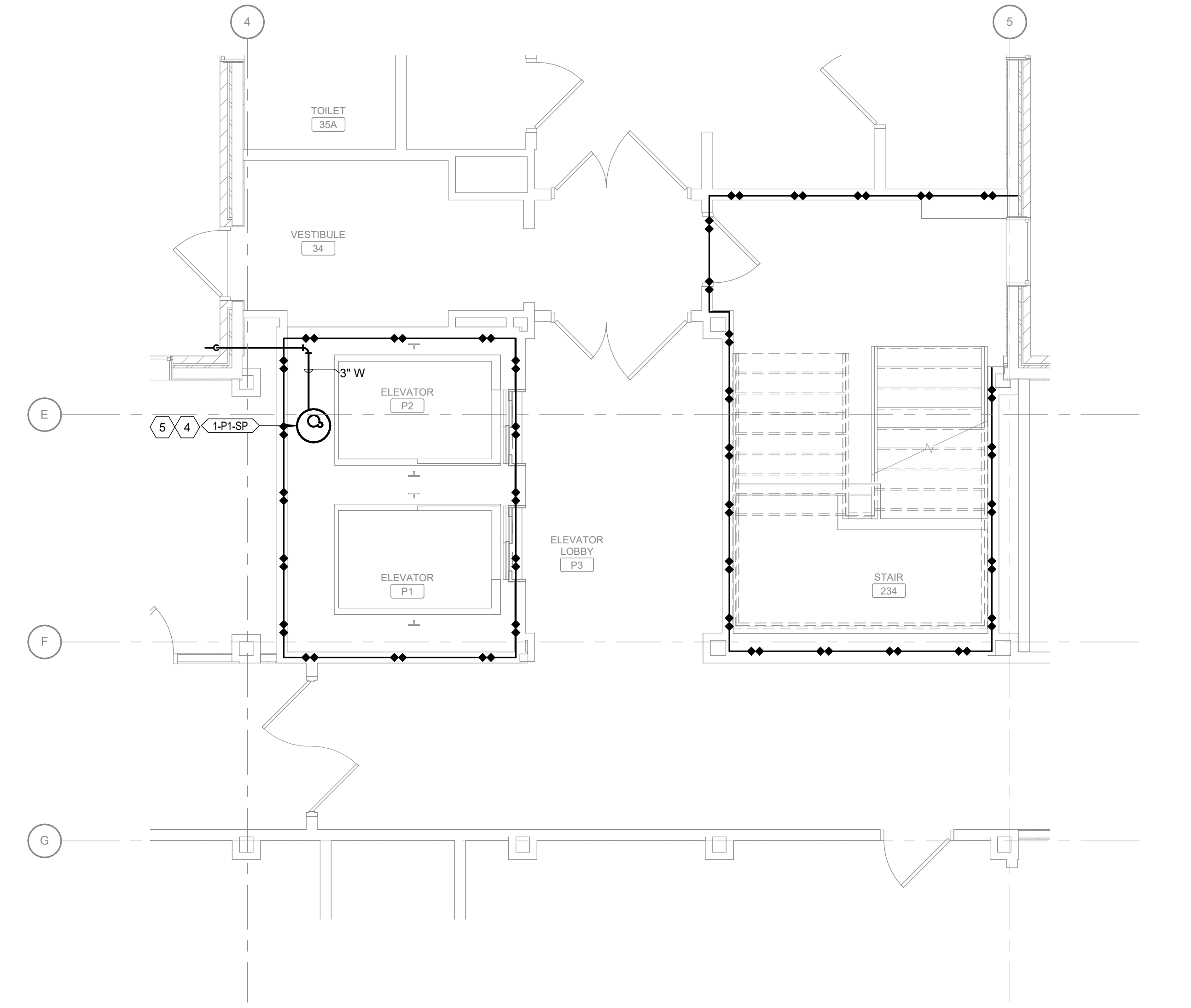
2 BUILDING 1 PARTIAL BASEMENT MECHANICAL PLAN - P1 & P2 Scale: 1/4" = 1'-0"
