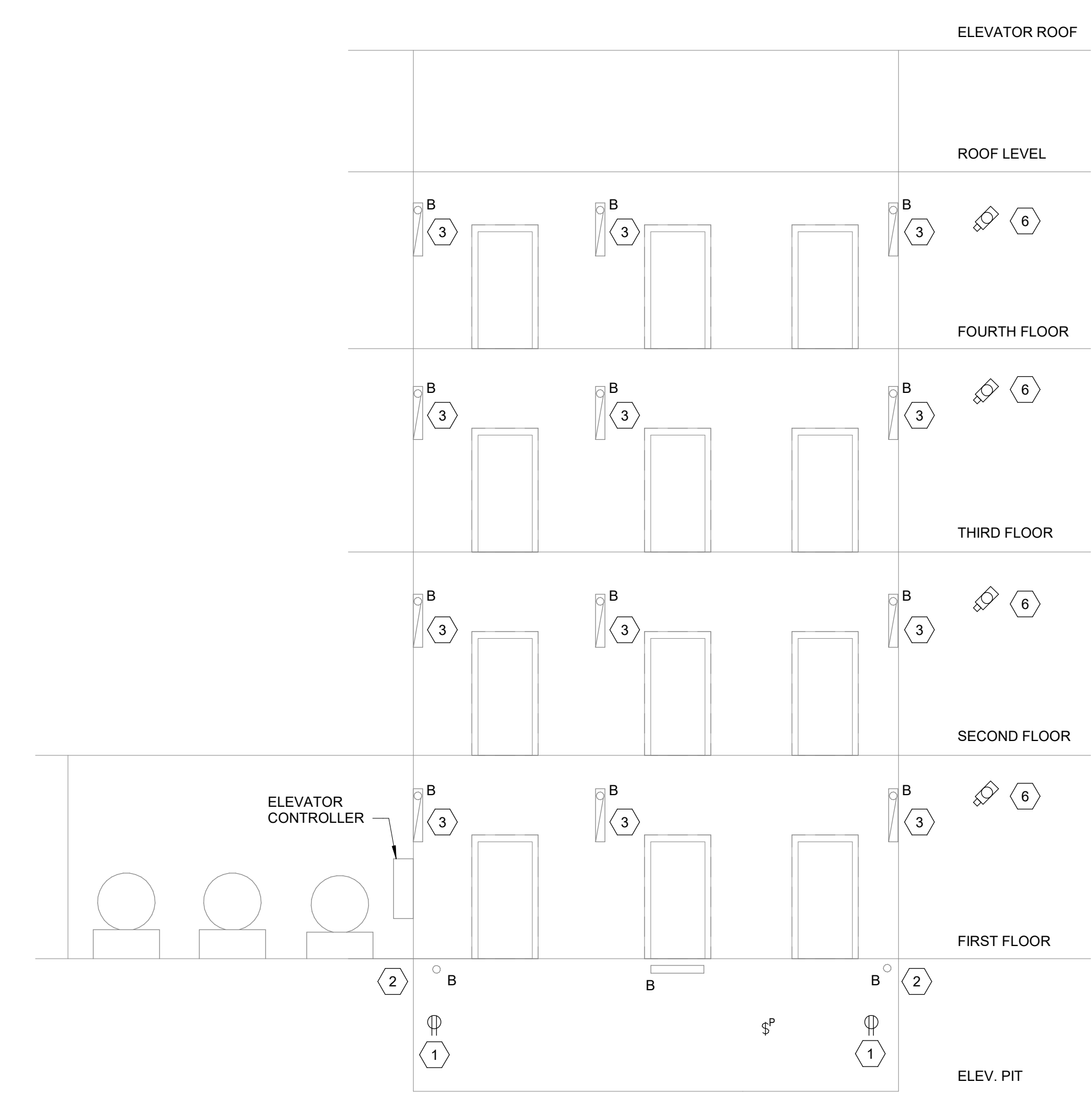
ELEVATORS - P17, P18 & P19 BUILDING 137
