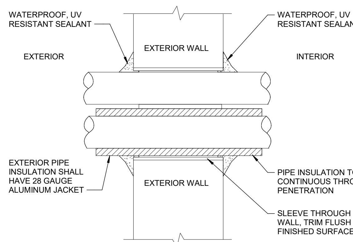
5 PIPE WALL PENETRATION Scale: No Scale
