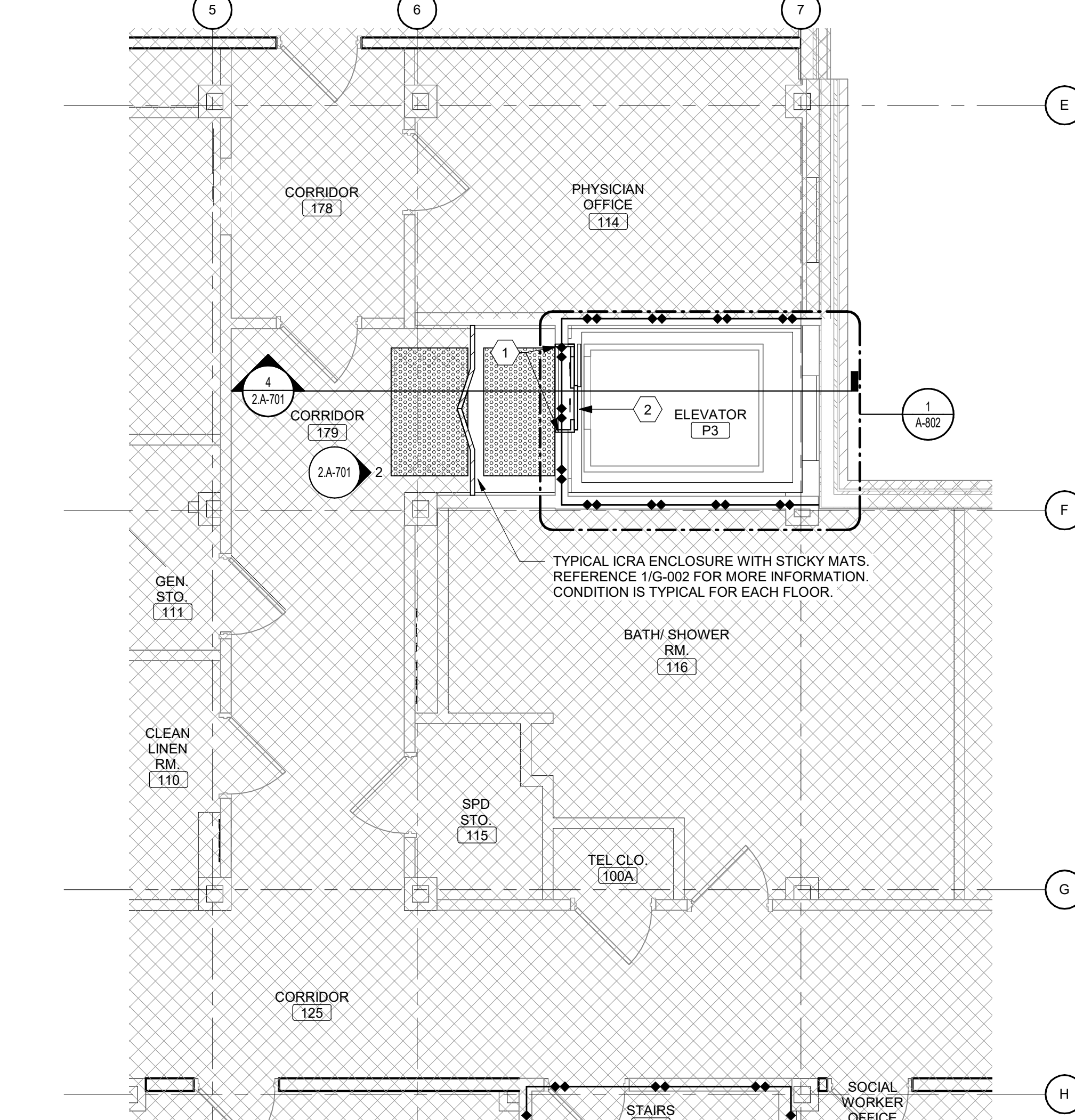
2 BUILDING 2 PARTIAL FIRST FLOOR PLAN Scale: 1/4" = 1'-0"
