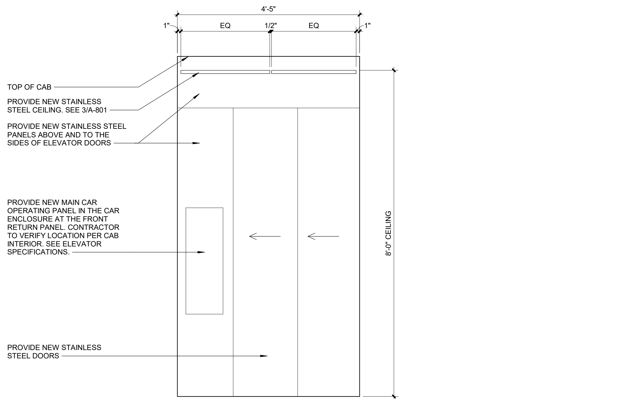
2 ELEVATOR CAB FRONT ELEVATION (P1 & P2) Scale: 3/4" = 1'-0"
