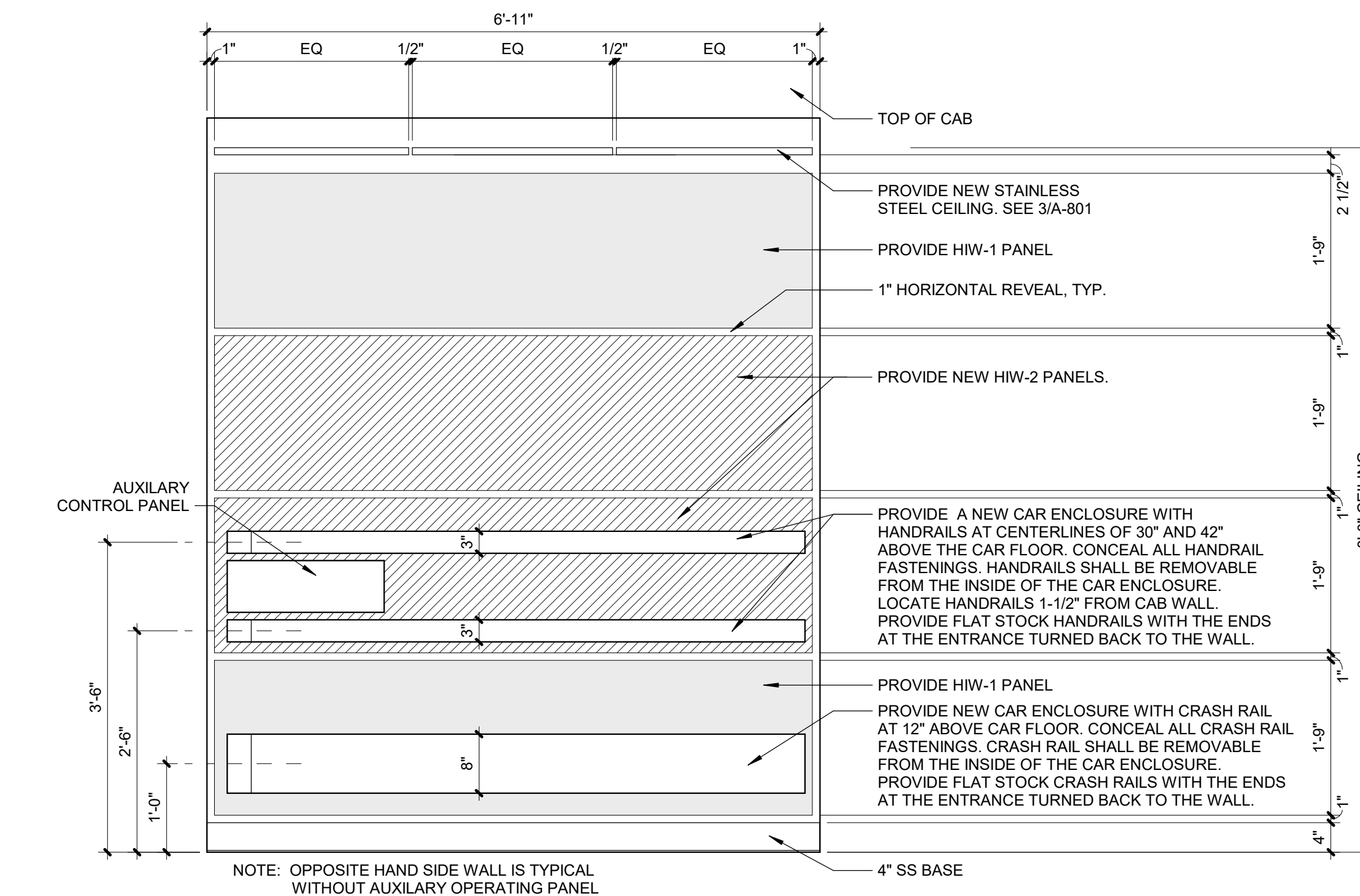
4 ELEVATOR CAB SIDE ELEVATION (P1 & P2) Scale: 3/4" = 1'-0"
