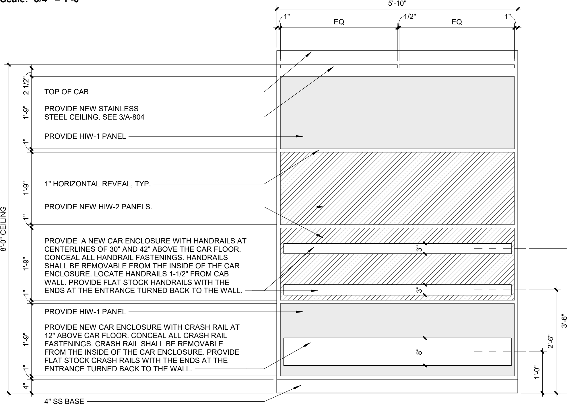
5 ELEVATOR CAB REAR ELEVATION (P6 & P7) Scale: 3/4" = 1'-0"
