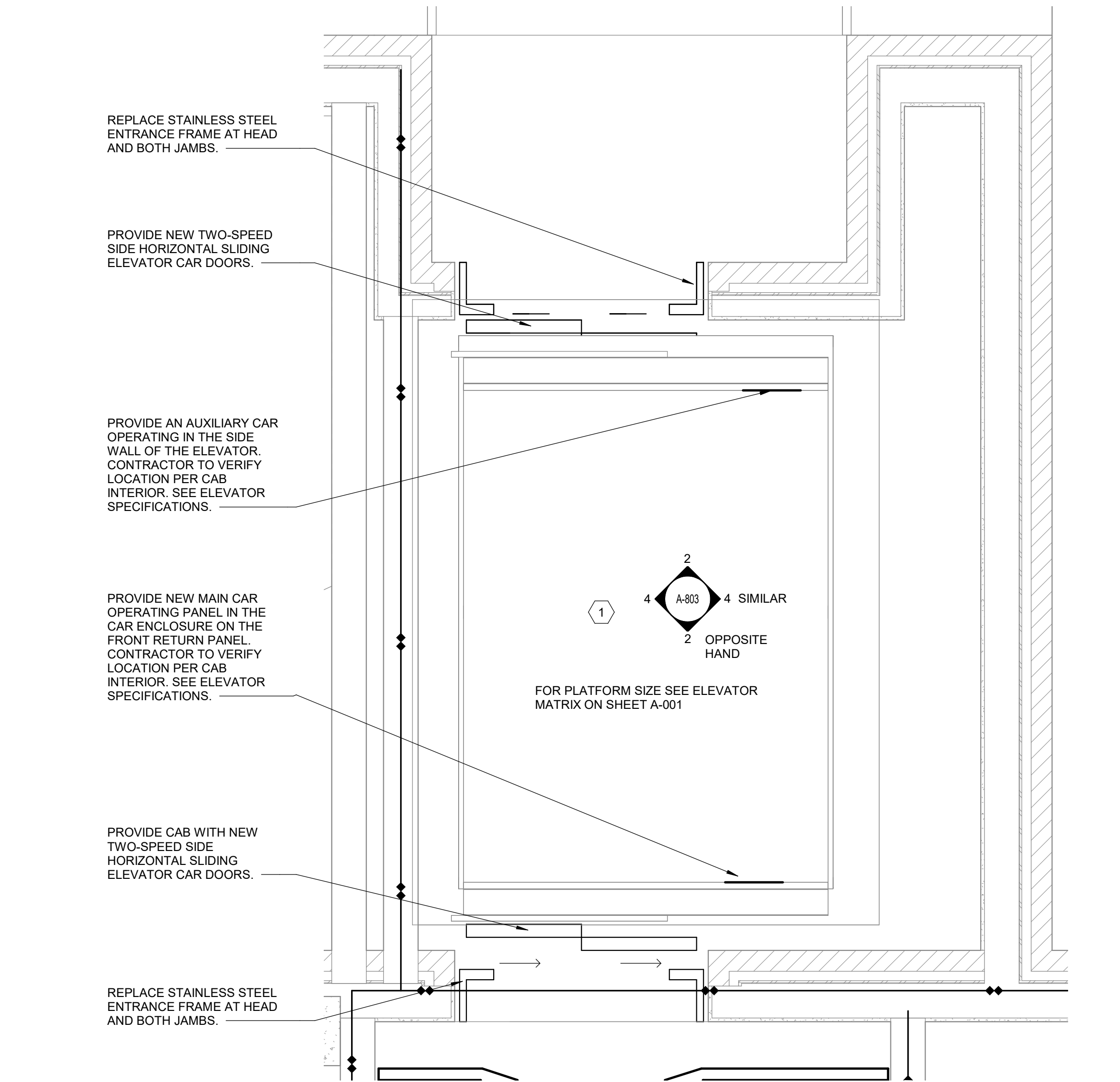
1 BUILDING 5 TYPICAL ELEVATOR FLOOR PLAN (P13) Scale: 3/4" = 1'-0"
