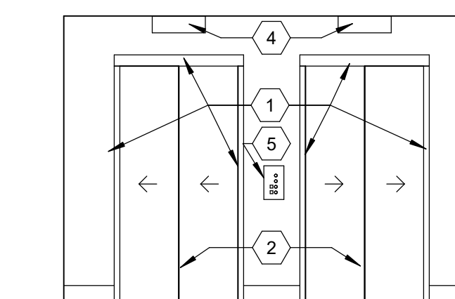
4 ELEVATORS @ FIRST FLOOR - BLDG 1 - P1 & P2 Scale: 1/4" = 1'-0"
