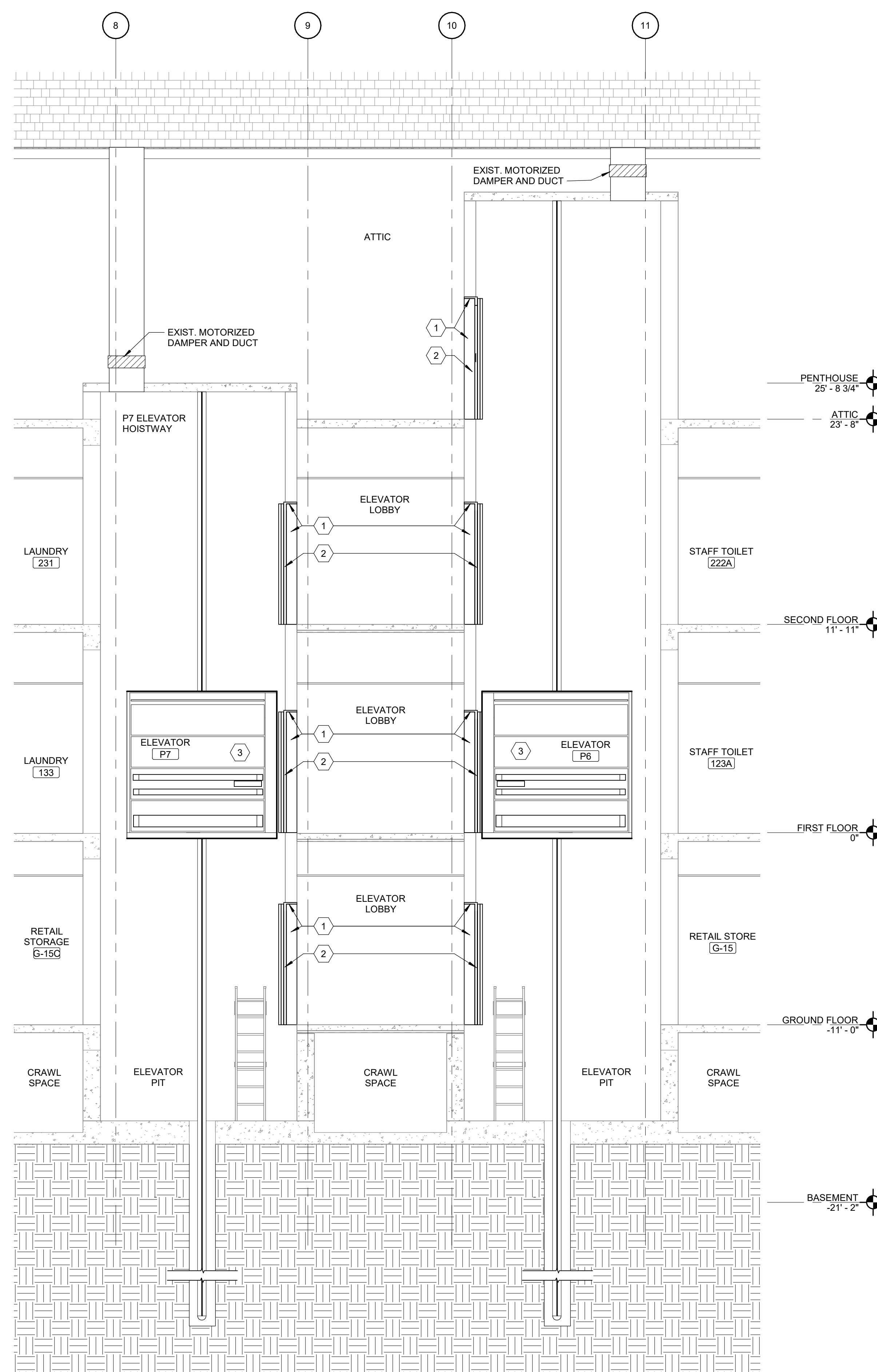
8 SECTION THROUGH ELEVATORS P7-P6 Scale: 1/4" = 1'-0"
