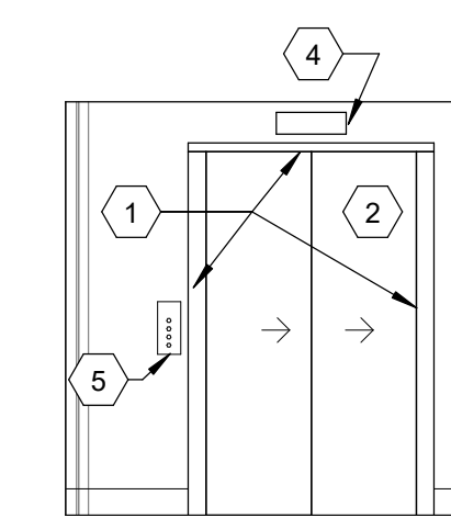
6 ELEV. @ FIRST FLOOR - P7 Scale: 1/4" = 1'-0"
