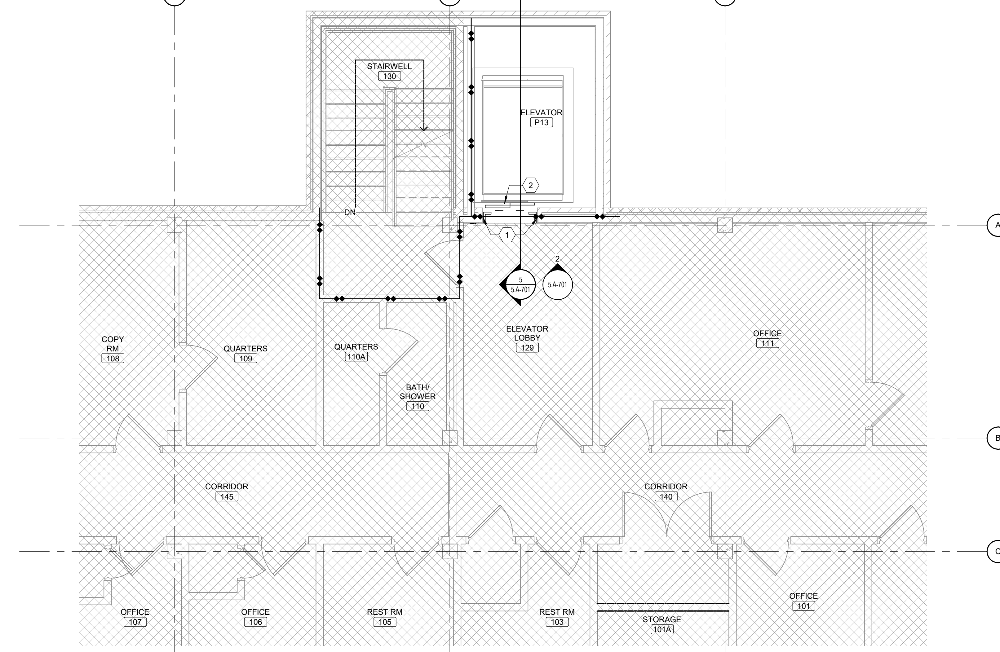
2 BUILDING 5 PARTIAL FIRST FLOOR PLAN Scale: 1/4" = 1'-0"
