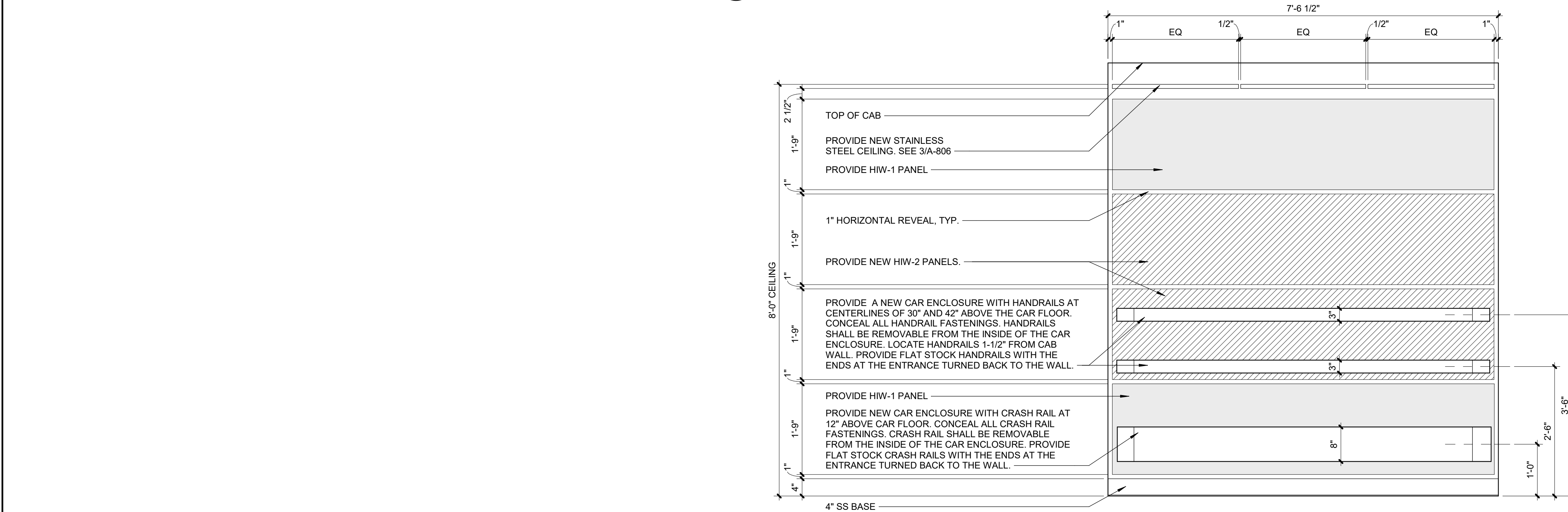
4 ELEVATOR CAB REAR ELEVATION (P17 - P19) Scale: 3/4" = 1'-0"
