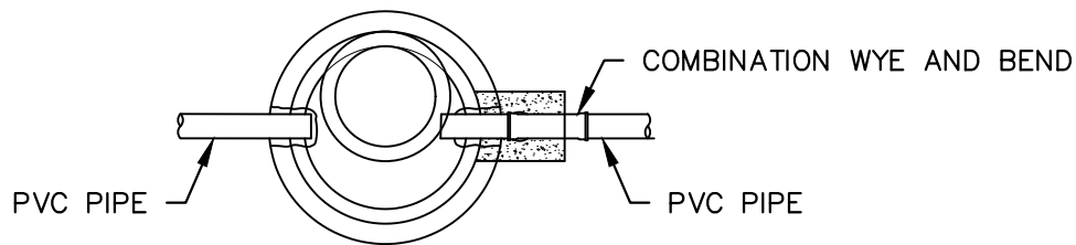
PLAN VIEW
