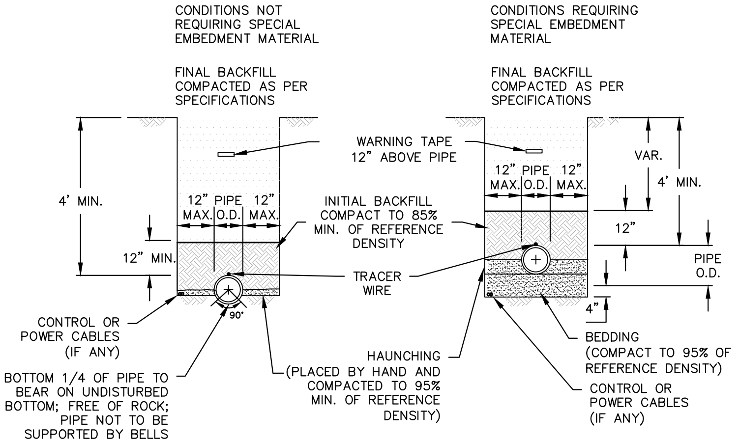
1A TYPICAL TRENCH SECTION NTS
