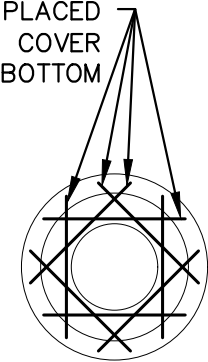
BAR PLACEMENT
