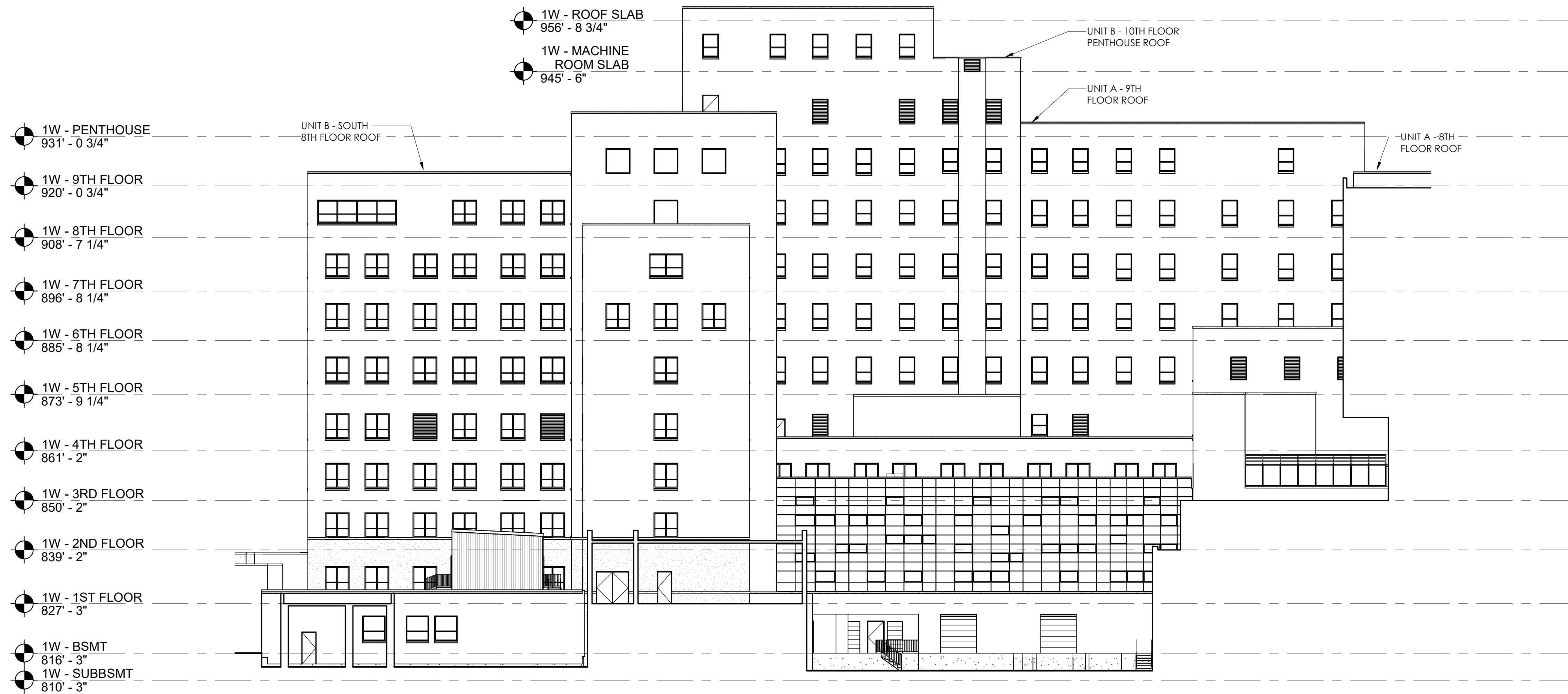
02 EAST ELEVATION 01W-AS201 SCALE: 1/16" = 1'-0"
