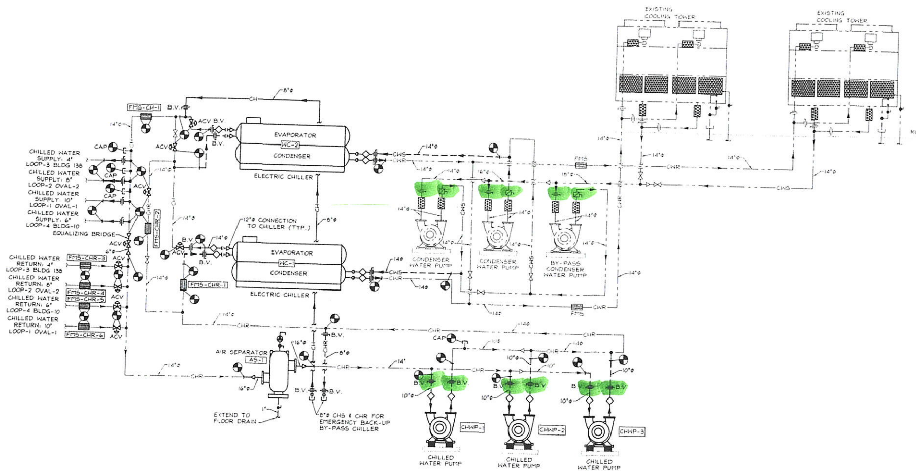
CHILLED & CONDENSER WATER FLOW DIAGRAM NOT TO SCALE
