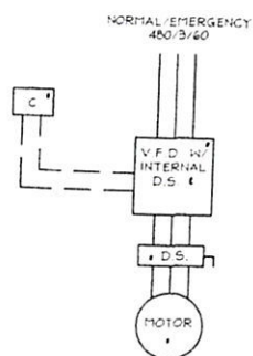
CHILLED WATER PUMP CHWP-3 125 HP (FREE STANDING)
