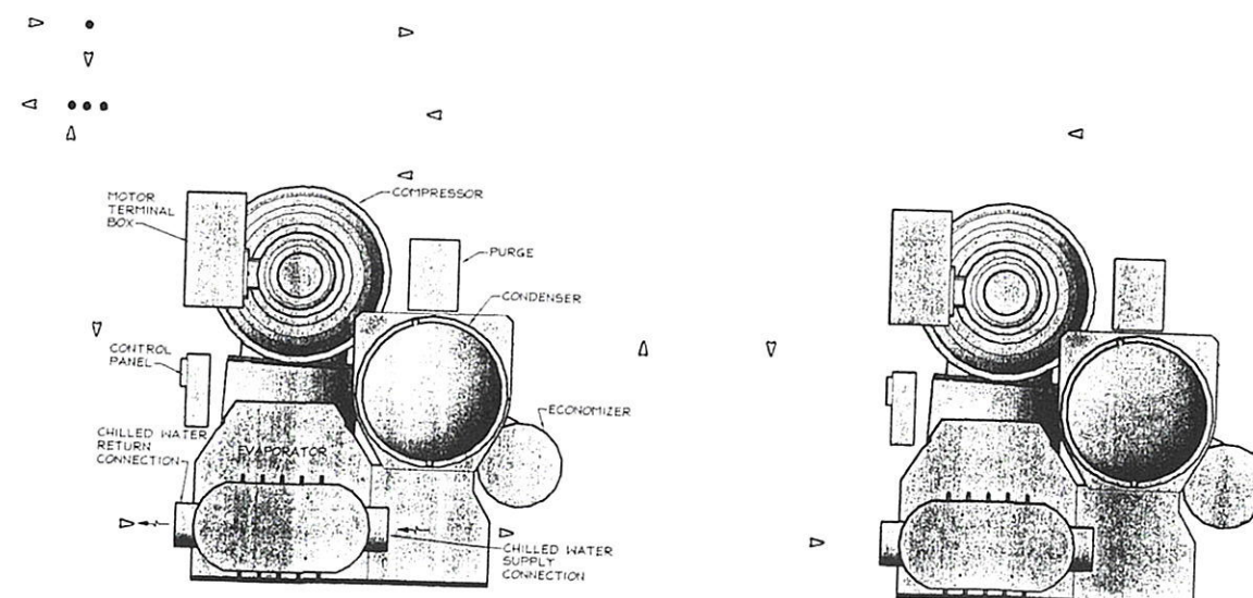
4 CHILLER END DETAIL H-500 DETAIL NOT TO SCALE
