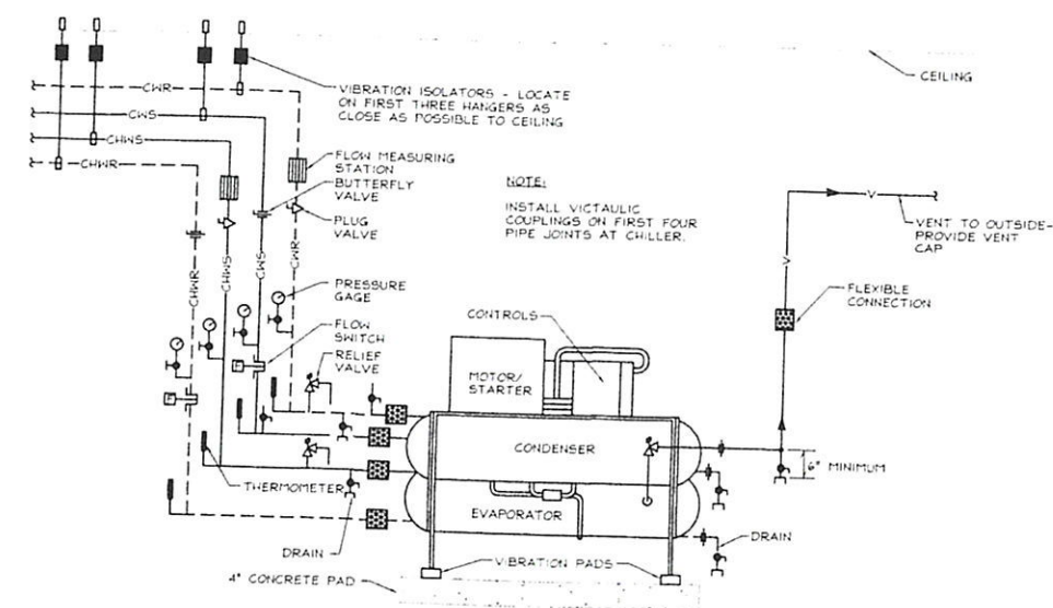
2 ELECTRIC CHILLER PIPING DIAGRAM H-500 DETAIL NOT TO SCALE
