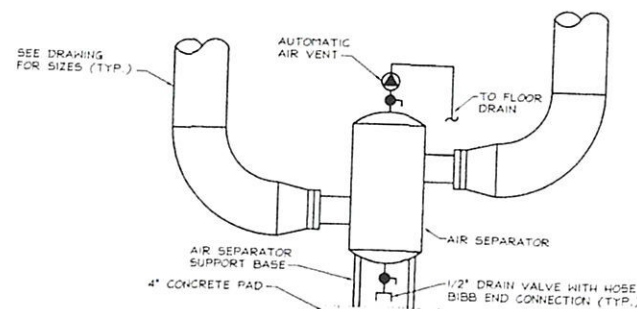
3 AIR SEPARATOR H-500 DETAIL NOT TO SCALE
