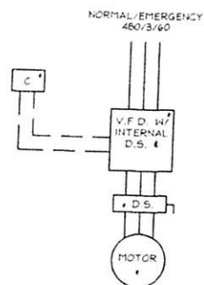
CHILLED WATER PUMP CHWP-2 125 HP (FREE STANDING)
