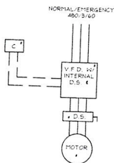
CHILLED WATER PUMP CHWP-1 125 HP (FREE STANDING)
