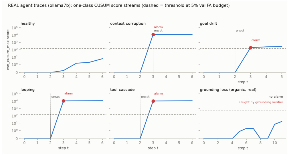
Figure 1: Real agent traces (ollama7b: qwen2.5:7b against real tools). One-class CUSUM score streams per failure class; dashed = threshold at the 5% validation FA budget, dotted = verified injection onset. The healthy run stays two orders of magnitude below the line, and every injected class — context corruption, goal drift , looping and tool cascade — alarms one step after onset. The sixth panel is grounding loss , and it is different in kind: fabrication cannot be injected into a live run, so this episode is a genuine one from the organic (non-injected) corpus, scored against that corpus’s own healthy null. The CUSUM stays flat – a fabricated figure perturbs no behavioural channel – and the class is caught instead by the deterministic grounding verifier. That is the blind spot the verifier exists to cover, shown rather than asserted. Note the y axis is symlog: real streams span twelve orders of magnitude, because the CUSUM accumulates multiplicatively once a failure takes hold.
