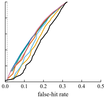
News (MRPC)
