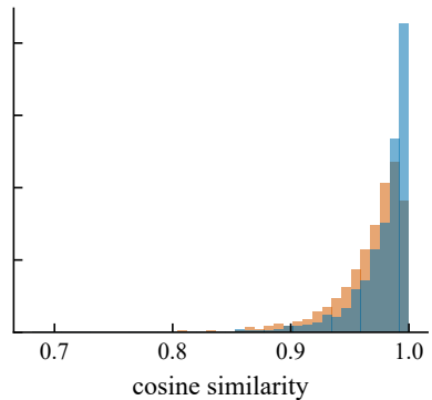
Adversarial (PAWS)
