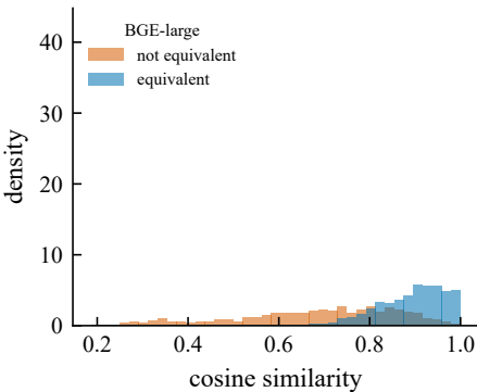
Questions (QQP)
