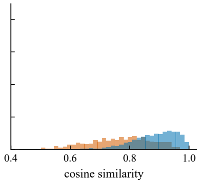
News (MRPC)
