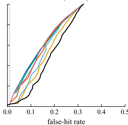
News (MRPC)
