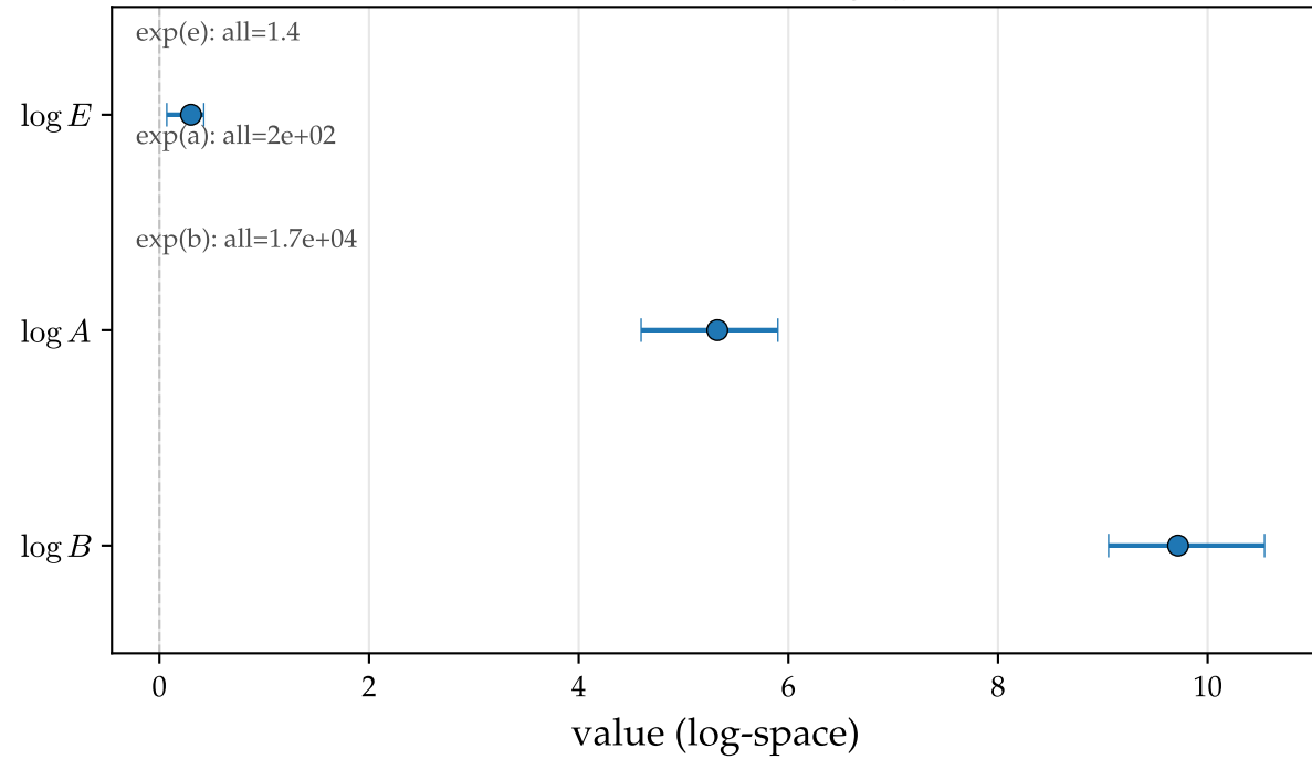
Chinchilla constants (log-space)
