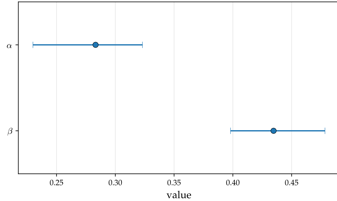
Chinchilla exponents
