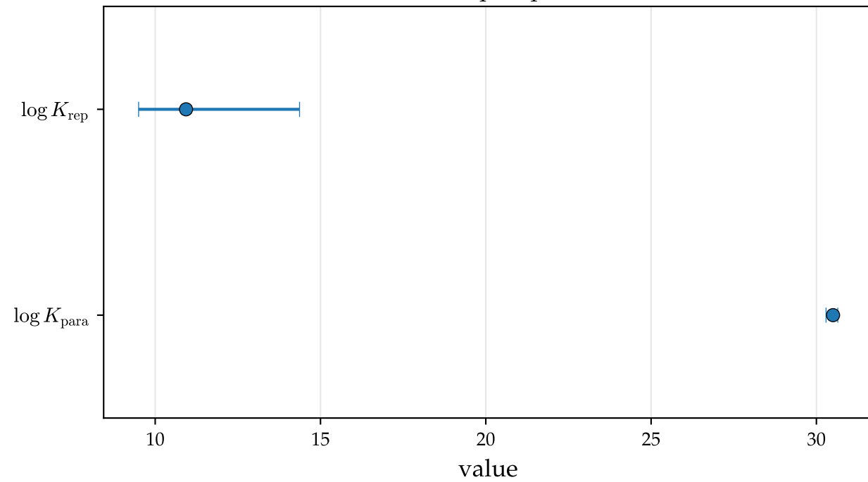
\log K (rep vs para)
