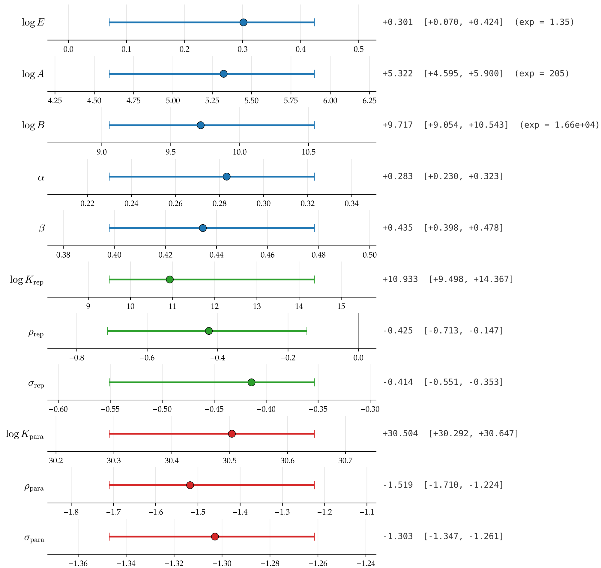
One-go triple fit — 95% bootstrap CIs (all, B = 200 , n_{\text{kept}} = 341 / 356 )
