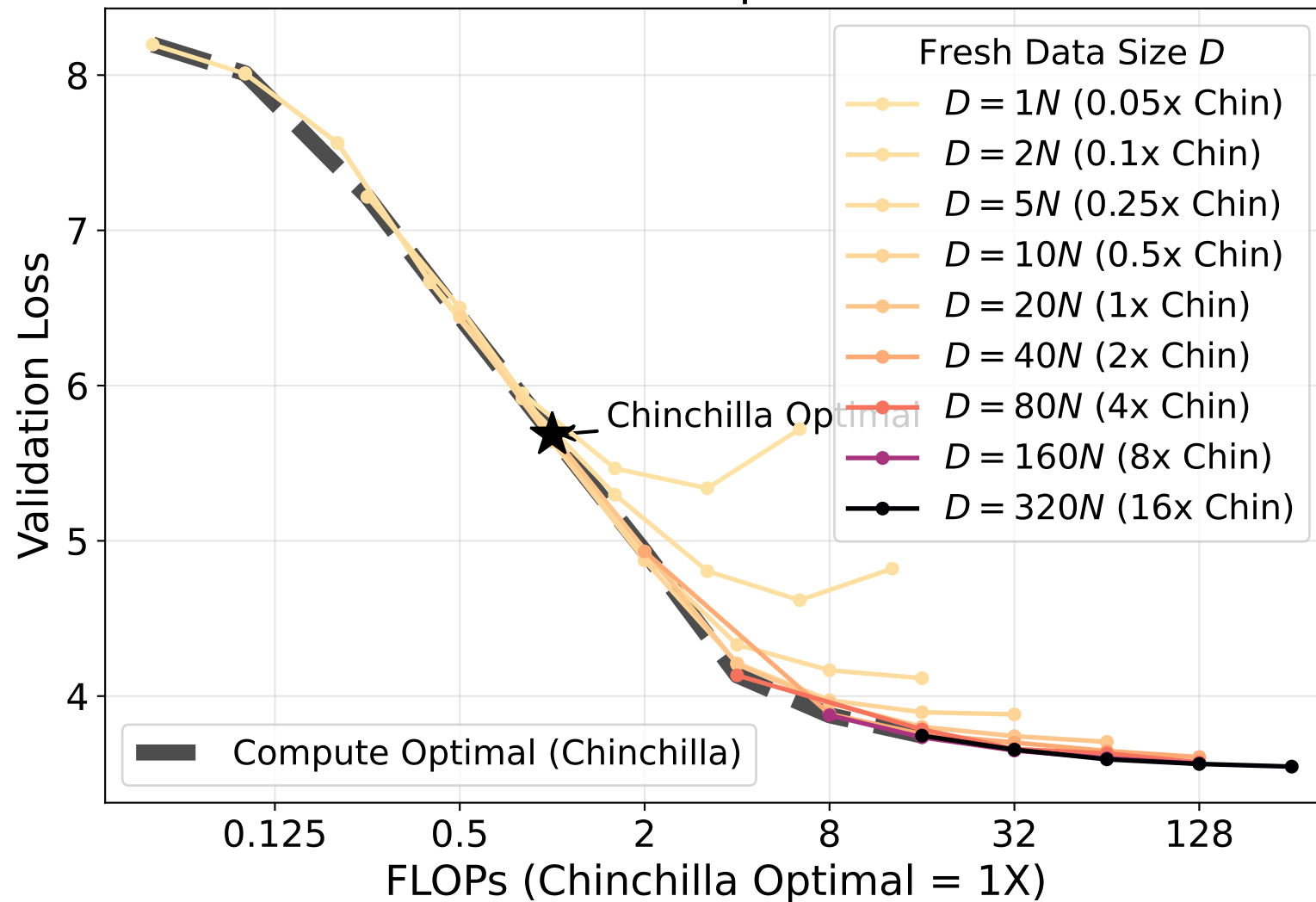
Multi-epoch
