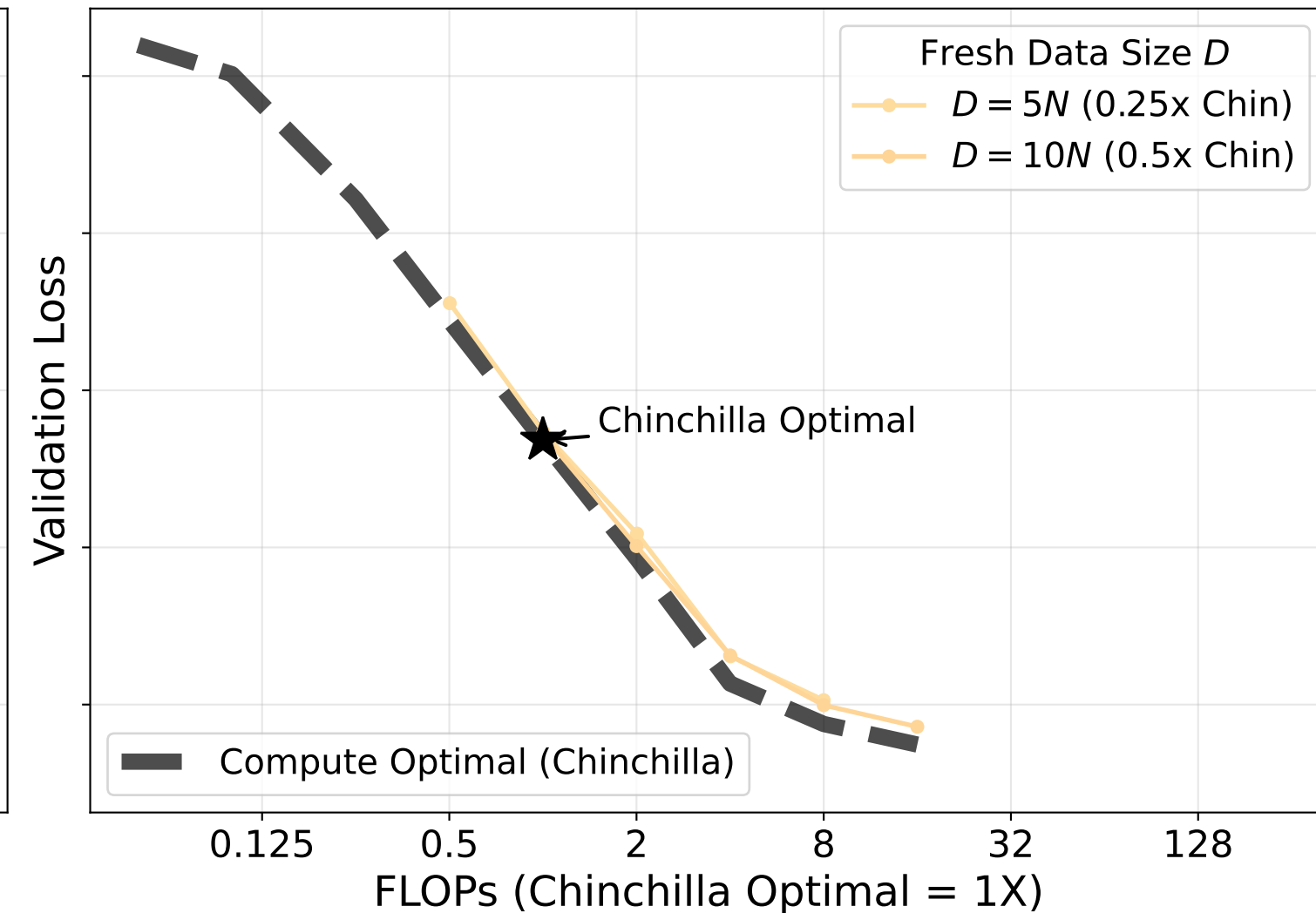
Self-distillation
