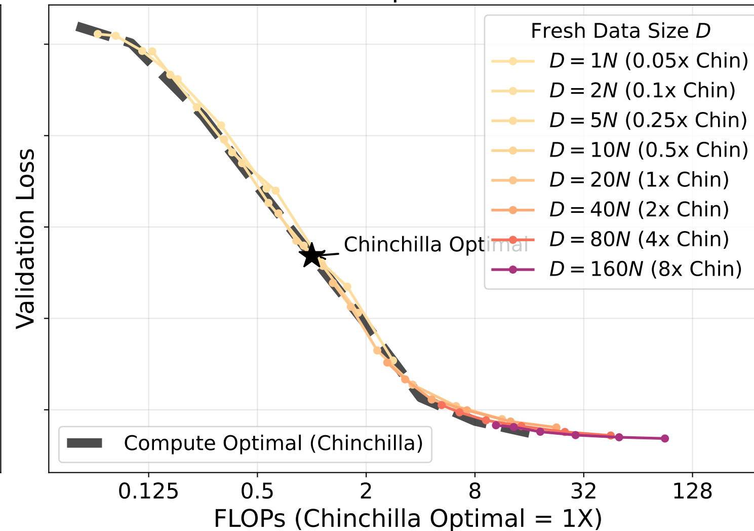
Paraphrase
