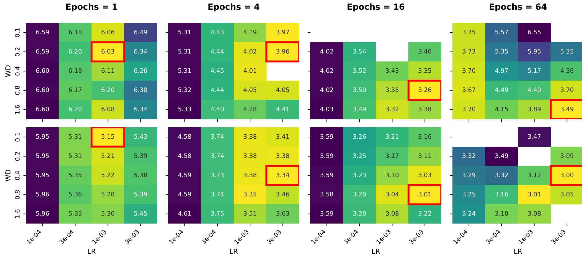
370M — Validation loss across (WD, LR) per (TTP, Epochs). Red box marks the optimum per cell.
