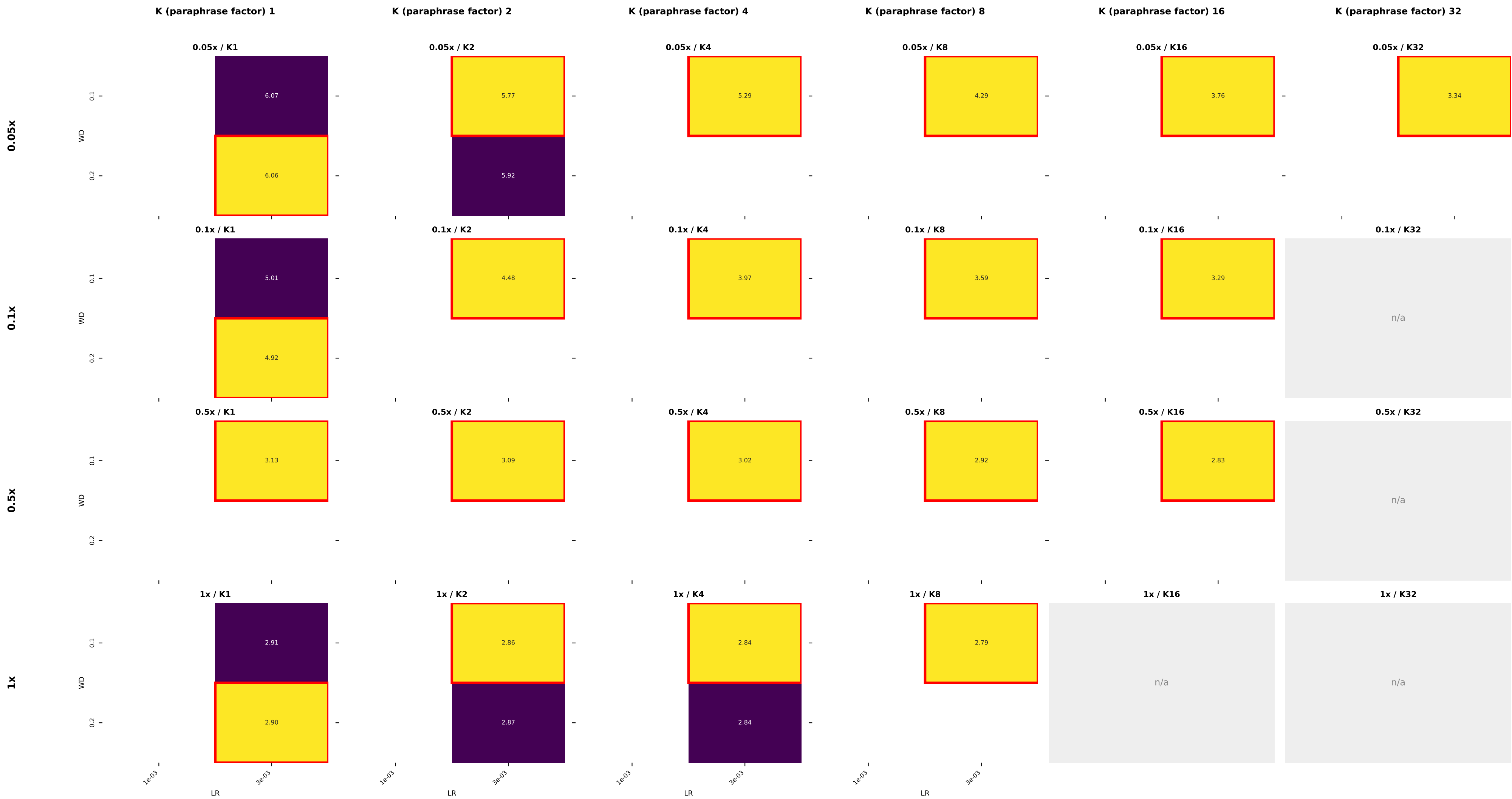
370M — Validation Loss (WD vs LR) Rows: Chinchilla multiplier (fresh data size) | Columns: K (paraphrase factor) Red box = best hyperparams per setting | Gray = n/a
