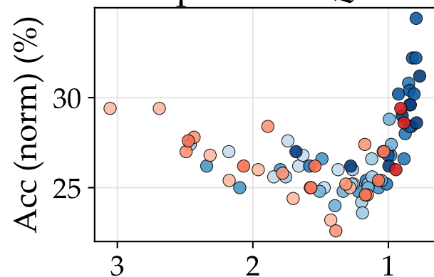
OpenBookQA
