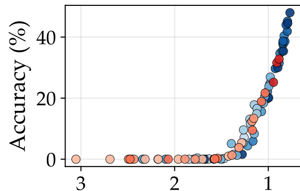
LAMBADA
