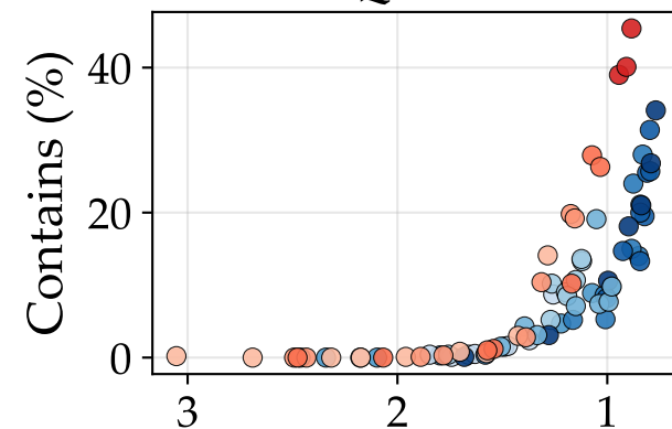
SQuAD
