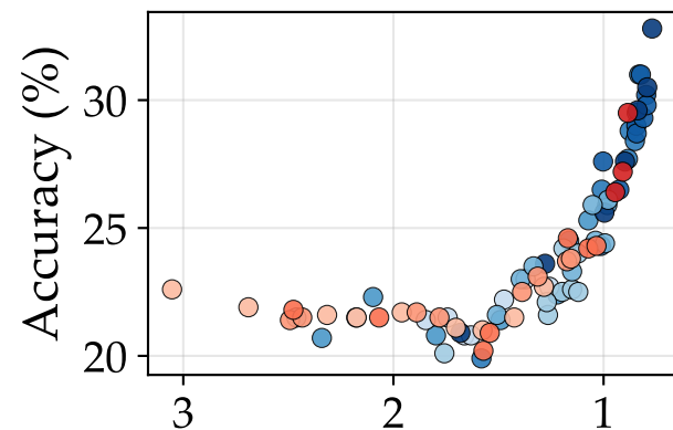
RACE
