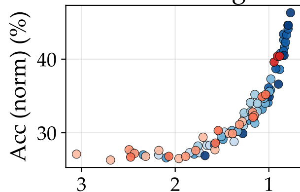
HellaSwag
