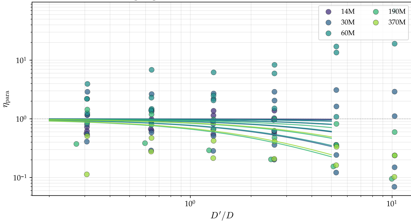
Joint Form B on paraphrase: \log K = 28.1 , \rho = -1.30 , \sigma = -1.22 (LOO=0.027)
