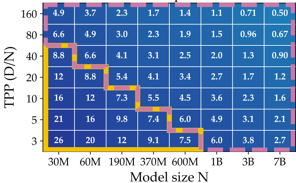
R^* — Repetition
