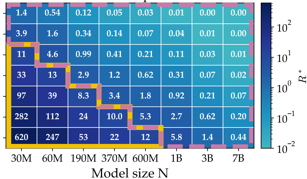
R^* — Paraphrase
