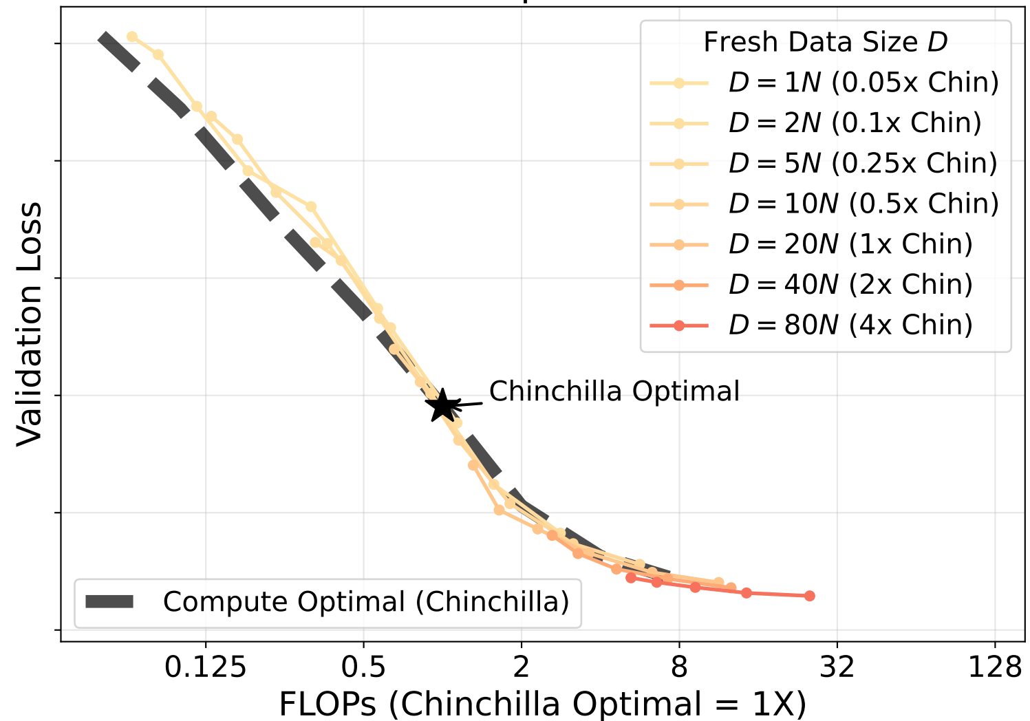
Paraphrase
