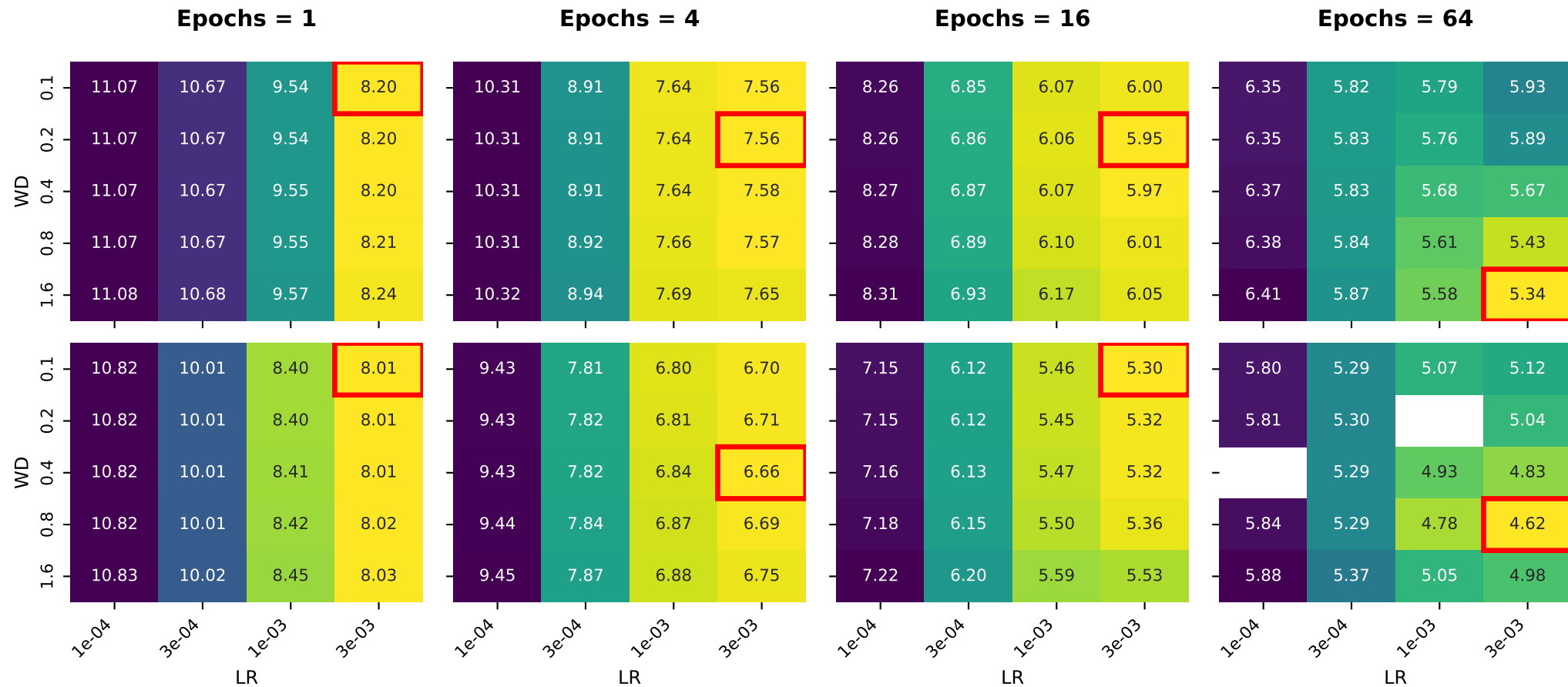
30M — Validation loss across (WD, LR) per (TTP, Epochs). Red box marks the optimum per cell.
