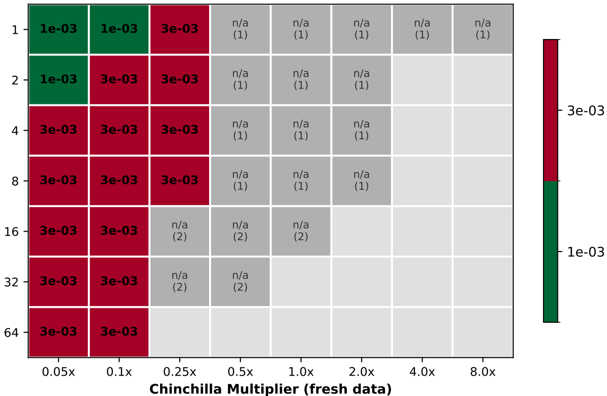
Optimal LR
