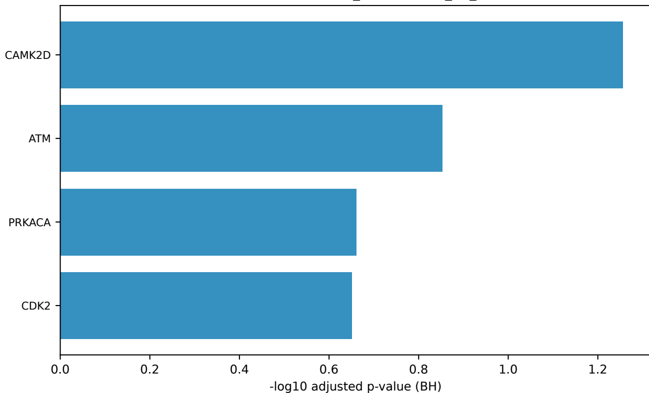
Kinase enrichment (KEA_2015) — hits_UP_90min
