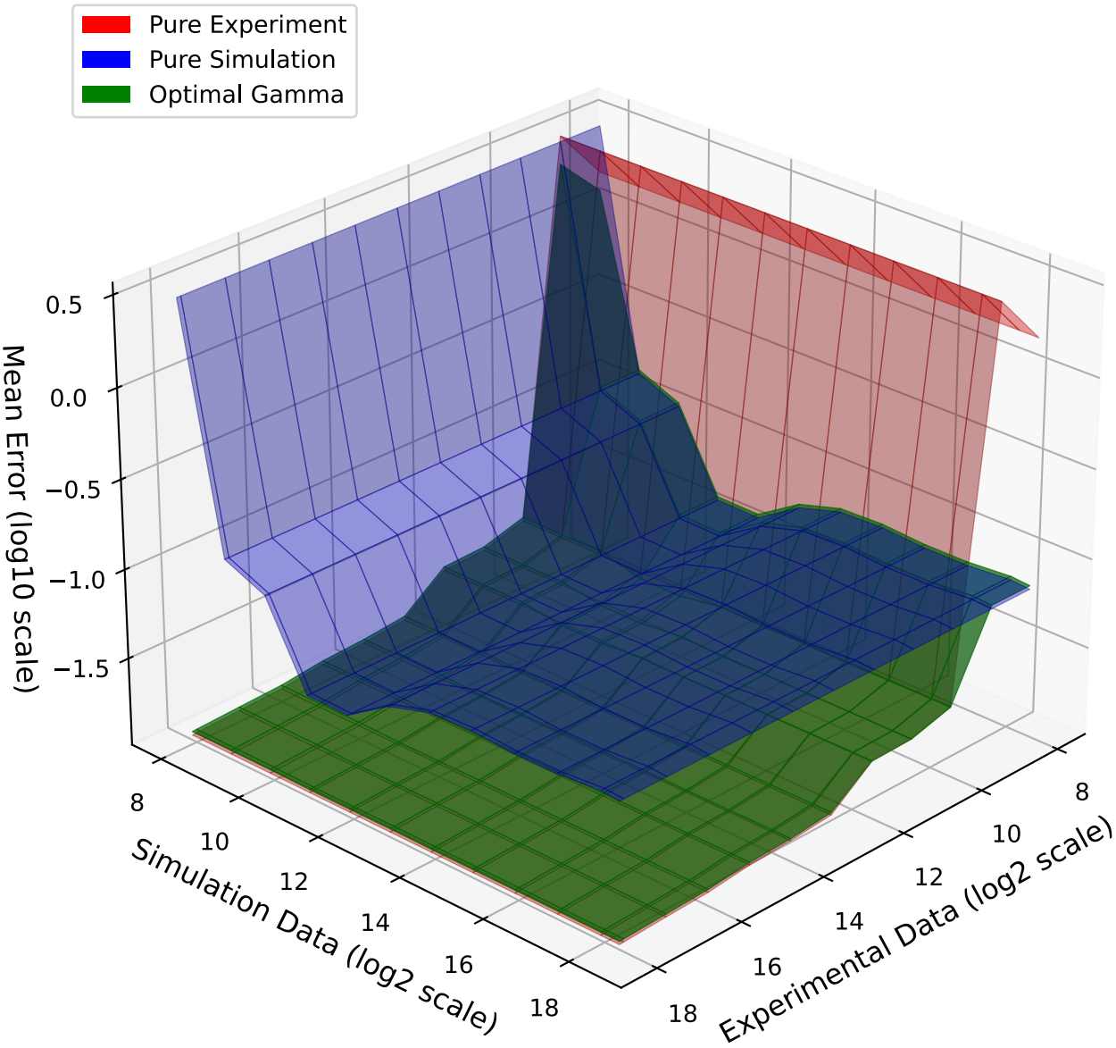
Optimal Gamma Error Surface vs Pure Models
