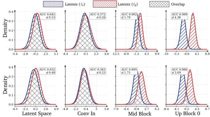
Figure 3: LDA projections of z_e and z_g for iMF-B/2 (top) and iMF-XL/2 (bottom). The vertical axis shows the Gaussian-smoothed, normalized histogram density of the one-dimensional LDA scores.
