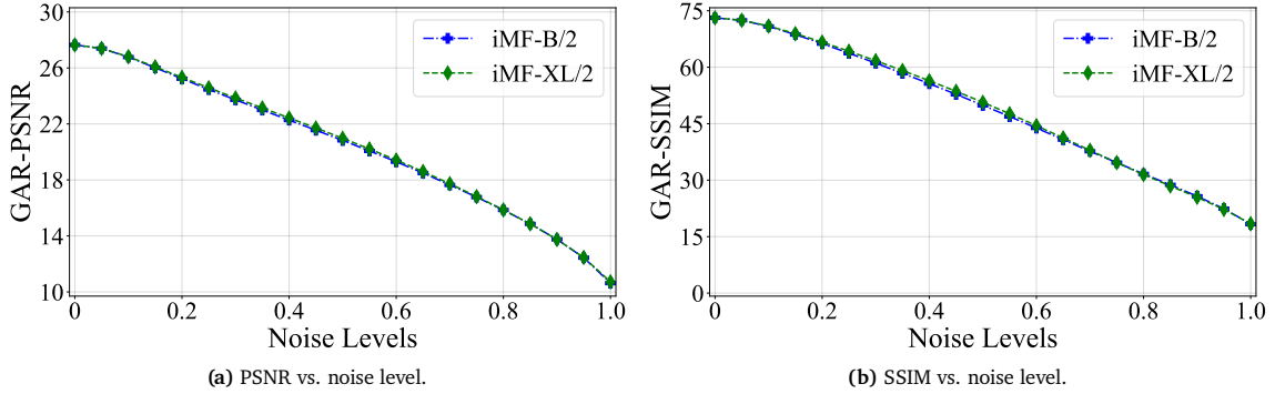
Figure 10: Structural quality under GAR across noise levels. PSNR (left) and SSIM (right) degrade consistently as noise increases. Increasing generative model capacity (iMF-B/2 vs. iMF-XL/2) does not improve structural quality, as both follow nearly identical trends.
