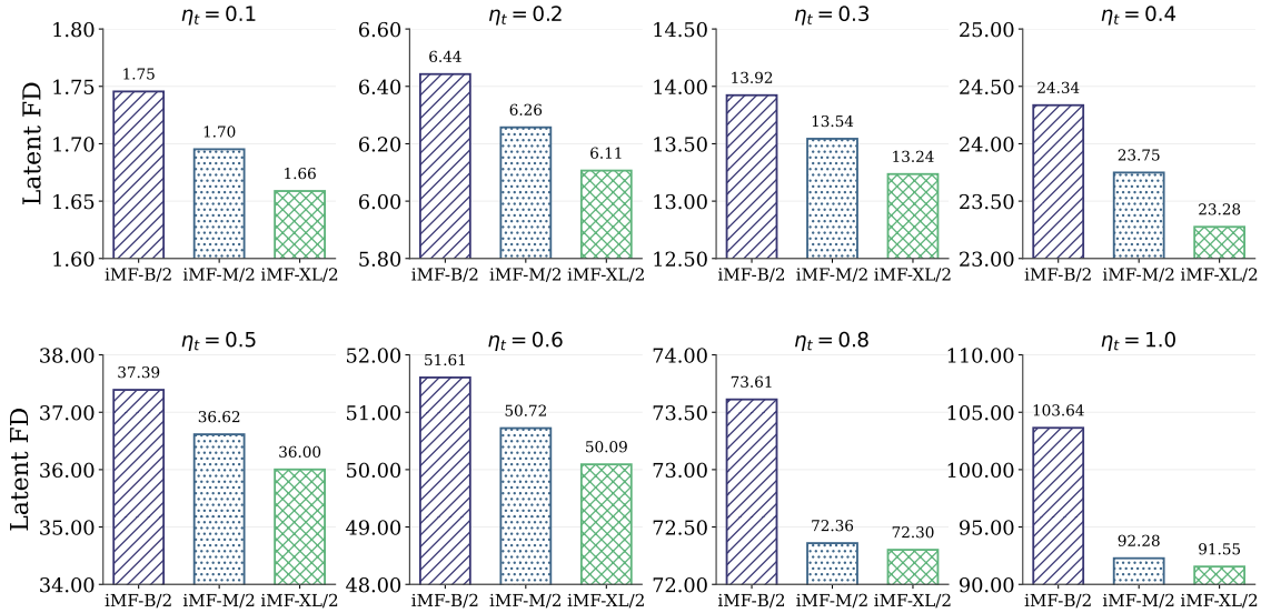
Figure 12: Latent-FD( \mathcal{P}_g^t, \mathcal{P}_e ) across noise levels for different generative models, with \eta_t = 1.0 corresponding to Latent-FD( \mathcal{P}_g, \mathcal{P}_e ). The model ordering is preserved across noise levels.
