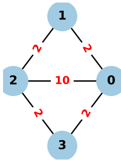
Diagonal Square ( N=4 , E=5 )
