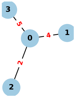
Heavy Star S_4 ( N=4 , E=3 )
