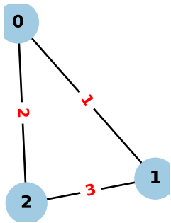
Weighted Triangle ( N=3 , E=3 )
