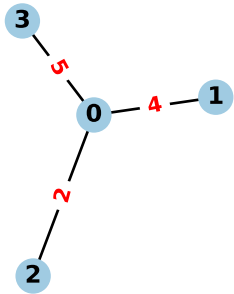
Heavy Star S_4 ( N=4 , E=3 )
