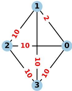
Frustrated K_4 ( N=4 , E=6 )
