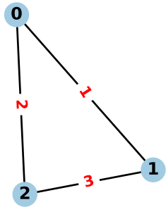
Weighted Triangle ( N=3 , E=3 )
