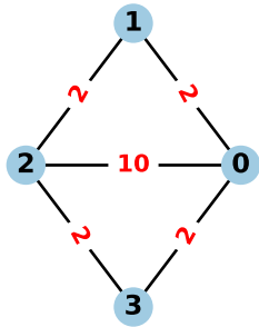
Diagonal Square ( N=4 , E=5 )
