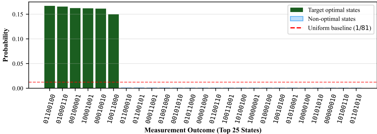
Grover Measurement Distribution: Frustrated K_4 ( K=3 , 2 iterations)
