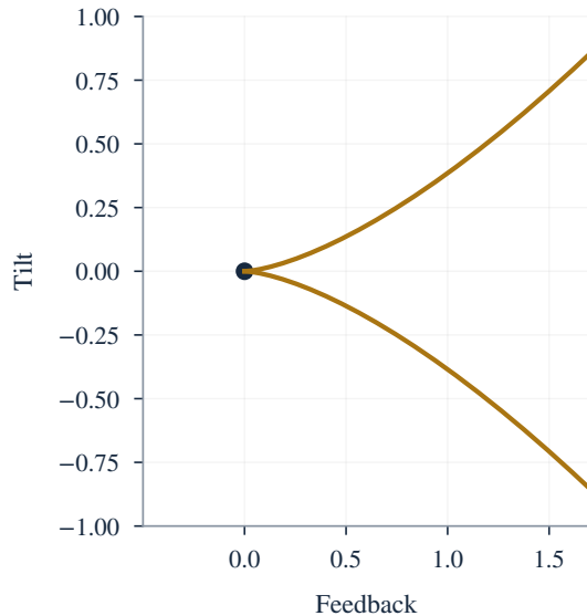
B Two folds meet at a cusp
