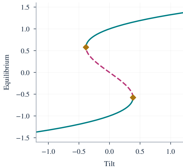
A Equilibrium section: feedback = 1
