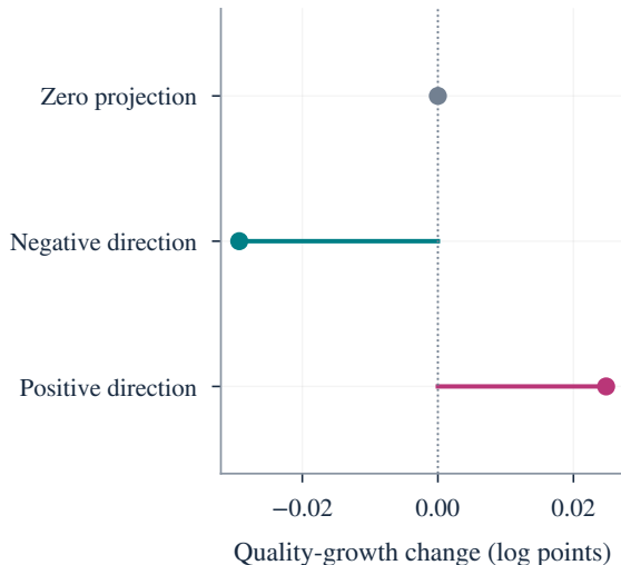
B Different quality consequences
