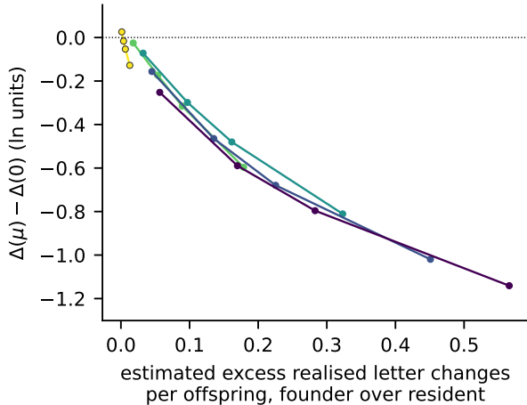
b against estimated excess letter changes
