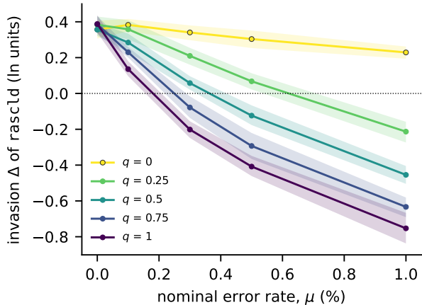
a invasion by redraw probability
