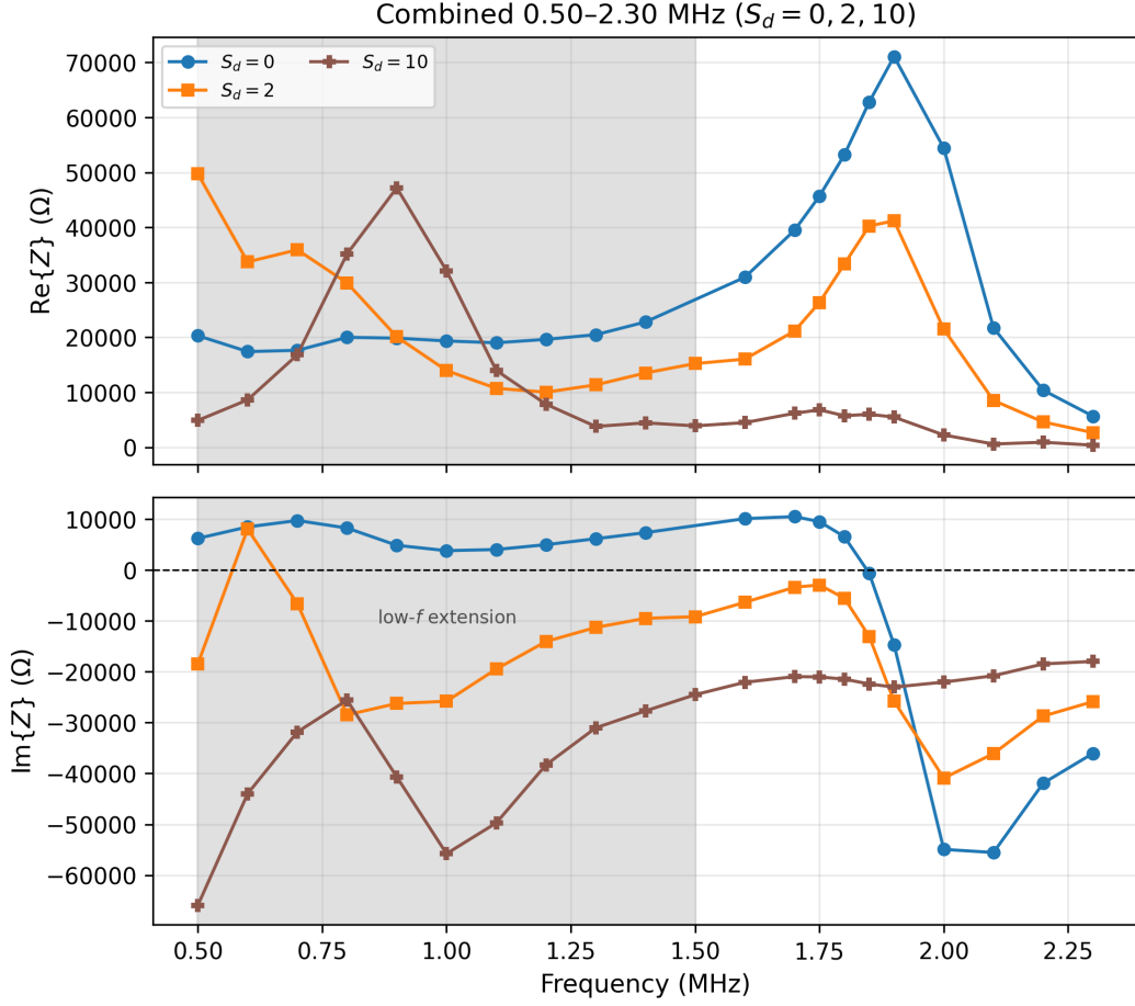
Figure 6. Combined CW impedance for S_d = 0, 2, 10 over 0.50–2.30 MHz. The shaded region is the low-frequency extension. Shared tones at f \geq 1.50 MHz match the dense band exactly; S_d = 0 omits the incomplete 1.50 MHz restart (visible 1.40–1.60 MHz gap).
