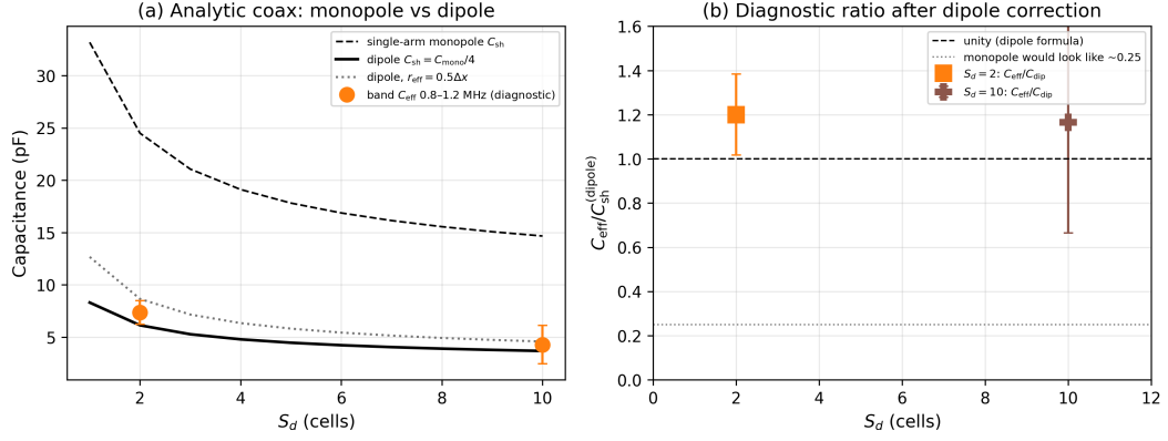
Figure 9. (a) Monopole coax (dashed), dipole coax (solid), and staircased-radius dipole sensitivity (dotted), with diagnostic low-frequency C_{eff} means. (b) Ratio to the dipole formula is order unity ( \approx 1.2 ).
