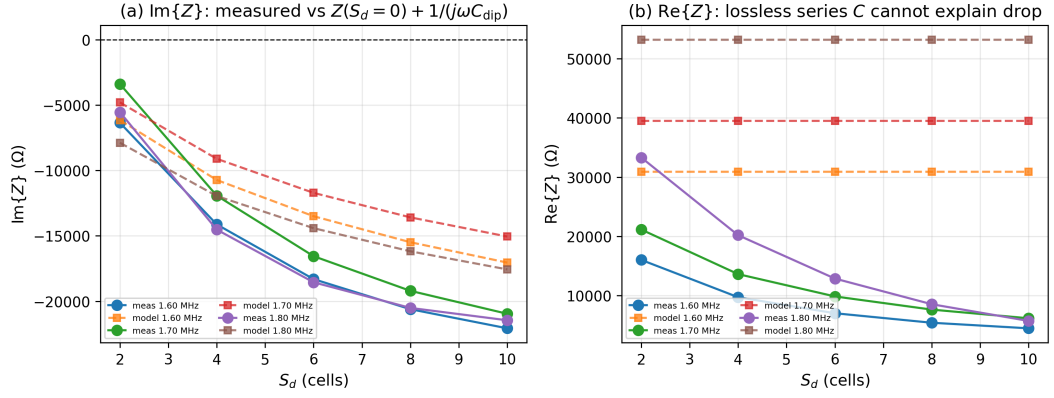
Figure 10. Circuit overlay at dense-band frequencies: measured Z(S_d) versus Z(S_d=0) + 1/(j\omega C_{sh}^{(dip)}) . (a) Imaginary part. (b) Real part. Lossless series C cannot explain the measured resistive drop.
