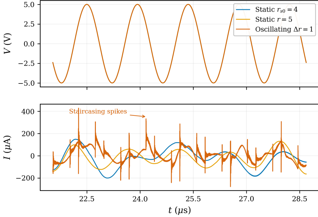
Figure 2. Hard pilot late-time feed traces (last \sim 5 drive cycles). Voltage traces coincide; oscillating current shows impulsive spikes synchronized with integer radius updates.
