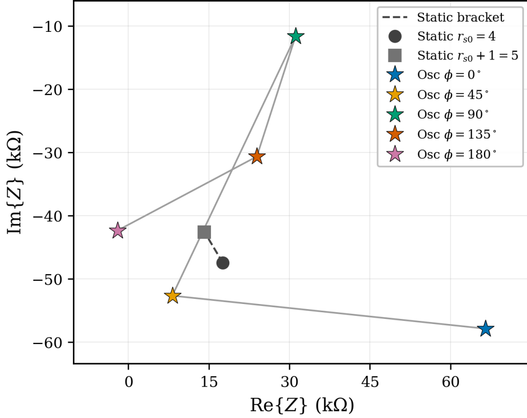
Figure 7. Soft phase scan at 700 kHz, \Delta r = 1 . Gray markers and dashed segment: static bracket. Colored stars: oscillating cases at \phi = 0^\circ – 180^\circ , connected in phase order. All oscillating points remain outside the bracket while \arg(Z) rotates.
