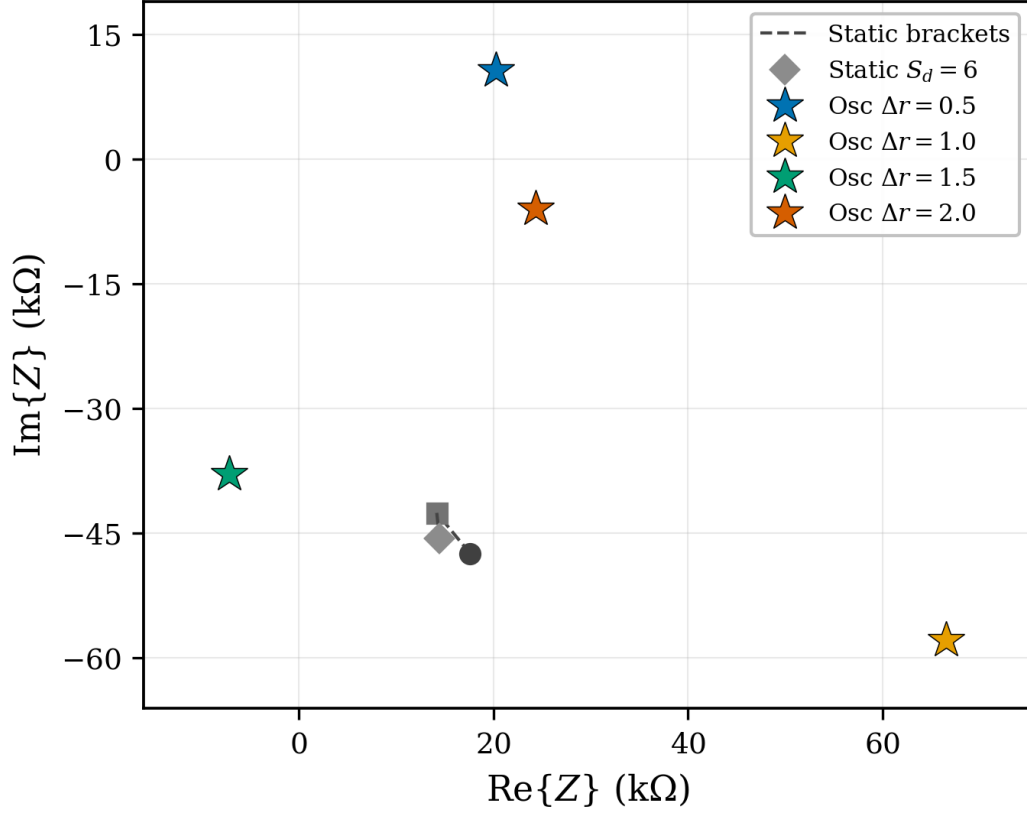
Figure 8. Matched soft \Delta r scan (soft = \Delta r ) at 700 kHz. Dashed segments: static brackets through S_d = 6 . Stars: oscillating amplitudes 0.5–2. All remain out-of-bracket without a monotonic amplitude progression.
