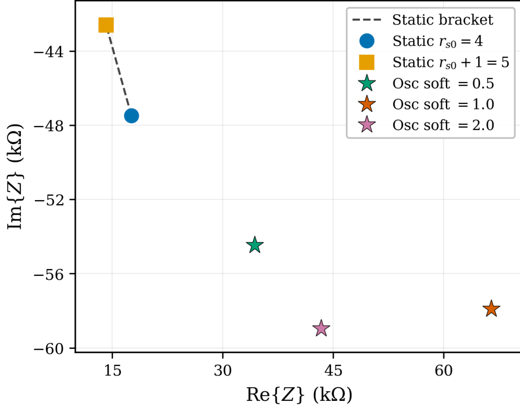
Figure 5. Soft-edge width sensitivity at fixed \Delta r = 1 , 700 kHz: oscillating Z for blend widths 0.5, 1, and 2 cells remains outside the static bracket.
