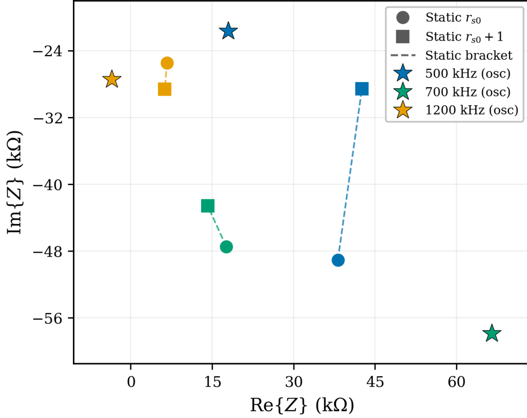
Figure 6. Sparse-frequency soft \Delta r = 1 results in the complex plane. Circles/squares and dashed segments are static brackets at each tone; stars are oscillating cases. Color encodes frequency (0.5, 0.7, 1.2 MHz).
