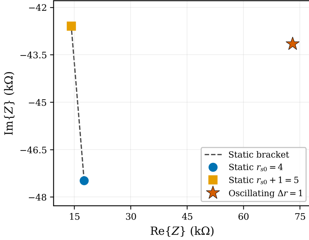
Figure 1. Hard pilot complex-plane phasor Z at 700 kHz: static jackets at r_{s0} = 4 and r_{s0} + 1 = 5 define the dashed bracket; the oscillating \Delta r = 1 case lies far outside that segment.
