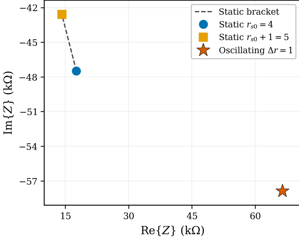
Figure 3. Soft-edge pilot: same static bracket as Figure 1; oscillating \Delta r = 1 with one-cell soft blend remains far outside the bracket.
