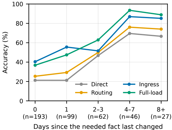
Qwen3.5-27B
