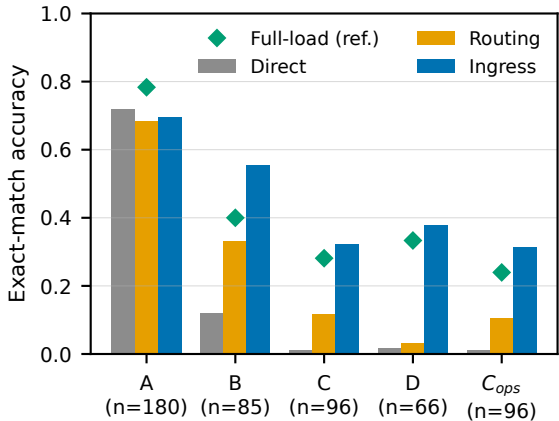
Qwen3.5-27B
