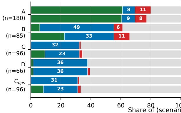
Qwen3.5-27B
