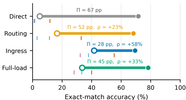
(b) Partial-state penalty \Pi = \text{Acc}_A - \text{Acc}_{\text{BuCuD}} and recovery \rho
