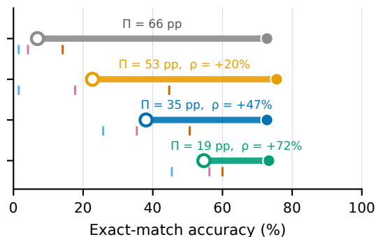
(b) Partial-state penalty \Pi = \text{Acc}_A - \text{Acc}_{\text{BuCuD}} and recovery \rho
