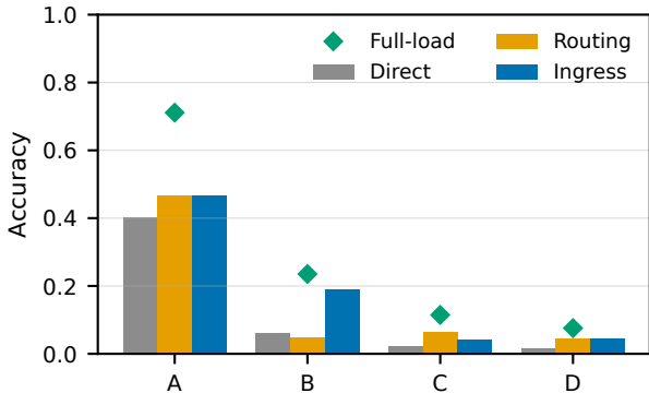
Qwen3.5-9B
